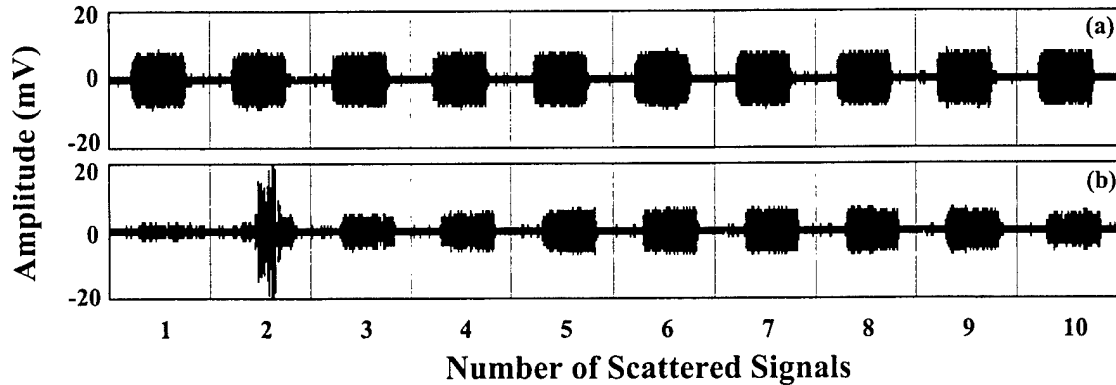
Figure 2. Sonazoid bubble (a) detected over 450 \mu s without excitation (and without bubble growth) and (b) demonstrating growth following a 2.5 MHz, 16 cycle 1.8 MPa excitation pulse. The imaging pulse pressure was less than 0.1 MPa in both cases. Notice, the difference in the initial bubble size (sequence 1) in the two cases.
