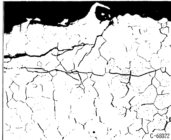
Figure 12. - Microstructure of polycrystalline tungsten showing brittle transgranular fracture. Test temperature, 600° F; carbon content, 45 ppm. X150.
