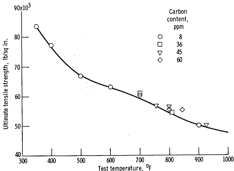
Figure 9. - Ultimate tensile strength of polycrystalline tungsten with varying carbon content.
