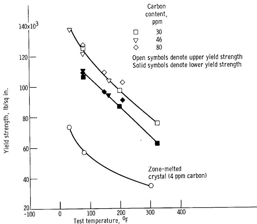
Figure 14. - Effect of carbon on yield strength of tungsten single crystals.
