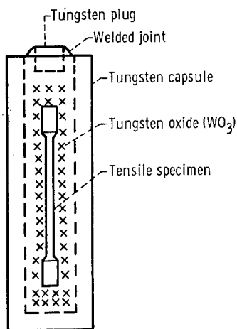
Figure 1. - Capsule employed to add controlled amounts of oxygen to tungsten.
