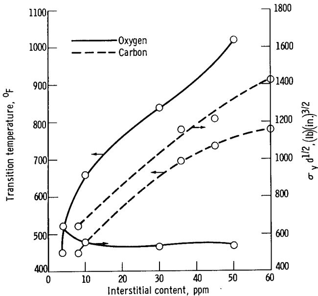
Figure 7. - Comparison of changes in transition temperature and \sigma_y d^{1/2} at 750° F as functions of interstitial impurity content.
