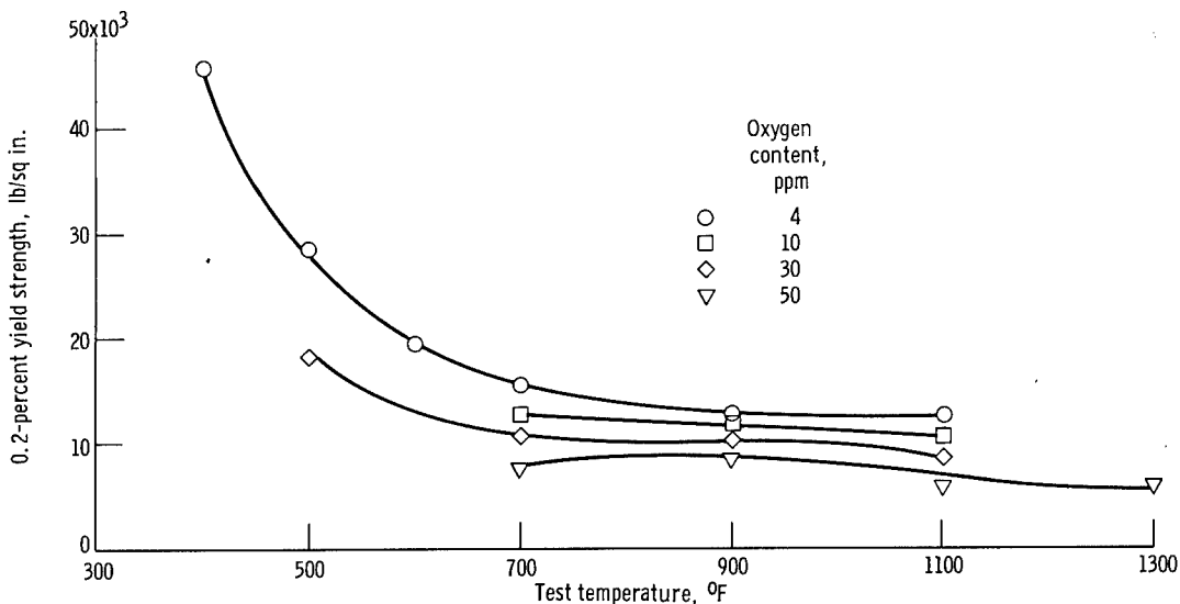
Figure 6. - Effect of oxygen on yield strength of polycrystalline tungsten.
