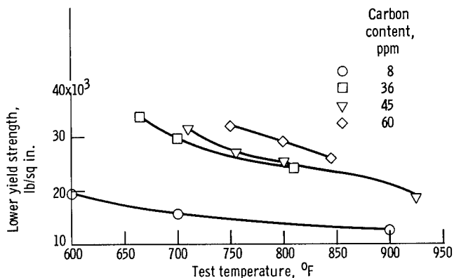
Figure 10. - Temperature dependence of yield strength in polycrystalline tungsten with varying carbon content.
