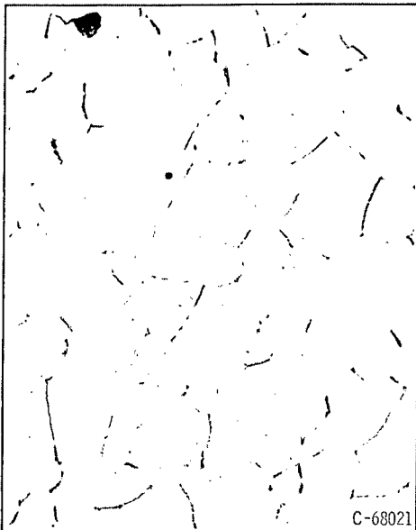
Figure 11. - Microstructure of polycrystalline tungsten. Carbon content, 45 ppm. X150.
