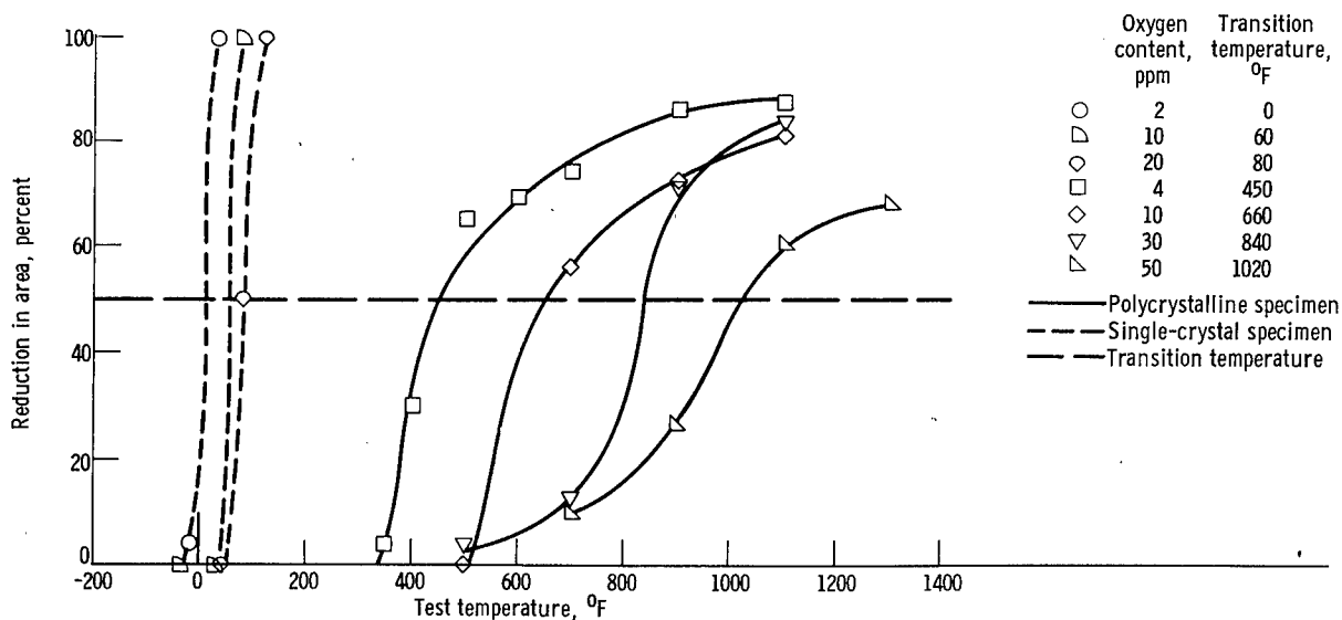
Figure 2. - Effect of oxygen on ductility of tungsten.
