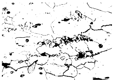
(c) Tungsten - 8 volume percent hafnium carbide.
