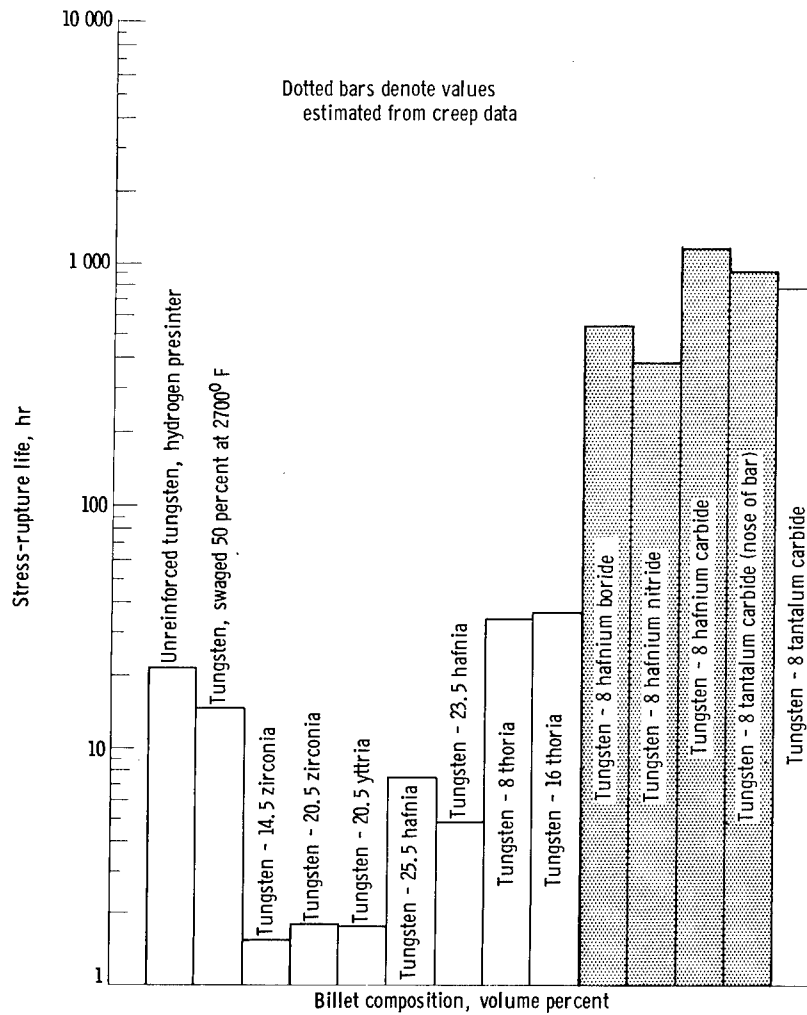
Figure 7. - Stress-rupture life of tungsten, tungsten-oxide, and tungsten - refractory-compound composites. Temperature, 3000° F; stress, 8000 pounds per square inch.
