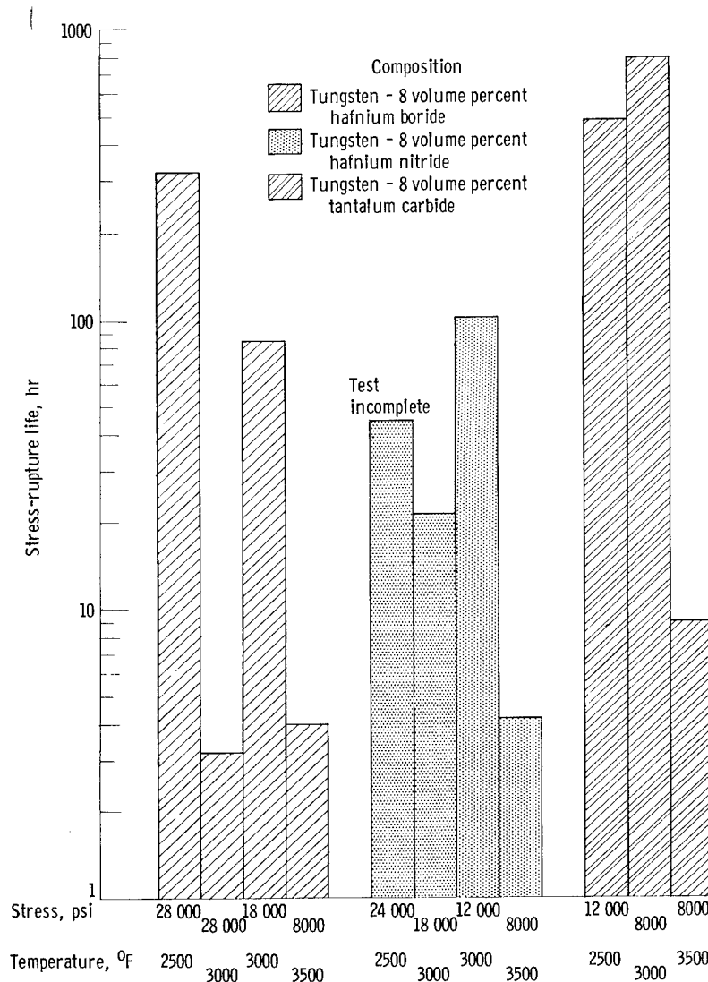
Figure 11. - Stress-rupture tests of tungsten - 8-percent-refractory-compound composites at temperatures of 2500°, 3000°, and 3500° F.
