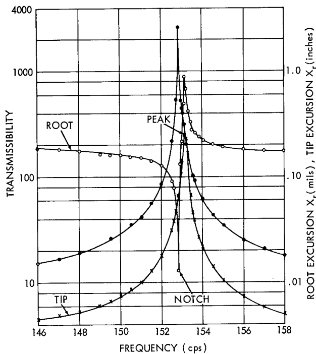
Figure 2—Transmissibility plot for a nominal 150 cps beam, 0.10 in. thick (specimen No. A-10).
