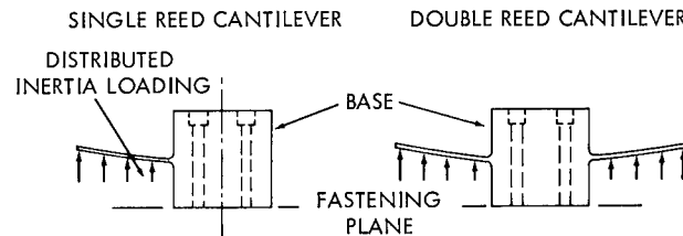
(b) Beam Under Inertia Loading During Vibration
