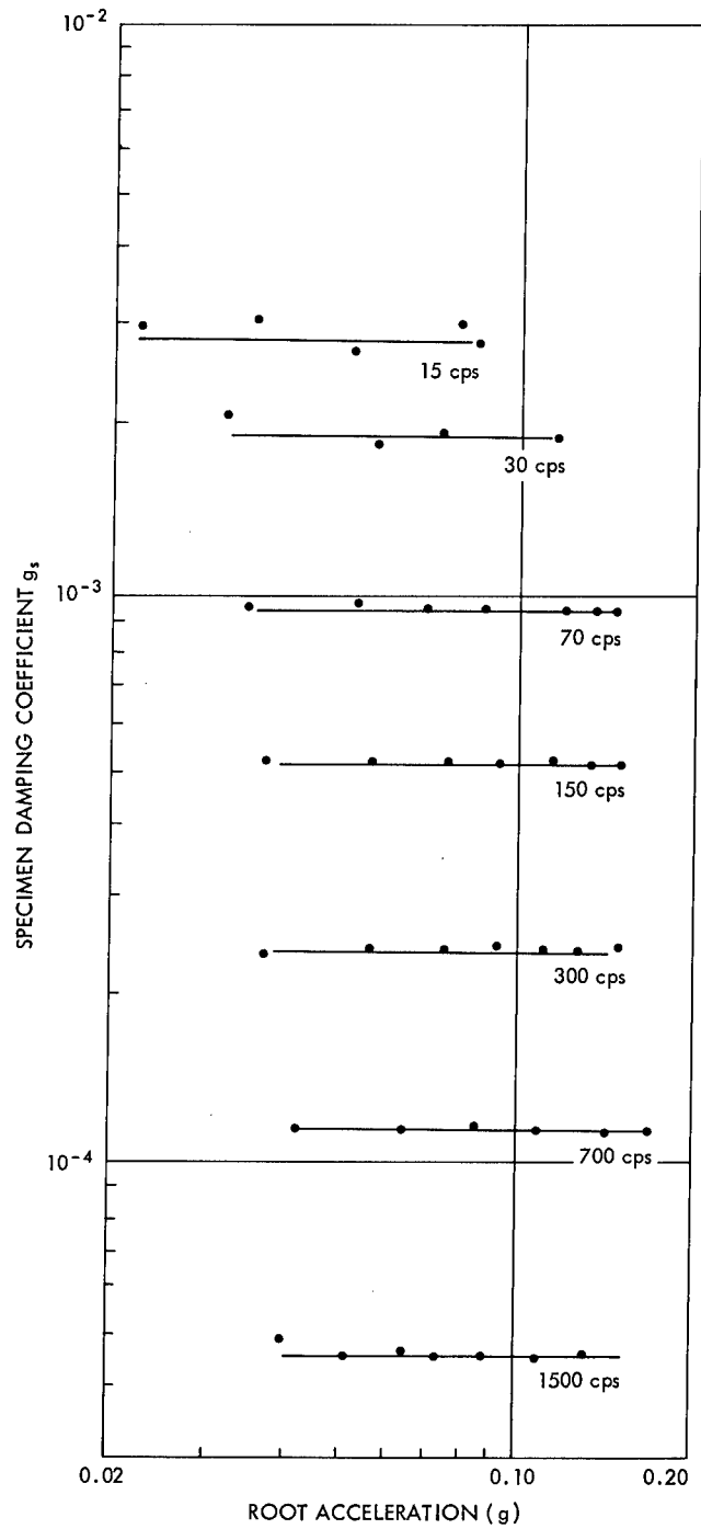
Figure 12—Results for seven resonant beams of 1/10-inch thick aluminum tested in a vacuum of 0.2 torr.
