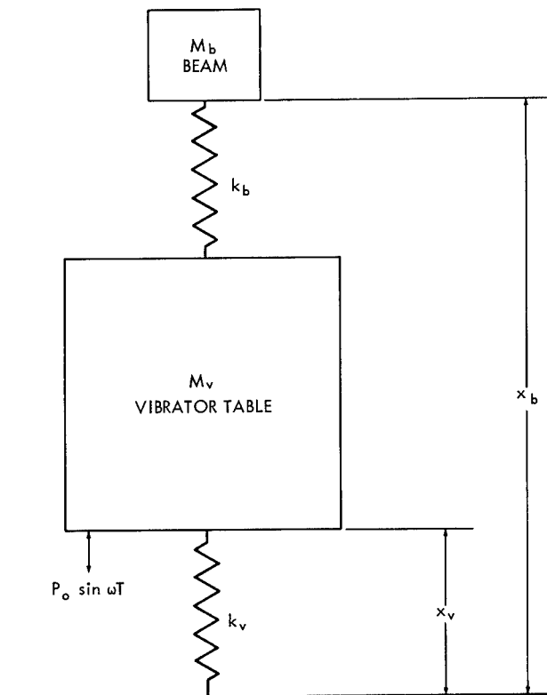
Figure 3—Model for the analysis of a beam-vibrator combination as a two-degree-of-freedom system.
