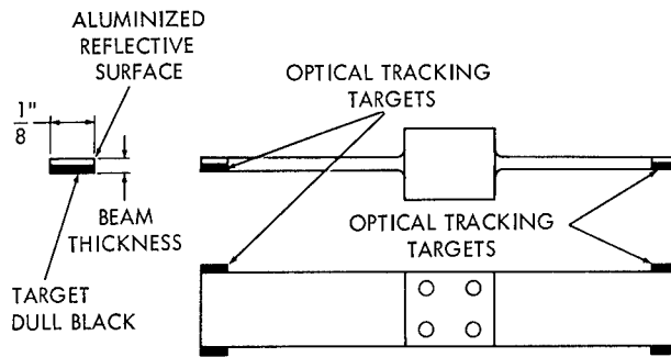
Figure 7—Location of optical tracking targets.
