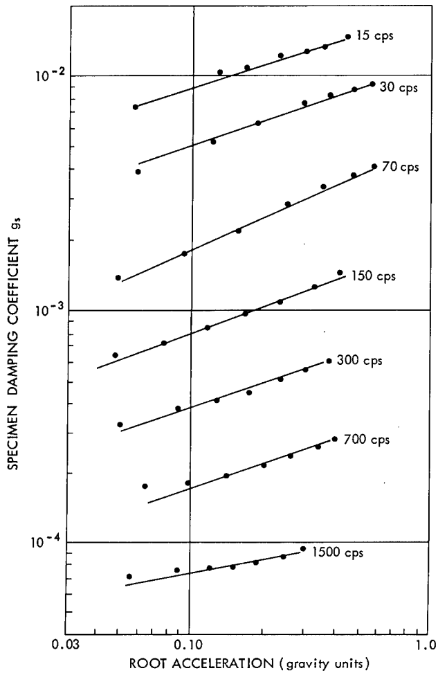
Figure 11—Results for damping in air for seven 1/10-inch thick aluminum cantilever beams (resonant frequencies shown).
