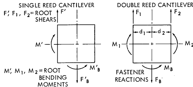
(c) Free Body Diagram of Beam Base Under Inertia Loading
