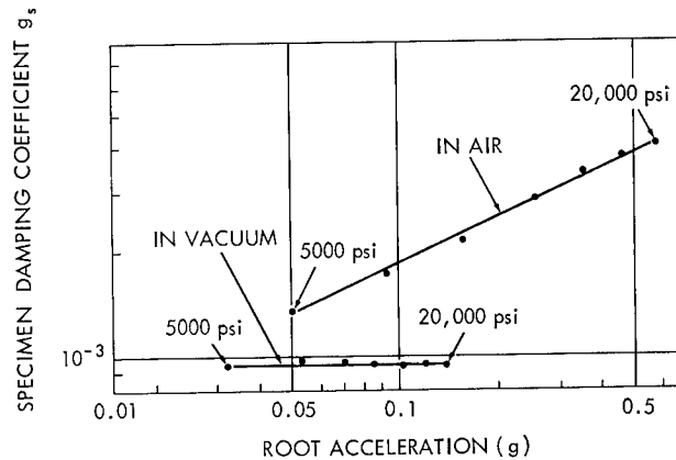
Figure 10—Comparison of damping in vacuum with damping in air for a nominal 70 cps beam stressed between 5000 and 20,000 psi at beam root.
