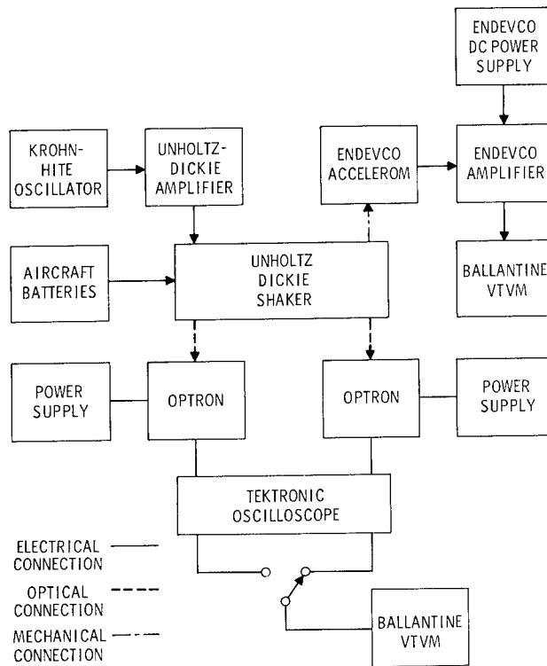
Figure 4—Instrumentation block diagram.
