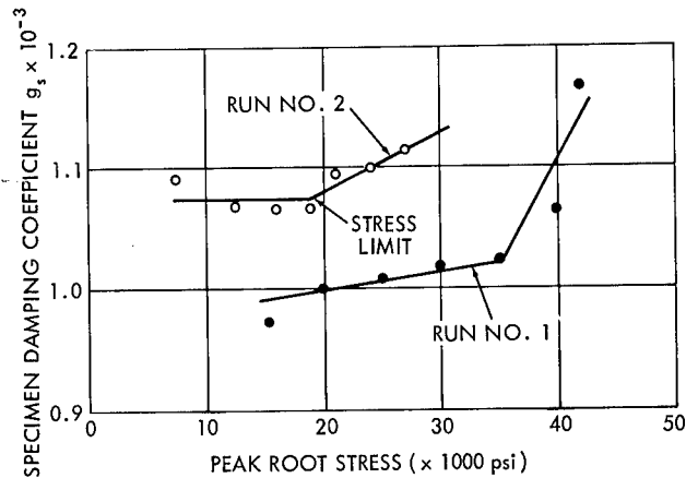
Figure 9—Graph showing the location of stress limit and the effect of near yield stresses on the damping coefficient.
