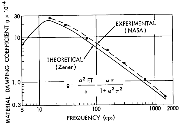
Figure 14—Comparison of damping as calculated by theoretical thermal relaxation equations and as measured experimentally (for 0.10-inch thick aluminum beams).
