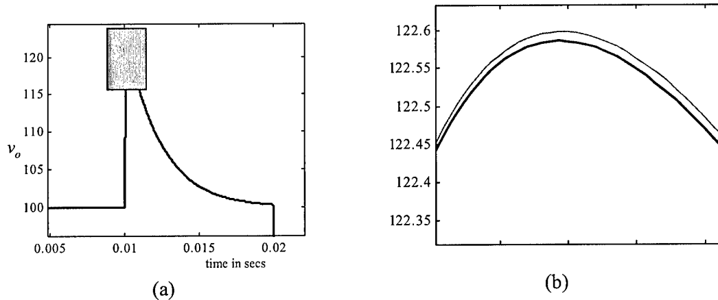
(a) (b) Figure 18. (a) Converter output voltage in sample system with individually optimized converter design (-) and converter design obtained from optimized sample system (--) (b) Expanded view of shaded area in (a)
