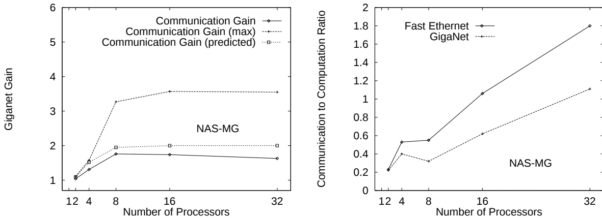
FIG. 6.5. Computation and communications gains achieved by GigaNet (left-hand chart) and communication to computation ratio for the Fast Ethernet and the GigaNet networks (right-hand chart). These experimental results have been obtained for the NAS-MG (Class B) benchmark using a dual node configuration.
