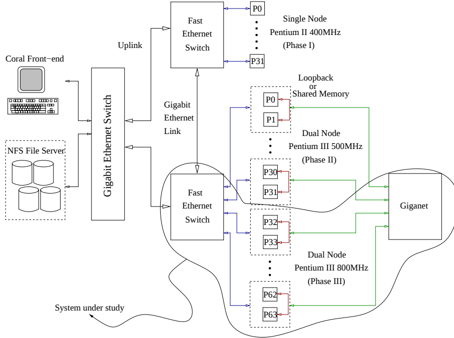
FIG. 2.1. Coral PC-Cluster at ICASE (Nasa Langley Research Center)
