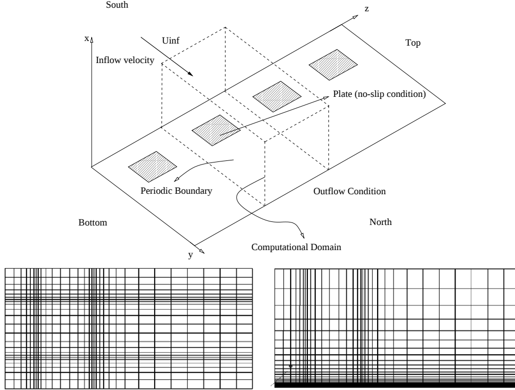
FIG. 4.2. Schematic configuration of the numerical simulation (top chart). Computational grid used, yz -plane (Bottom-left chart) and xy -plane (Bottom-right chart).
