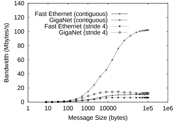
FIG. 6.1. Point-to-point communication bandwidth obtained by MPI/Pro over GigaNet and over Fast-Ethernet in Coral. The measurements have been obtained using the classical ping-pong test with two different message memory layouts: contiguous and stride-four vectors.
