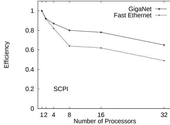
FIG. 6.2. Parallel efficiency obtained by the SCPI solver for a fixed problem size using a dual node configuration in combination with the GigaNet or the Fast-Ethernet networks.
