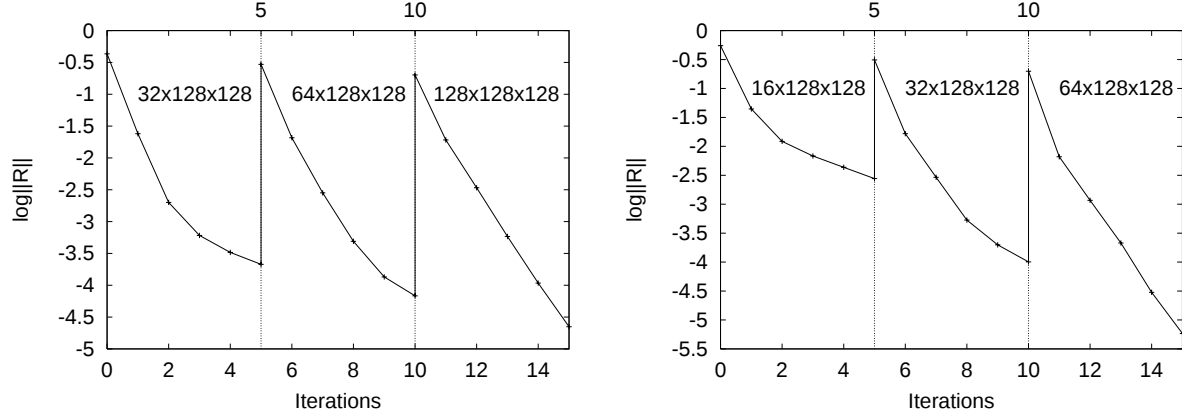
FIG. 7.1. L_2 -norm of the residual versus F(2,1) -cycles of the investigated SCPI algorithm for the flat plate simulation with Re = 10^4 on a 128 \times 128 \times 128 grid (left-hand chart), and a 64 \times 128 \times 128 (right-hand chart).
