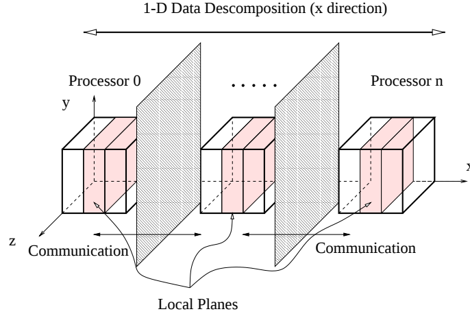
FIG. 5.1. Schematic data distribution of a 1-D data decomposition
