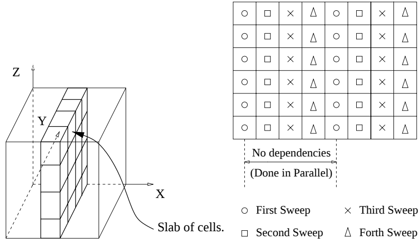
FIG. 4.1. Slab of cells updated simultaneously when using the yz-plane implicit smoother (left-hand chart). Four-color ordering of planes and data dependencies (right-hand chart).
