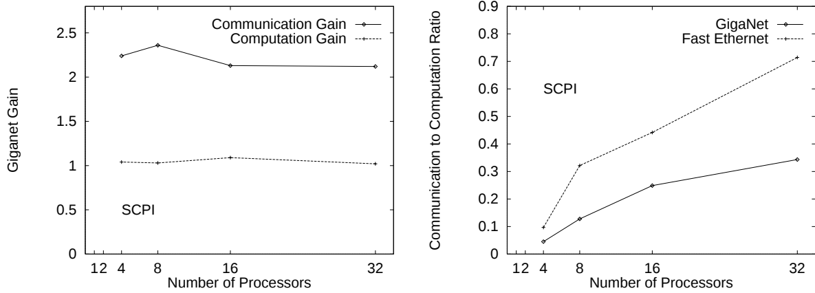
FIG. 6.3. Computation and communications gains achieved by GigaNet (left-hand chart) and communication to computation ratio for the Fast Ethernet and the GigaNet networks (right-hand chart). These experimental results have been obtained for the SCPI solver (using a fixed 32x128x128 problem size) and a dual node configuration.
