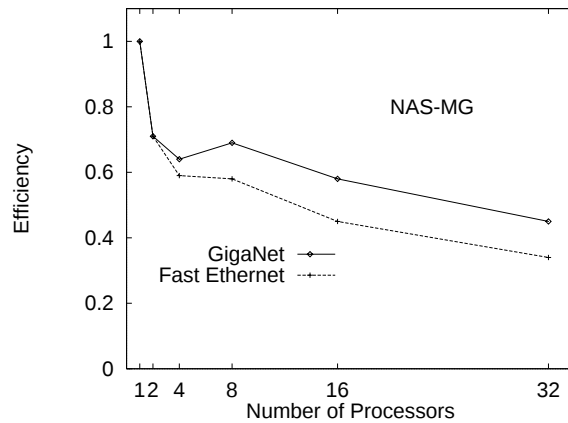
FIG. 6.4. Parallel efficiency obtained by the NAS-MG (class B) benchmarks using a dual node configuration in combination with the GigaNet or the Fast-Ethernet networks.
