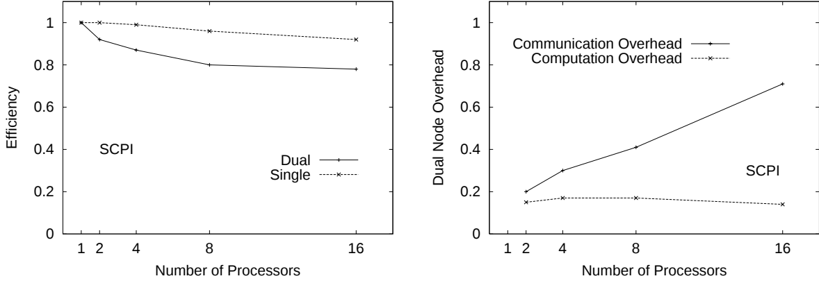
FIG. 6.6. Efficiency for a fixed 32 \times 128 \times 128 problem size (left-hand chart) and dual node communication and computation overheads achieved for the SCPI solver (right-hand chart). These measurements have been obtained over GigaNet.
