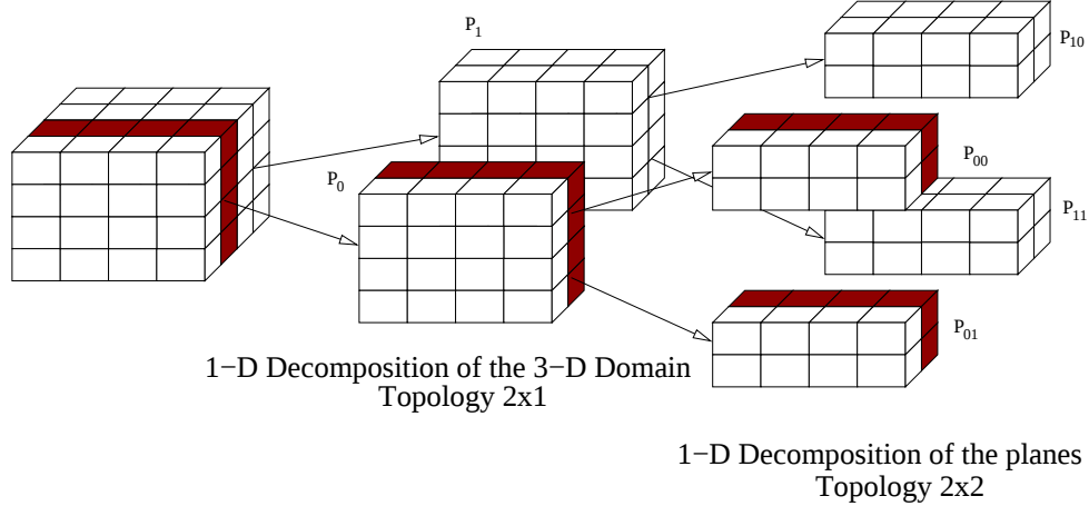
FIG. 5.2. Schematic data distribution of a 2-D data decomposition
