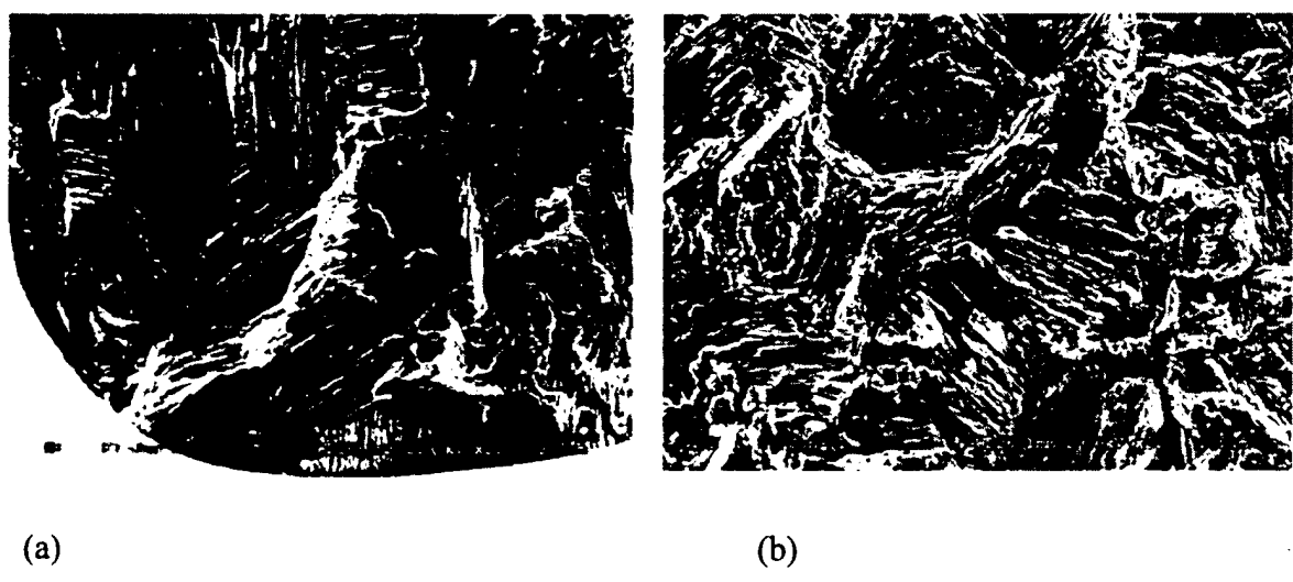
Fig. 4: Fatigue fracture surface of the specimen tested at \sigma_{max} = 450 MPa; (a) crack nucleation region and (b) away from crack origin
