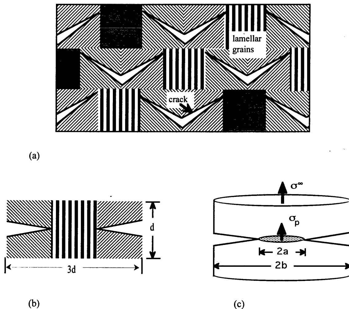
Fig. 5. Schematics of micro-cracking in lamellar Ti_3Al - TiAl polycrystals: (a) idealized crack distribution, (b) a specimen depicting a cracked ligament and (c) the corresponding unit cell
