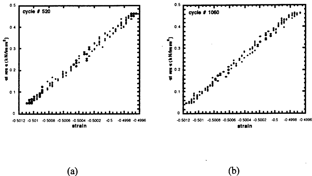
Fig. 5: Hysteresis recorded from S-N fatigue test of the specimen cycled at \sigma_{\max} = 460 MPa; (a) at N = 520 cycles and (b) at N = 1060 cycles
