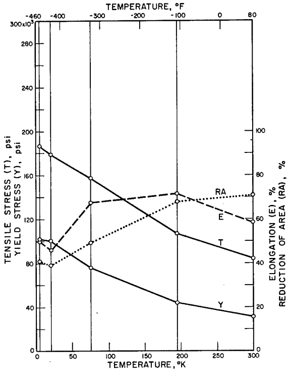
SS 310, ANNEALED
