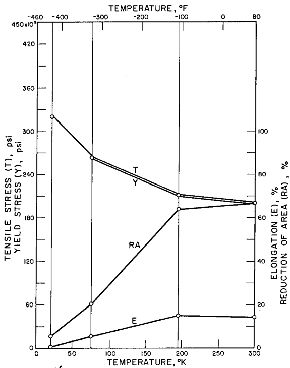
SS 410, HEAT TREATED 1800 °F - 1 HR, OQ, TEMPERED 700 °F - 4 HR, AC
