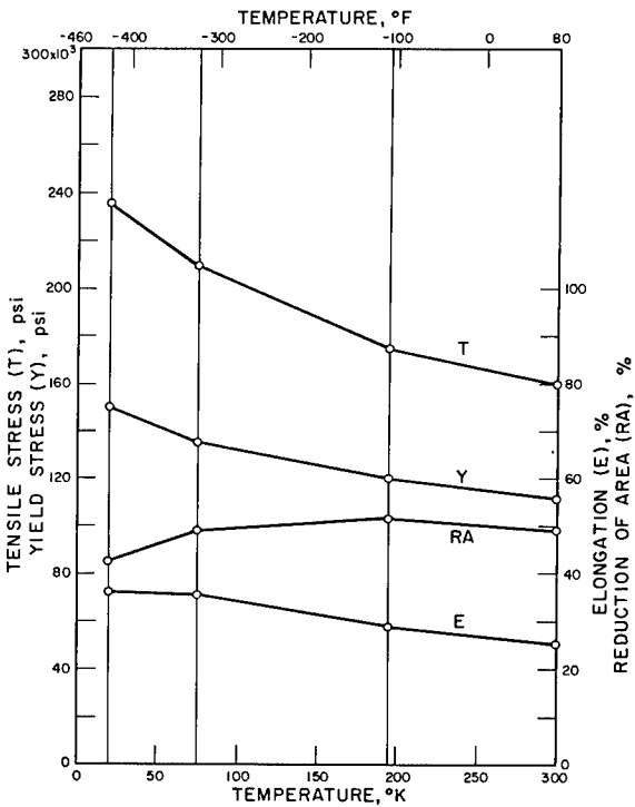
SS A-286, SOLUTION TREATED 1800°F - 1 1/2 HR, AC, AGED AT 1350 °F - 16HR, AC
