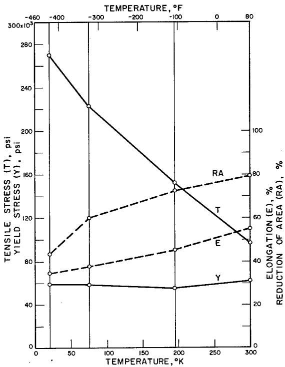
SS 321, ANNEALED
