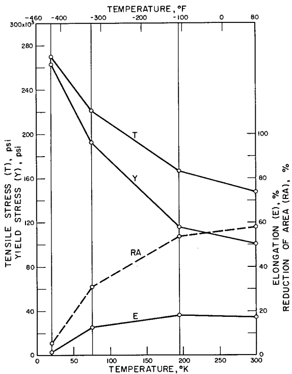
ES 1075, HEAT TREATED 1450 °F - 1HR, OQ, TEMPERED 720 °F - 1HR, AC
