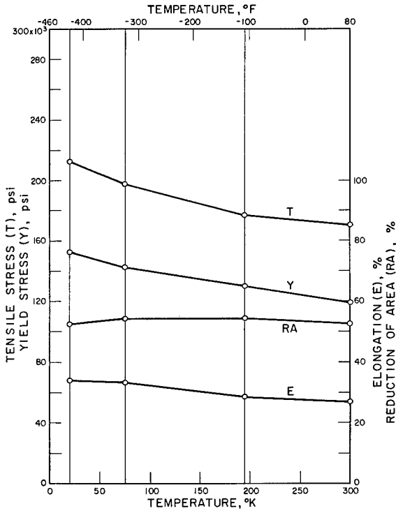
"K" MONEL NiB , AGE HARDENED 1100 °F - 21 HR, 1000 °F - 8 HR, AC
