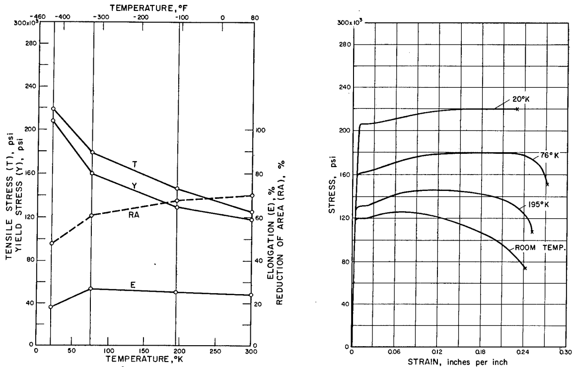
FIGURE 21. TENSILE PROPERTIES OF THE IRON ALLOYS.
