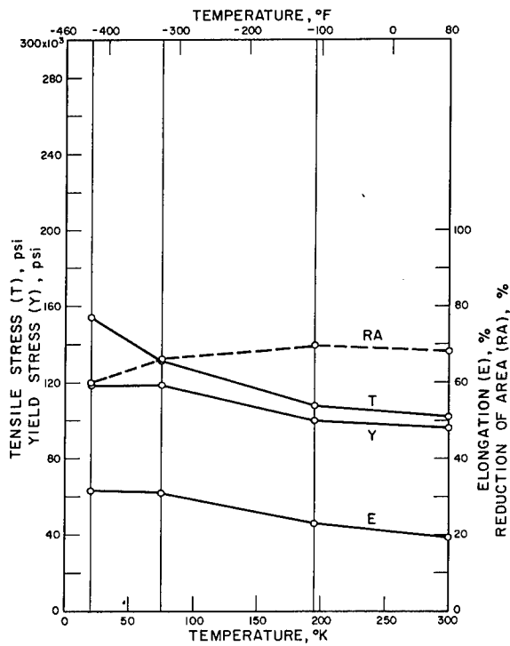
BERYLCO 25 , HARD
