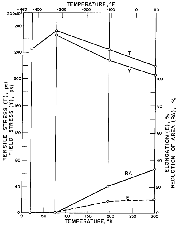
SS 17-7 PH, TH 1050
