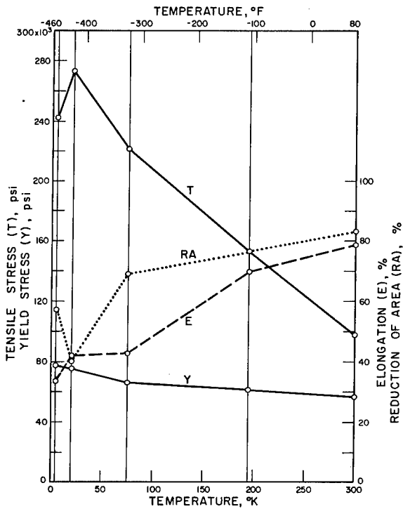
SS 304 L, ANNEALED
