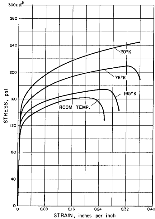
SS A-286, SOLUTION TREATED 1800°F - 1 1/2 HR, AC, AGED AT 1350 °F - 16HR, AC
