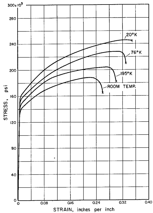
NiB INCONEL "X", HOT ROLLED, DIRECT AGED 1300 °F - 20 HR. AC TEMPERED
