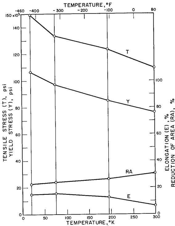
"S" MONEL NiB , CAST, ANNEALED 1600 °F - 1 HR, 1300 °F - 1/2 HR, OQ
