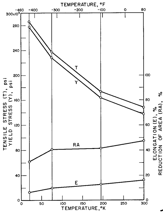
6Al-4V, ANNEALED
