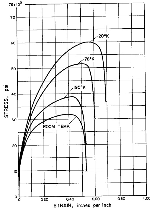
70/30 BRASS , 3/4 HARD
