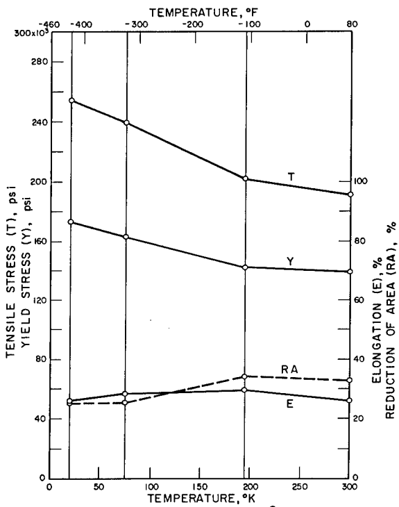
NiB RENÉ 41, SOLUTION TREATED 1975 °F - 4 HR, WQ
