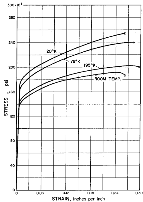
NiB RENÉ 41, SOLUTION TREATED 1975 °F - 4 HR, WQ
