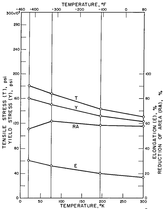
NiB INCONEL, 20% COLD DRAWN
