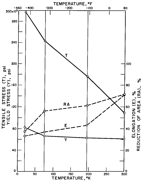
SS 303, ANNEALED
