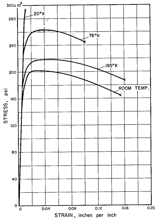
SS 416, HEAT TREATED 1800 °F - 1HR, OQ, TEMPERED 700 °F - 4HR, AC
