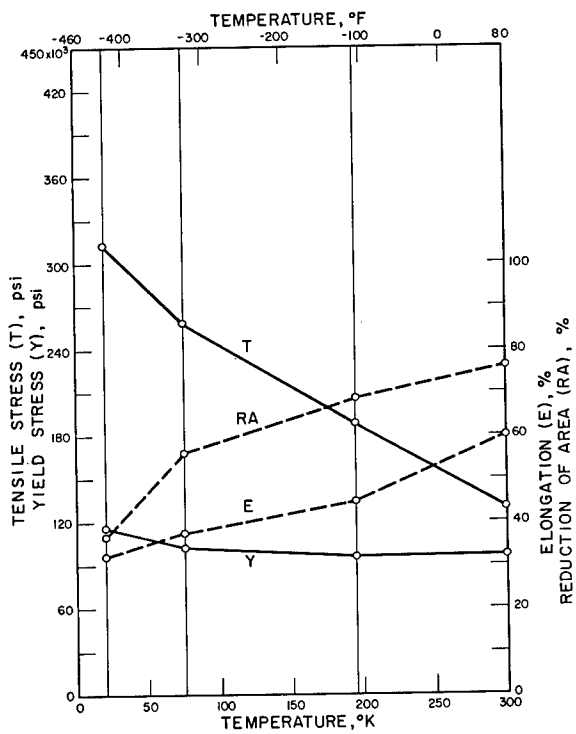
SS 302, COLD DRAWN
