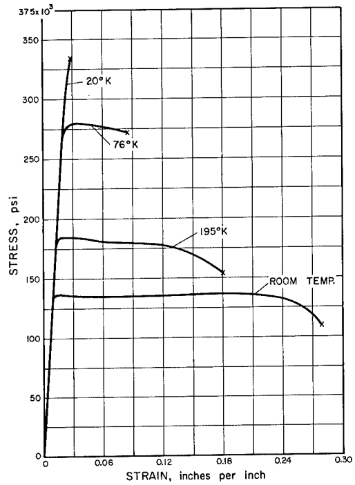
Ti 13V - 11Cr - 3Al, SOLUTION TREATED
