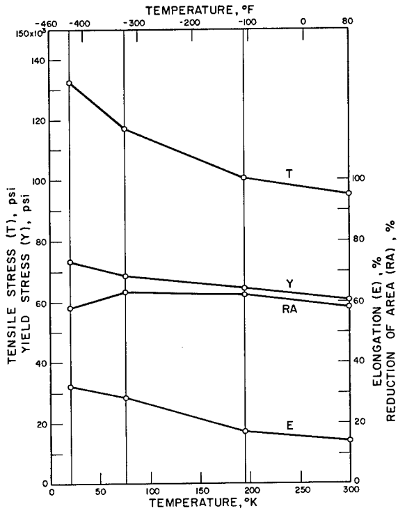
70/30 BRASS , 3/4 HARD
