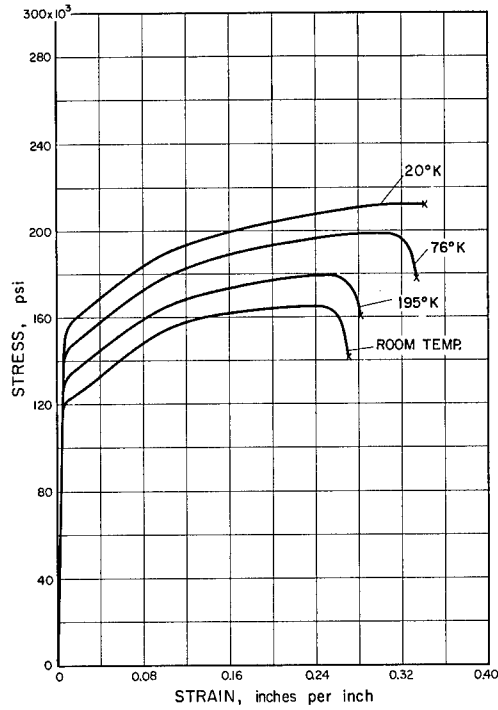
"K" MONEL NiB , AGE HARDENED 1100 °F - 21 HR, 1000 °F - 8 HR, AC
