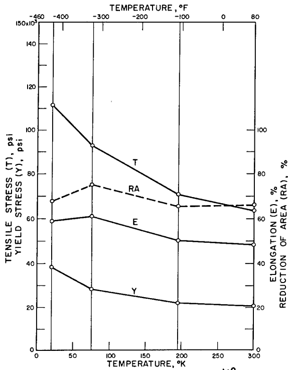
NiB "A" NICKEL, ANNEALED 1725 °F - 1/2 HR
