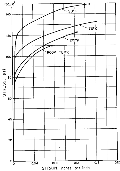
"S" MONEL NiB , CAST, ANNEALED 1600 °F - 1 HR, 1300 °F - 1/2 HR, OQ
