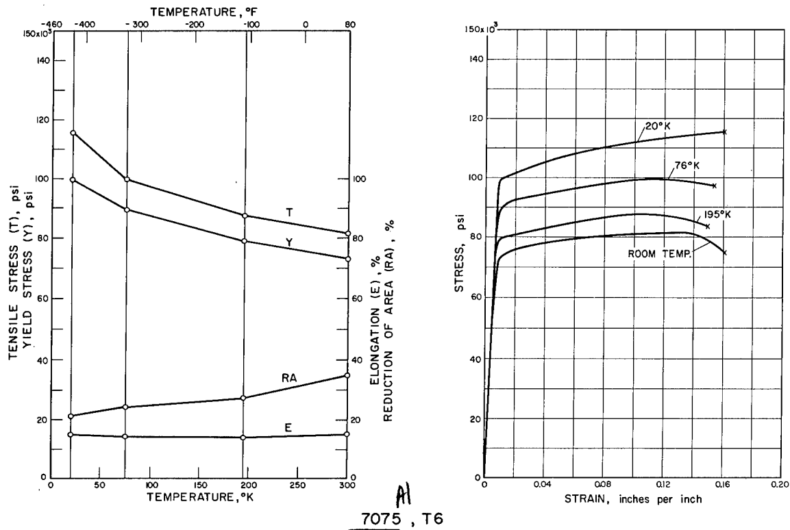
FIGURE 6. TENSILE PROPERTIES OF THE ALUMINUM ALLOYS.
