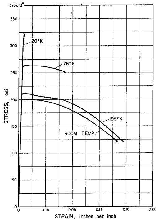
SS 410, HEAT TREATED 1800 °F - 1 HR, OQ, TEMPERED 700 °F - 4 HR, AC
