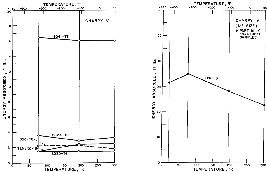
FIGURE 7. IMPACT PROPERTIES OF THE ALUMINUM ALLOYS.
