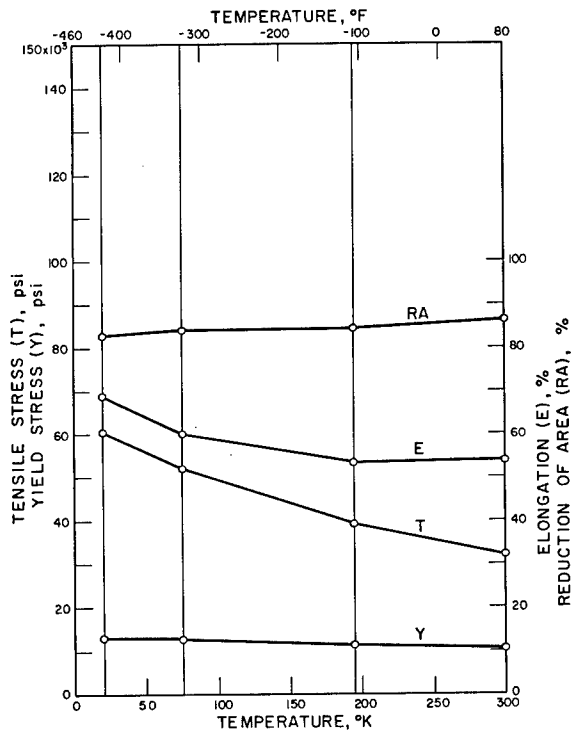
OFHC , SOFT
