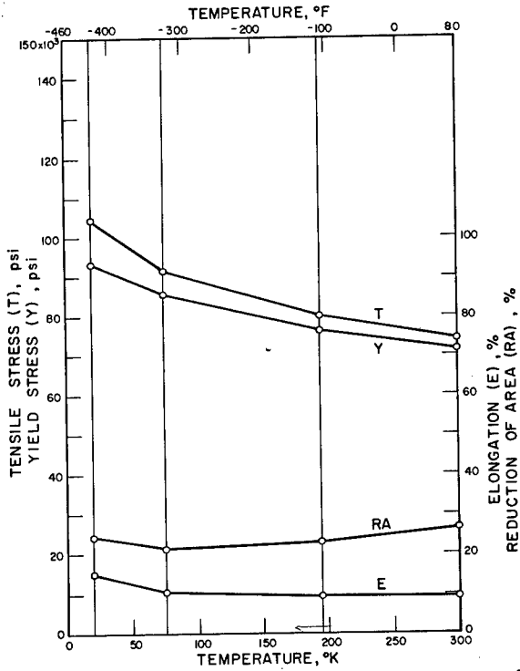
2024 Al, T86
