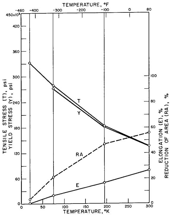
Ti 13V - 11Cr - 3Al, SOLUTION TREATED
