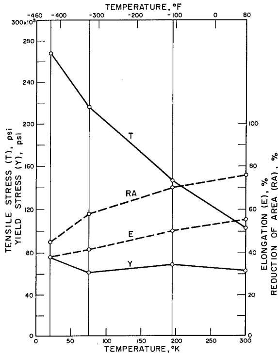
SS 347, ANNEALED
