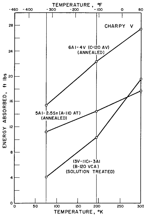
FIGURE 29. IMPACT PROPERTIES OF THE TITANIUM ALLOYS.
