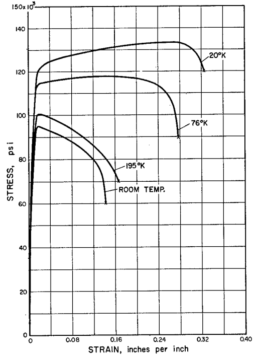
70/30 BRASS , 3/4 HARD
