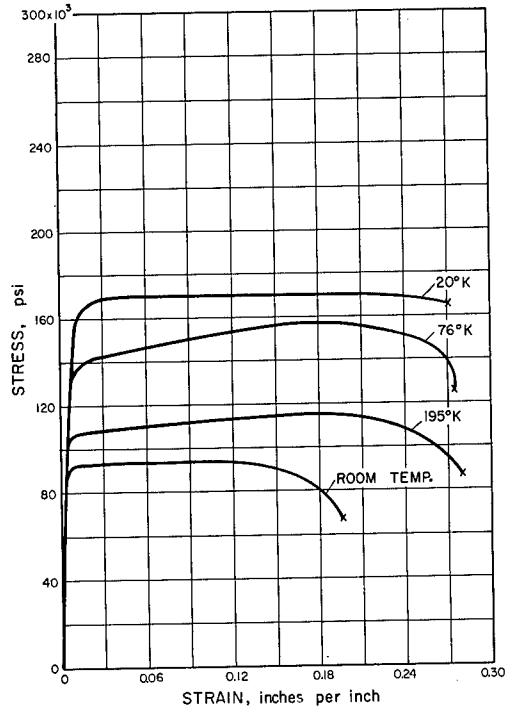
FeB INVAR 36, 12-15% COLD DRAWN
