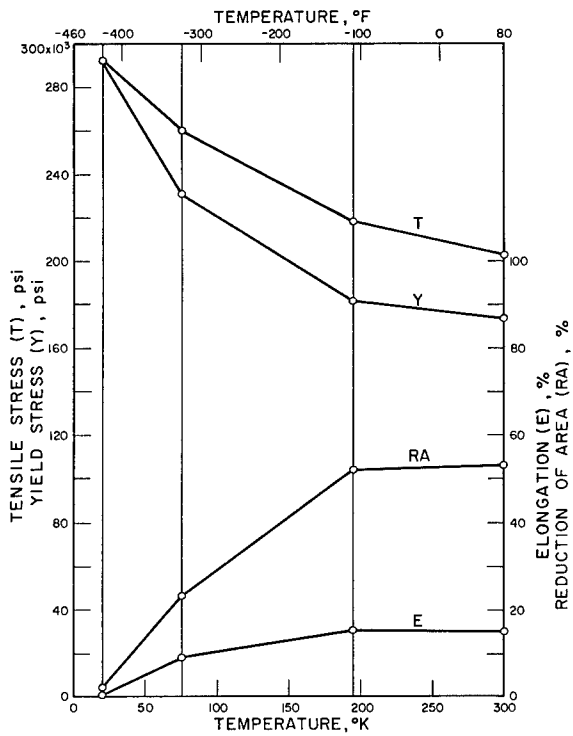
SS 416, HEAT TREATED 1800 °F - 1HR, OQ, TEMPERED 700 °F - 4HR, AC
