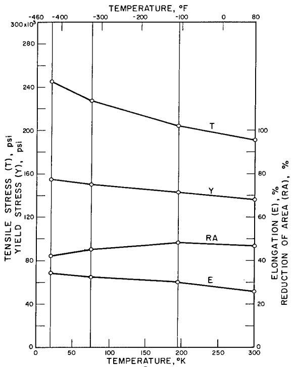
NiB INCONEL "X", HOT ROLLED, DIRECT AGED 1300 °F - 20 HR. AC TEMPERED
