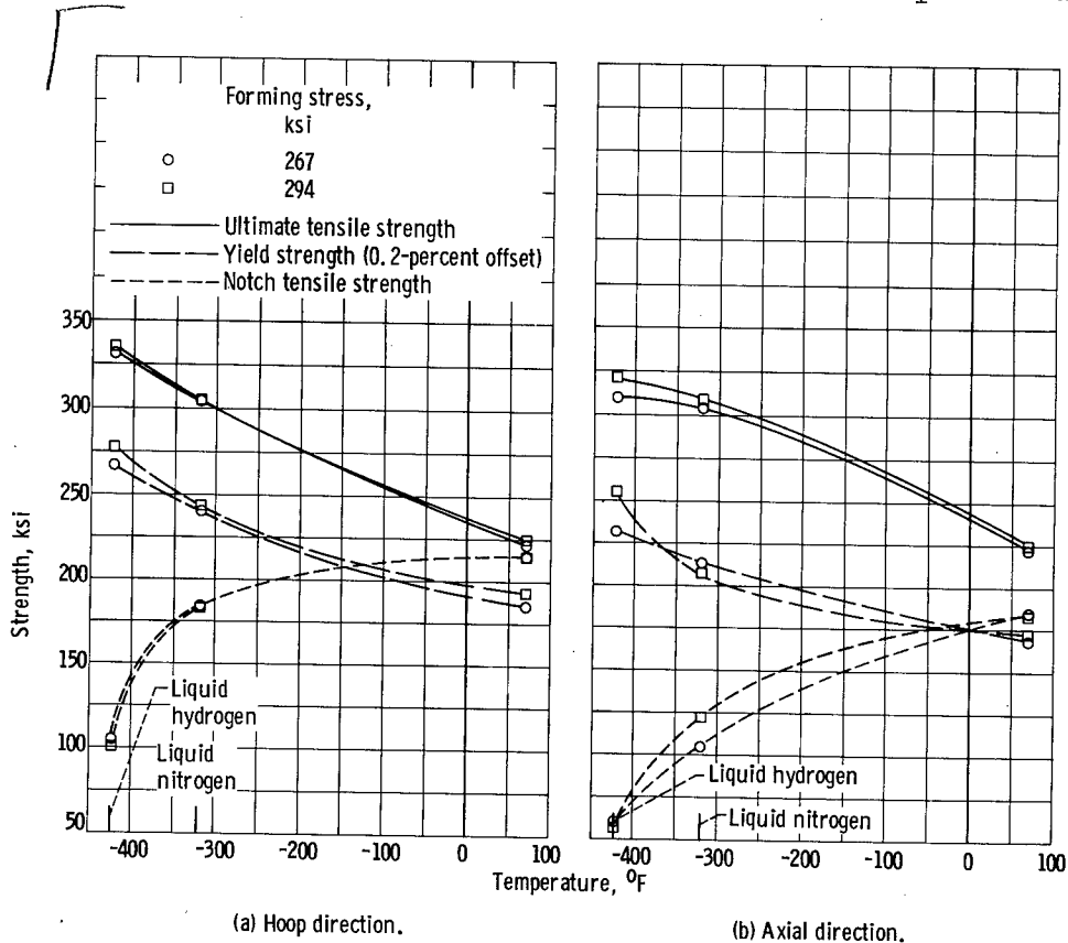
Figure 5. - Strength properties of cryoformed AISI 301 stainless steel as functions of temperature.
