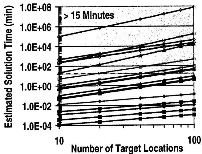
Figure 38 Scalability Assessment of ADP Algorithms Developed and Implemented for Hybrid, Multi-Rate Control Architecture (125 CPUs)
