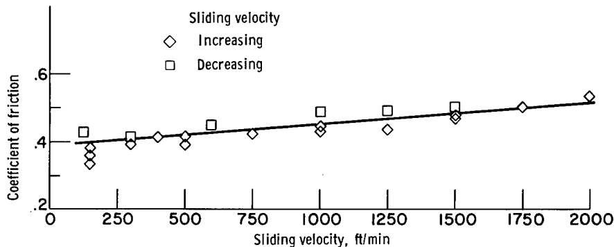
Figure 10. - Coefficient of friction of samarium sliding on 440-C stainless steel in vacuum ( 10^{-9} mm Hg). Load, 1000 grams; ambient temperature, 75° F.
