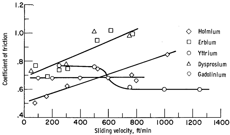
Figure 9. - Coefficient of friction of various rare-earth metals sliding on 440-C stainless steel in vacuum ( 10^{-9} mm Hg). Load, 1000 grams; ambient temperature, 75° F.
