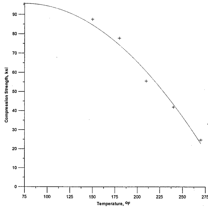
FIGURE 18. VARIATION OF COMPRESSION STRENGTH VALUES AS A FUNCTION OF TEMPERATURE FOR FIBERCOTE E 765/T300 3KPW CARBON FABRIC MATERIAL SYSTEM (68% RH)
