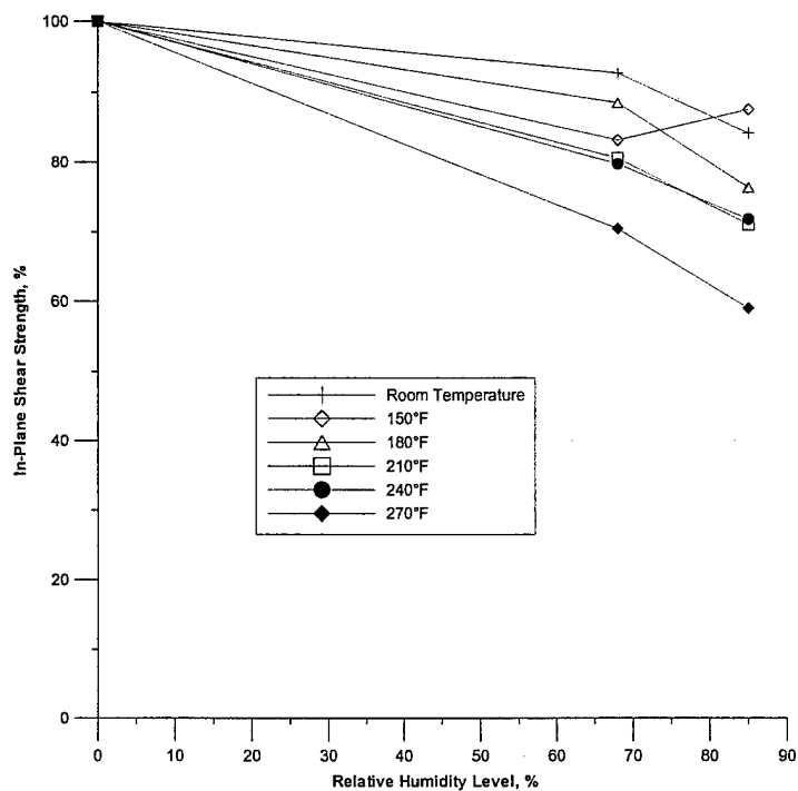
FIGURE 38. VARIATION IN THE PERCENTAGE OF IN-PLANE SHEAR STRENGTH VALUES AS A FUNCTION OF RELATIVE HUMIDITY LEVEL FOR THE SIX TEMPERATURES CONSIDERED FOR NEWPORT 7781/NB321 MATERIAL SYSTEM
