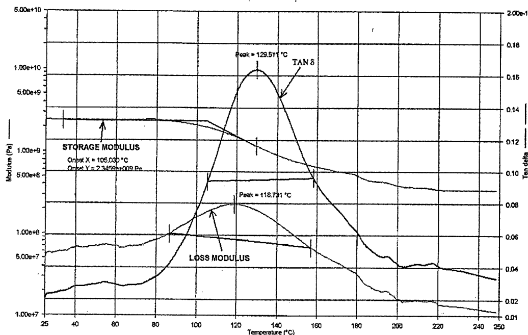
FIGURE A-3. A TYPICAL DMA RESULT
