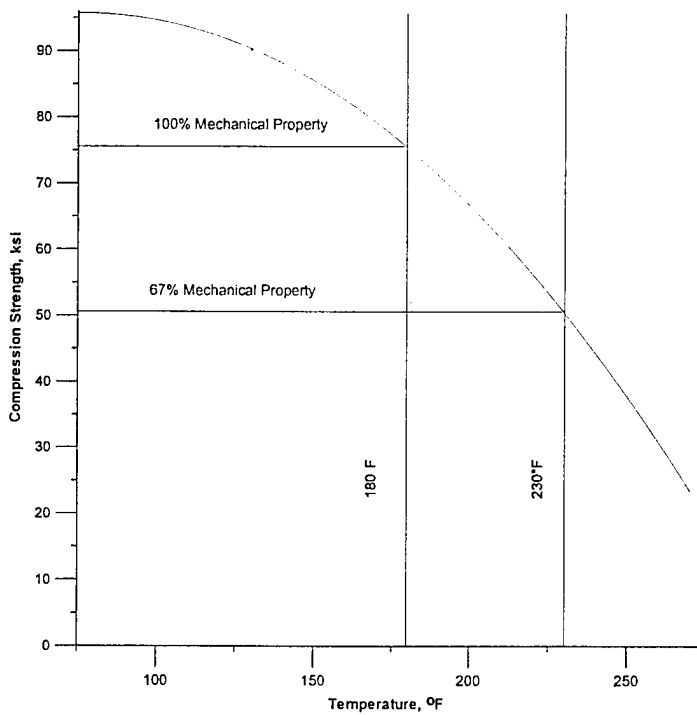
FIGURE 72. TWO-THIRD RETENTION METHOD SHOWN FOR FIBERCOTE E 765/T300 3KPW CARBON FABRIC COMPRESSION STRENGTH (68% RH)
