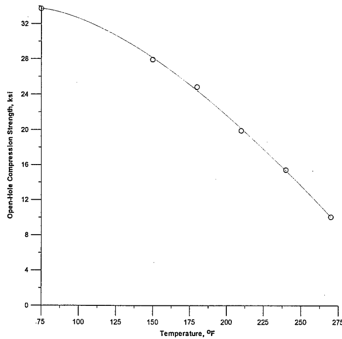
FIGURE 19. VARIATION OF OPEN-HOLE COMPRESSION STRENGTH VALUES AS A FUNCTION OF TEMPERATURE FOR FIBERCOTE E 765/T300 3KPW CARBON FABRIC MATERIAL SYSTEM (68% RH)
