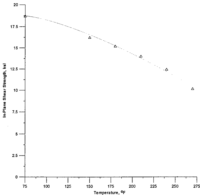
FIGURE 7. VARIATION OF IN-PLANE SHEAR STRENGTH VALUES AS A FUNCTION OF TEMPERATURE FOR FIBERCOTE E 765/T300 3KPW CARBON FABRIC MATERIAL SYSTEM (0% RH)
