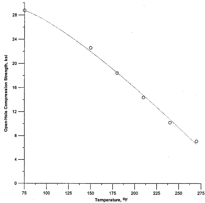
FIGURE 24. VARIATION OF OPEN-HOLE COMPRESSION STRENGTH VALUES AS A FUNCTION OF TEMPERATURE FOR NEWPORT 7781/NB321 GLASS FABRIC MATERIAL SYSTEM (85% RH)
