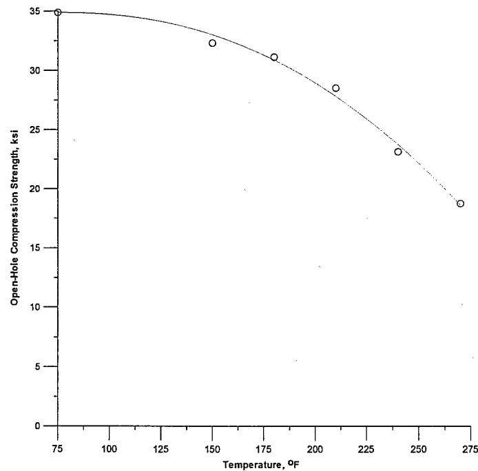
FIGURE 9. VARIATION OF OPEN-HOLE COMPRESSION STRENGTH VALUES AS A FUNCTION OF TEMPERATURE FOR FIBERCOTE E 765/T300 3KPW CARBON FABRIC MATERIAL SYSTEM (0% RH)
