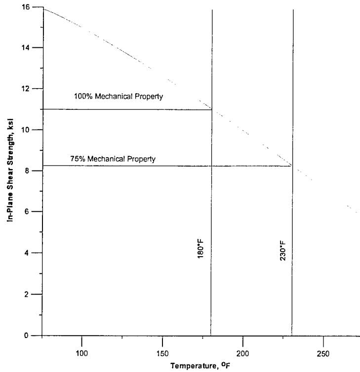
FIGURE 78. TWO-THIRD RETENTION METHOD SHOWN FOR FIBERCOTE E 765/T300 3KPW CARBON FABRIC IN-PLANE SHEAR STRENGTH (85% RH)
