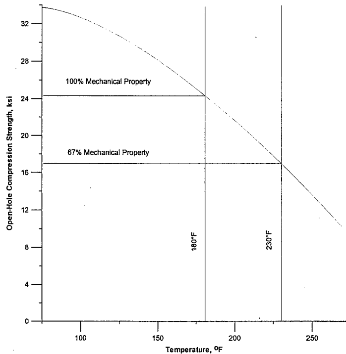
FIGURE 73. TWO-THIRD RETENTION METHOD SHOWN FOR FIBERCOTE E 765/T300 3KPW CARBON FABRIC OPEN-HOLE COMPRESSION STRENGTH (68% RH)
