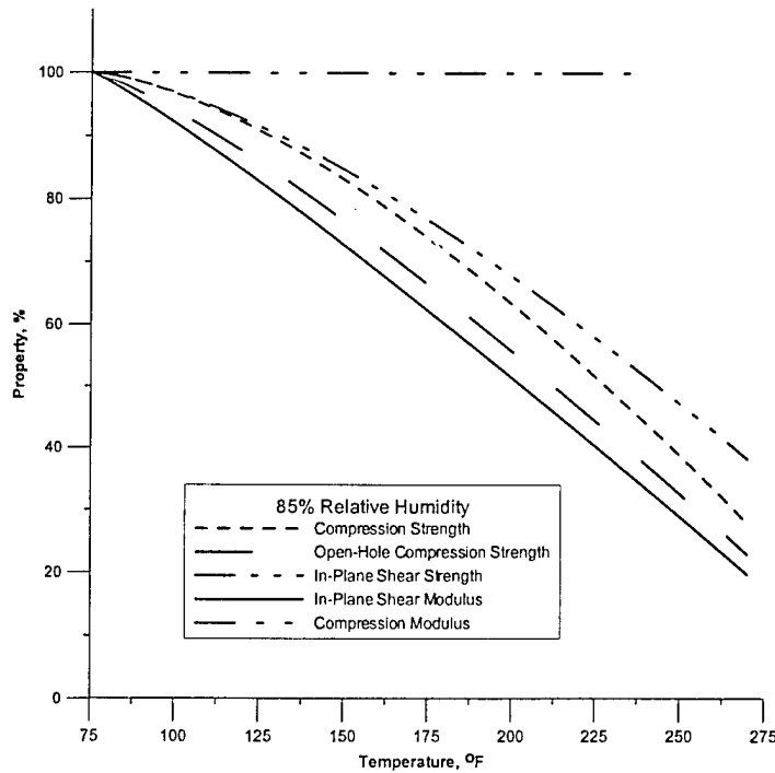
FIGURE 34. VARIATION IN THE PERCENTAGE OF MECHANICAL PROPERTIES AS A FUNCTION OF TEMPERATURE FOR NEWPORT 7781/NB321 GLASS FABRIC SPECIMENS CONDITIONED AT 85% RH
