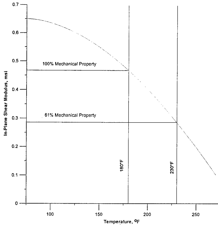
FIGURE 67. TWO-THIRD RETENTION METHOD SHOWN FOR NEWPORT 7781/NB321 GLASS FABRIC IN-PLANE SHEAR MODULUS (68% RH)
