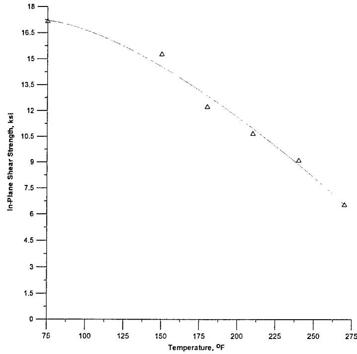
FIGURE 22. VARIATION OF IN-PLANE SHEAR STRENGTH VALUES AS A FUNCTION OF TEMPERATURE FOR NEWPORT 7781/NB321 GLASS FABRIC MATERIAL SYSTEM (85% RH)
