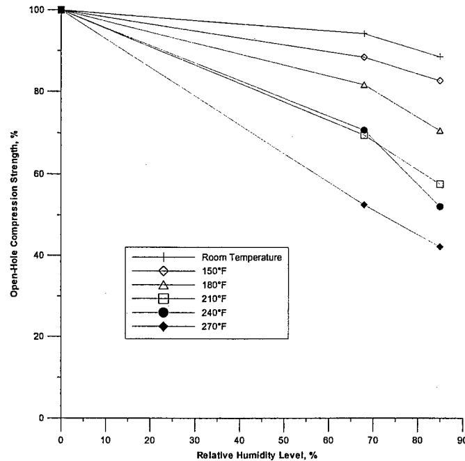
FIGURE 42. VARIATION IN THE PERCENTAGE OF OPEN-HOLE COMPRESSION STRENGTH VALUES AS A FUNCTION OF RELATIVE HUMIDITY LEVEL FOR THE SIX TEMPERATURES CONSIDERED FOR NEWPORT 7781/NB321 MATERIAL SYSTEM
