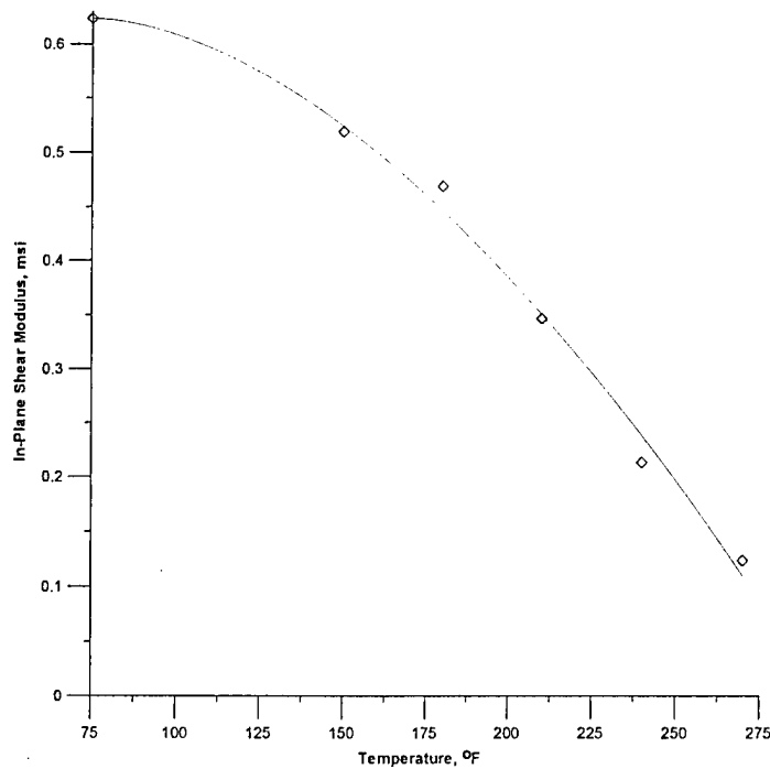
FIGURE 20. VARIATION OF IN-PLANE SHEAR MODULUS VALUES AS A FUNCTION OF TEMPERATURE FOR FIBERCOTE E 765/T300 3Kpw CARBON FABRIC MATERIAL SYSTEM (68% RH)
