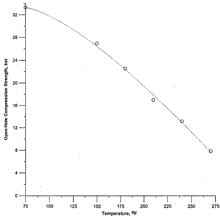
FIGURE 29. VARIATION OF OPEN-HOLE COMPRESSION STRENGTH VALUES AS A FUNCTION OF TEMPERATURE FOR FIBERCOTE E 765/T300 3KPW CARBON FABRIC MATERIAL SYSTEM (85% RH)
