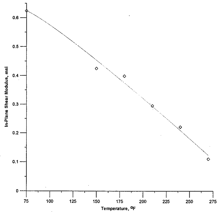
FIGURE 25. VARIATION OF IN-PLANE SHEAR MODULUS VALUES AS A FUNCTION OF TEMPERATURE FOR NEWPORT 7781/NB321 GLASS FABRIC MATERIAL SYSTEM (85% RH)
