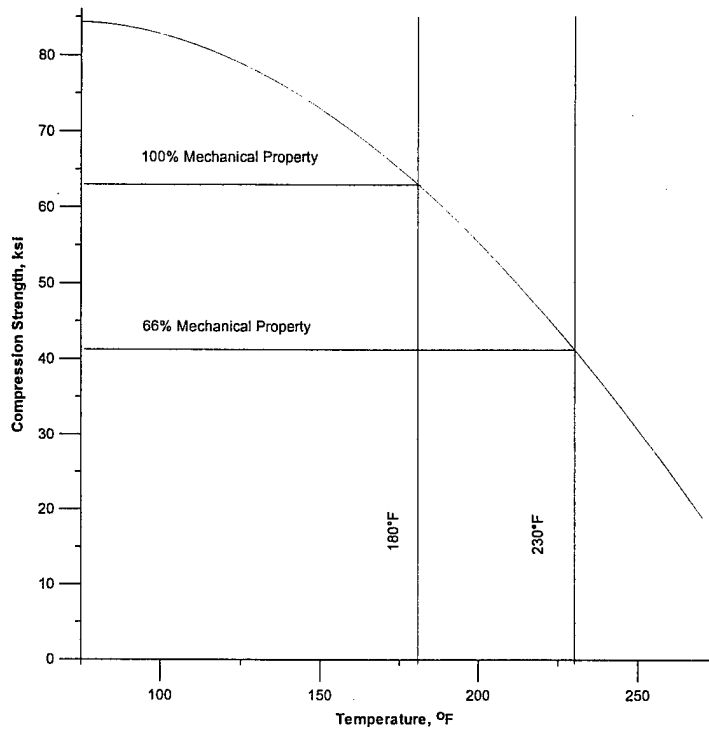
FIGURE 80. TWO-THIRD RETENTION METHOD SHOWN FOR FIBERCOTE E 765/T300 3KPW CARBON FABRIC COMPRESSION STRENGTH (85% RH)
