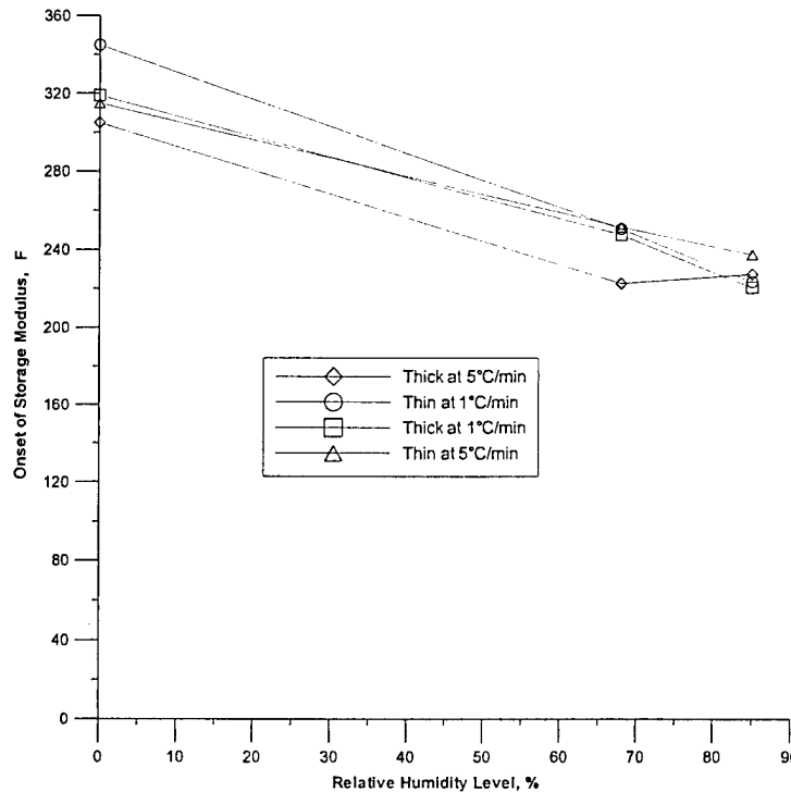
FIGURE 51. VARIATION IN THE ONSET OF STORAGE MODULUS VALUES AS A FUNCTION OF RELATIVE HUMIDITY LEVEL FOR FIBERCOTE E 765/T300 3KPW MATERIAL SYSTEM
