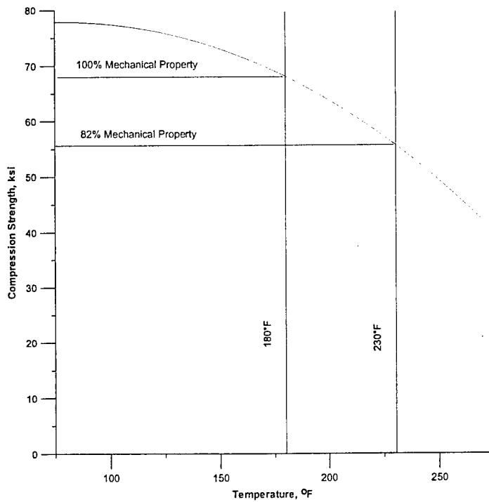
FIGURE 60. TWO-THIRD RETENTION METHOD SHOWN FOR NEWPORT 7781/NB321 GLASS FABRIC COMPRESSION STRENGTH (0% RH)
