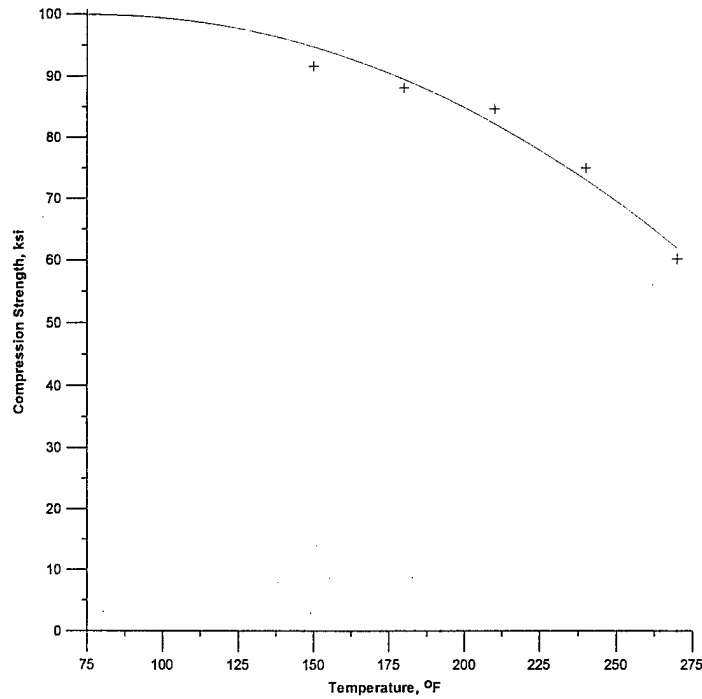
FIGURE 8. VARIATION OF COMPRESSION STRENGTH VALUES AS A FUNCTION OF TEMPERATURE FOR FIBERCOTE E 765/T300 3KPW CARBON FABRIC MATERIAL SYSTEM (0% RH)
