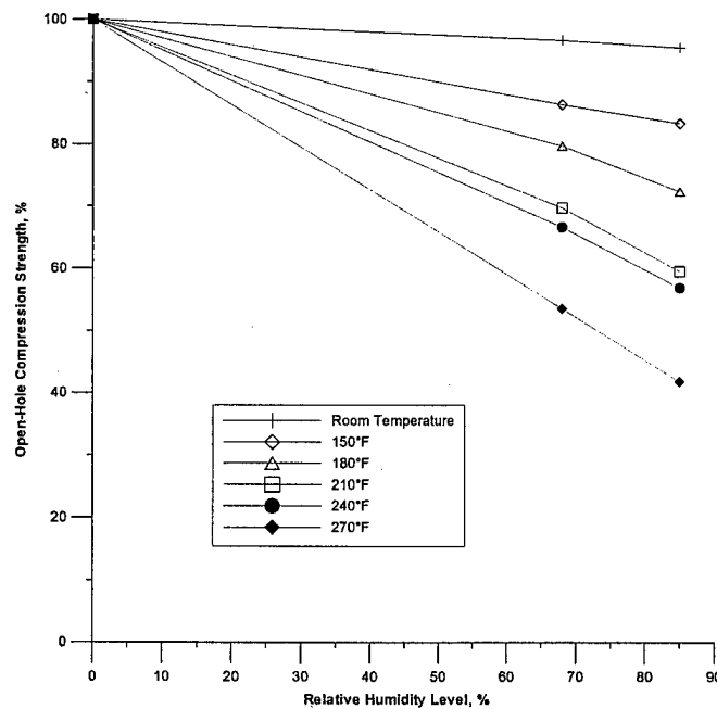
FIGURE 47. VARIATION IN THE PERCENTAGE OF OPEN-HOLE COMPRESSION STRENGTH VALUES AS A FUNCTION OF RELATIVE HUMIDITY LEVEL FOR THE SIX TEMPERATURES CONSIDERED FOR FIBERCOTE E 765/T300 3KPW MATERIAL SYSTEM
