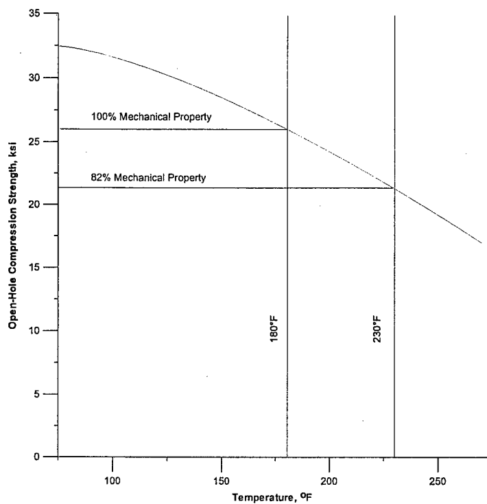
FIGURE 61. TWO-THIRD RETENTION METHOD SHOWN FOR NEWPORT 7781/NB321 GLASS FABRIC OPEN-HOLE COMPRESSION STRENGTH (0% RH)
