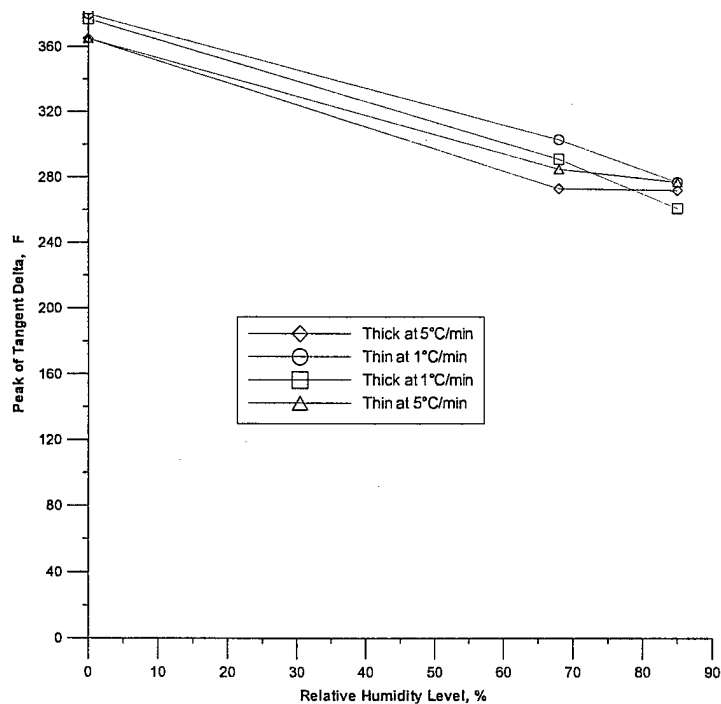
FIGURE 50. VARIATION IN THE PEAK OF TANGENT DELTA VALUES AS A FUNCTION OF RELATIVE HUMIDITY LEVEL FOR FIBERCOTE E 765/T300 3KPW MATERIAL SYSTEM
