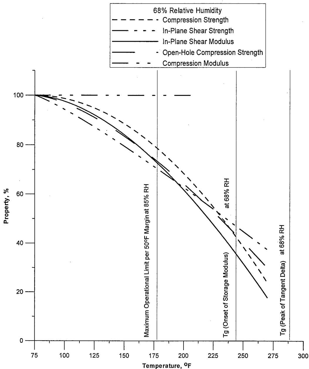
FIGURE 56. MATERIAL OPERATIONAL LIMIT AS PREDICTED BY THE 50°F MARGIN METHOD BASED ON THE RESULTS FOR FIBERCOTE E 765/T300 3KPW CARBON FABRIC SPECIMENS CONDITIONED AT 68% RH
