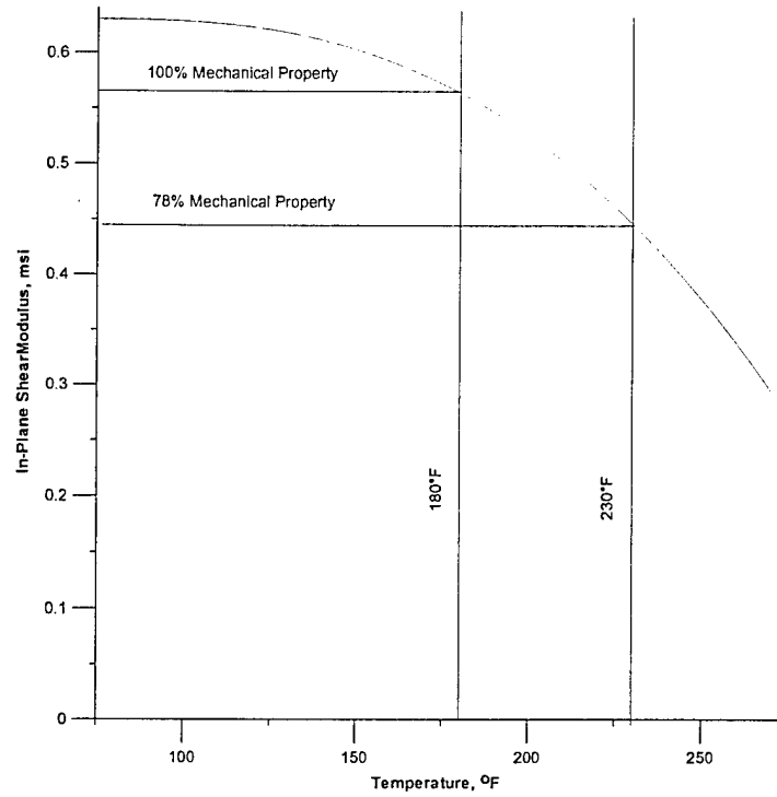
FIGURE 63. TWO-THIRD RETENTION METHOD SHOWN FOR FIBERCOTE E 765/T300 3KPW CARBON FABRIC IN-PLANE SHEAR MODULUS (0% RH)
