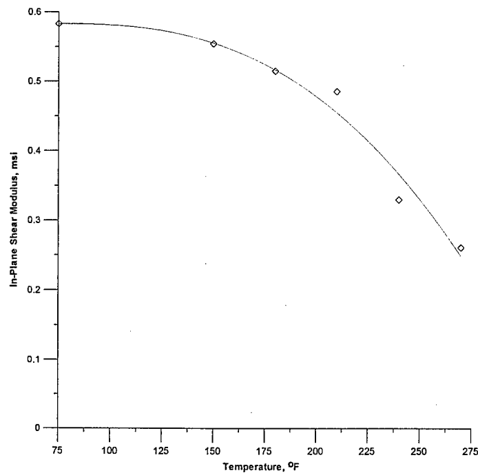
FIGURE 5. VARIATION OF IN-PLANE SHEAR MODULUS VALUES AS A FUNCTION OF TEMPERATURE FOR NEWPORT 7781/NB321 GLASS FABRIC MATERIAL SYSTEM (0% RH)
