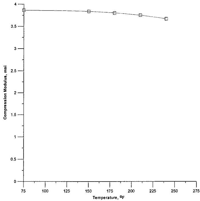
FIGURE 6. VARIATION OF COMPRESSION MODULUS VALUES AS A FUNCTION OF TEMPERATURE FOR NEWPORT 7781/NB321 GLASS FABRIC MATERIAL SYSTEM (0% RH)
