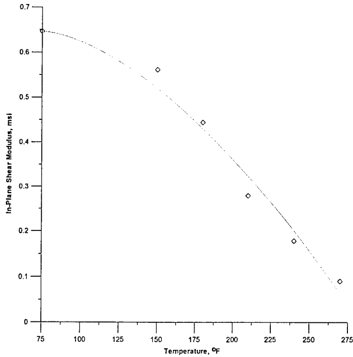
FIGURE 30. VARIATION OF IN-PLANE SHEAR MODULUS VALUES AS A FUNCTION OF TEMPERATURE FOR FIBERCOTE E 765/T300 3KPW CARBON FABRIC MATERIAL SYSTEM (85% RH)
