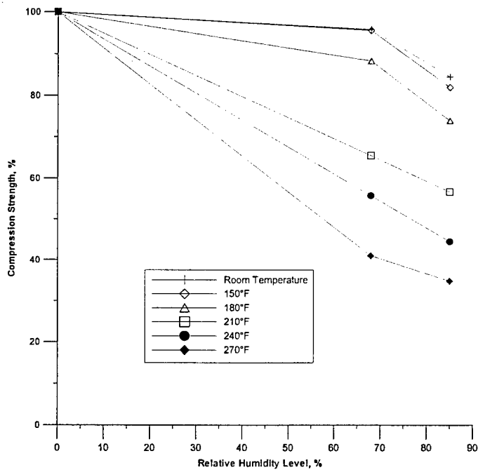
FIGURE 45. VARIATION IN THE PERCENTAGE OF COMPRESSION TRENGTH VALUES AS A FUNCTION OF RELATIVE HUMIDITY LEVEL FOR THE SIX TEMPERATURES CONSIDERED FOR FIBERCOTE E 765/T300 3KPW MATERIAL SYSTEM
