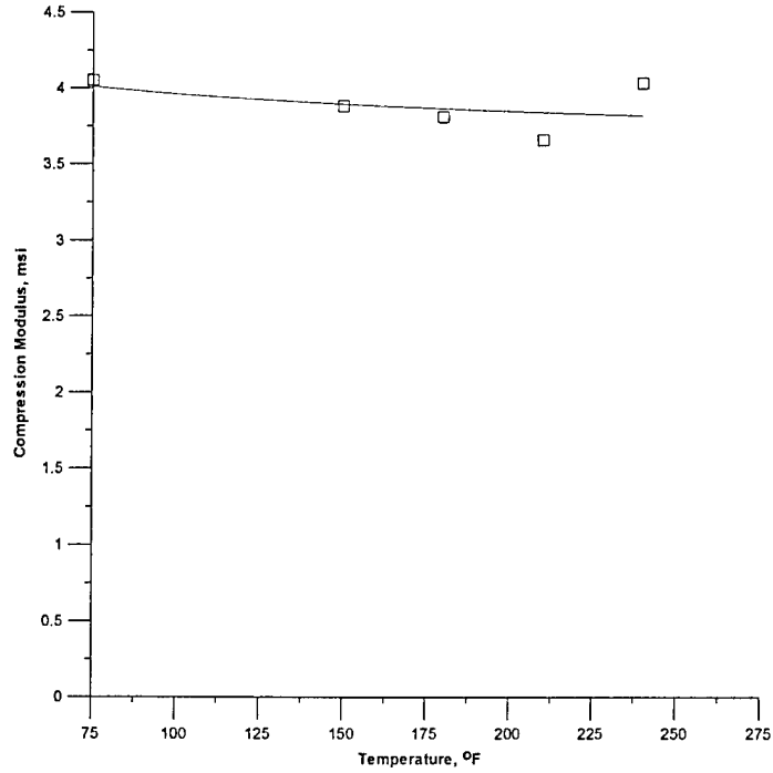
FIGURE 16. VARIATION OF COMPRESSION MODULUS VALUES AS A FUNCTION OF TEMPERATURE FOR NEWPORT 7781/NB321 GLASS FABRIC MATERIAL SYSTEM (68% RH)
