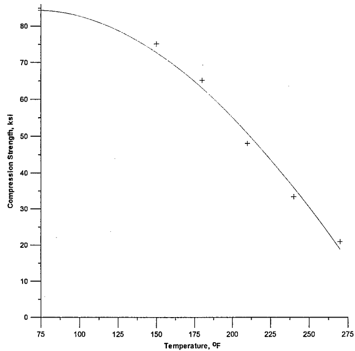
FIGURE 28. VARIATION OF COMPRESSION STRENGTH VALUES AS A FUNCTION OF TEMPERATURE FOR FIBERCOTE E 765/T300 3KPW CARBON FABRIC MATERIAL SYSTEM (85% RH)
