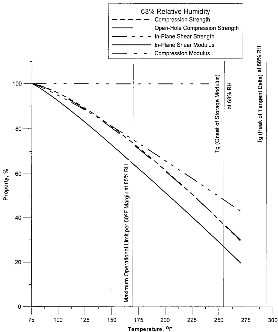
FIGURE 53. MATERIAL OPERATIONAL LIMIT AS PREDICTED BY THE 50°F MARGIN METHOD AT 85% RH BASED ON THE RESULTS FOR NEWPORT 7781/NB321 GLASS FABRIC SPECIMENS CONDITIONED AT 68% RH
