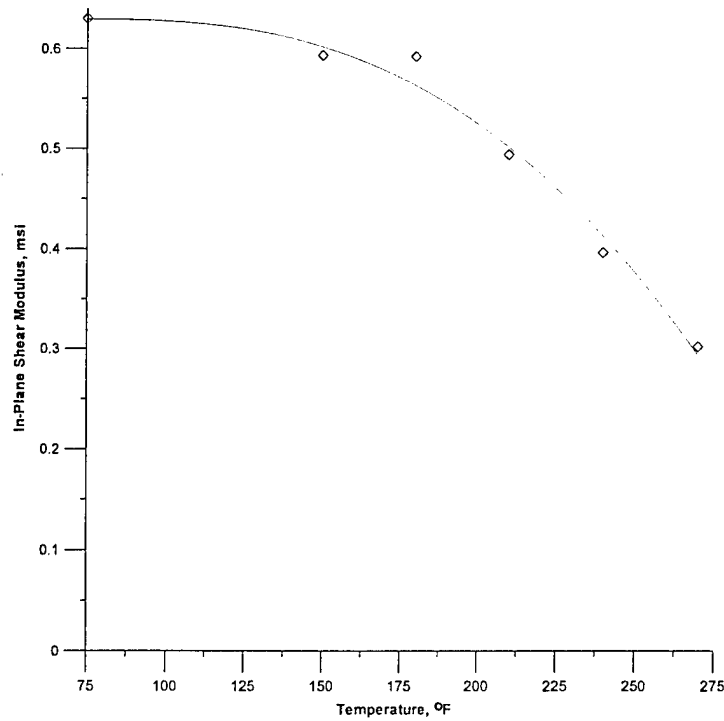
FIGURE 10. VARIATION OF IN-PLANE SHEAR MODULUS VALUES AS A FUNCTION OF TEMPERATURE FOR FIBERCOTE E 765/T300 3KPW CARBON FABRIC MATERIAL SYSTEM (0% RH)
