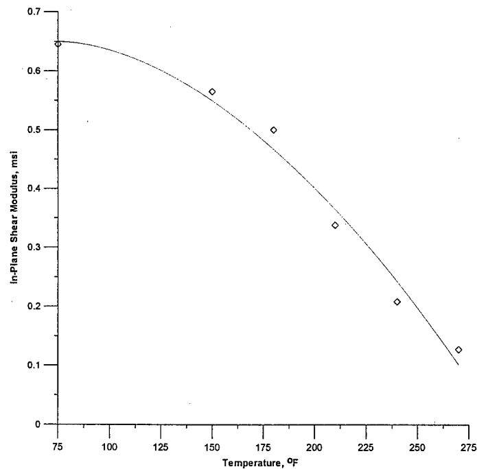
FIGURE 15. VARIATION OF IN-PLANE SHEAR MODULUS VALUES AS A FUNCTION OF TEMPERATURE FOR NEWPORT 7781/NB321 GLASS FABRIC MATERIAL SYSTEM (68% RH)
