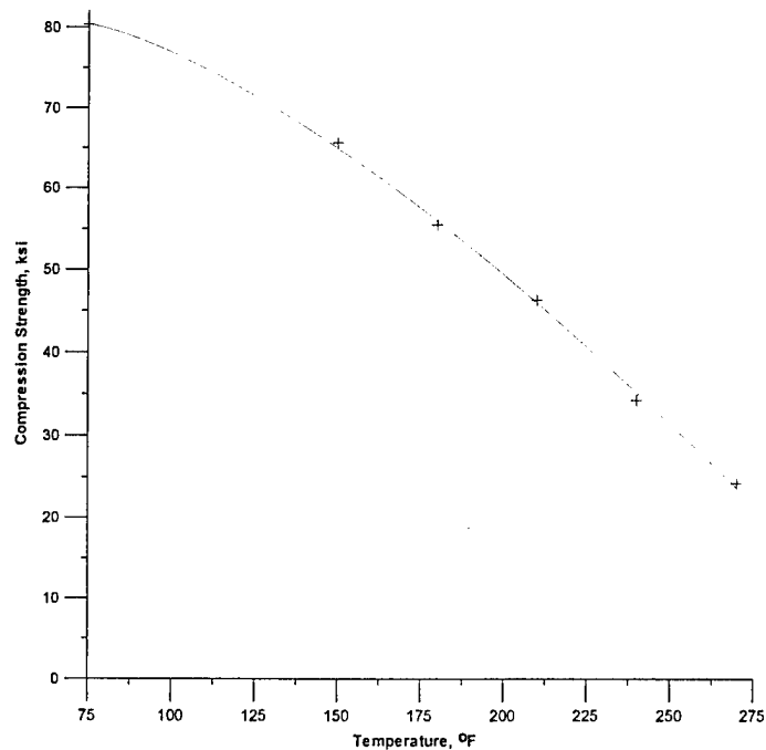
FIGURE 13. VARIATION OF COMPRESSION STRENGTH VALUES AS A FUNCTION OF TEMPERATURE FOR NEWPORT 7781/NB321 GLASS FABRIC MATERIAL SYSTEM (68% RH)
