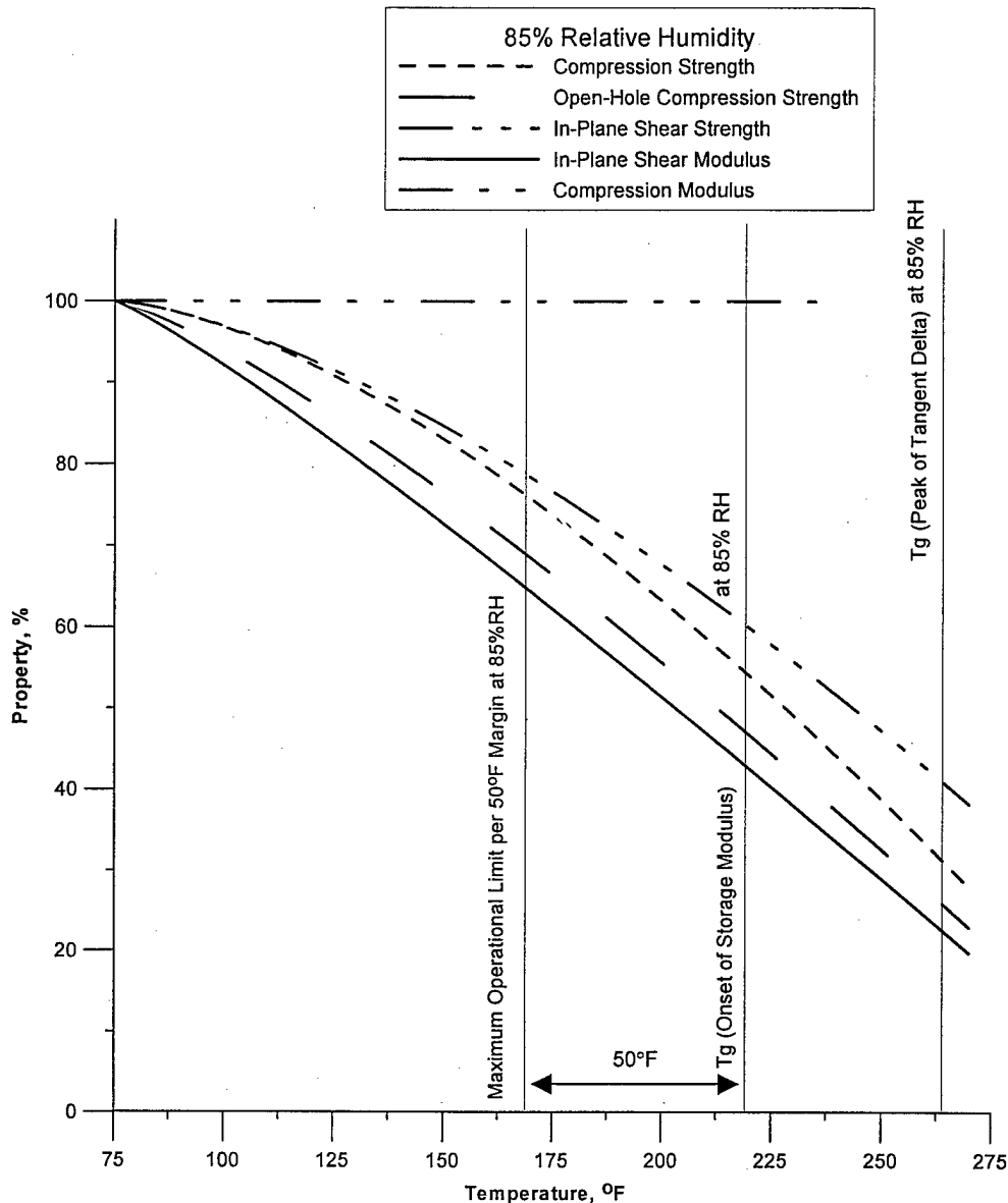
FIGURE 54. MATERIAL OPERATIONAL LIMIT AS PREDICTED BY THE 50°F MARGIN METHOD AT 85% RH BASED ON THE RESULTS FOR NEWPORT 7781/NB321 GLASS FABRIC SPECIMENS CONDITIONED AT 85% RH
