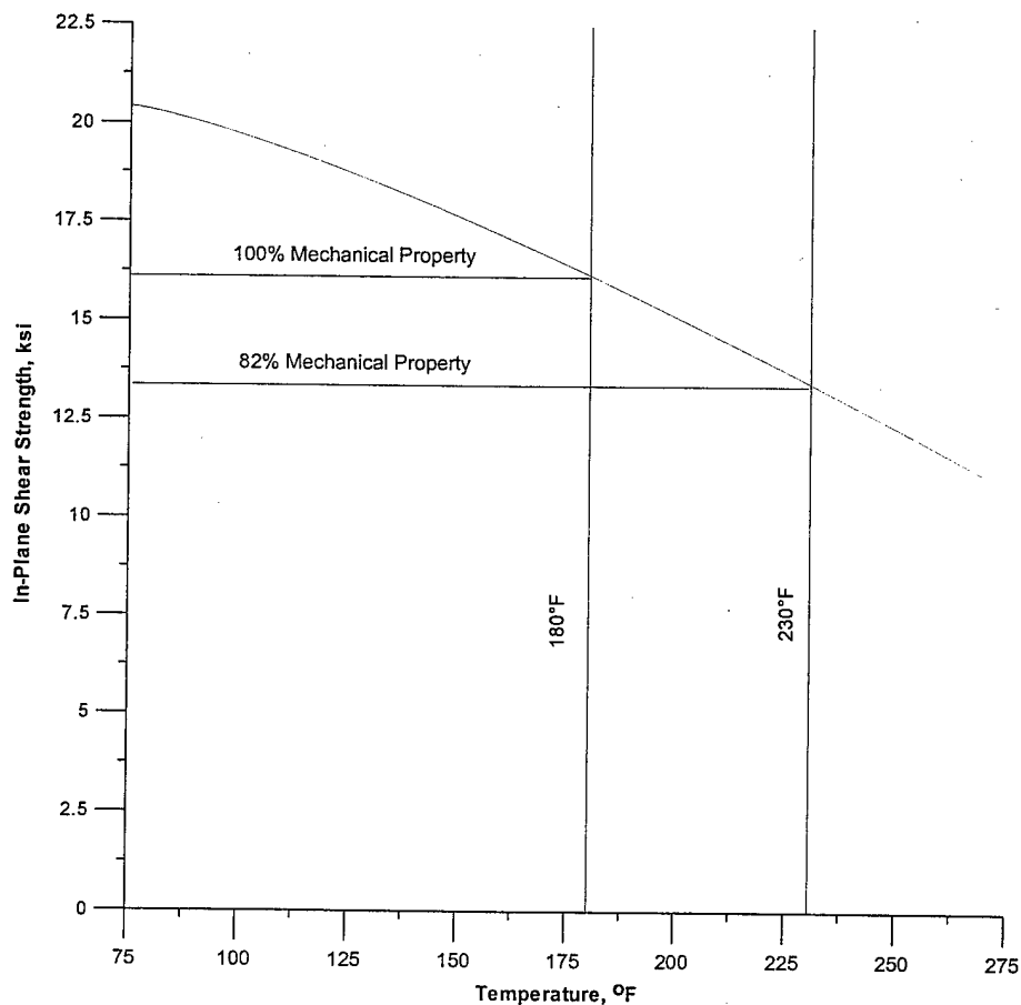
FIGURE 58. TWO-THIRD RETENTION METHOD SHOWN FOR NEWPORT 7781/NB321 GLASS FABRIC IN-PLANE SHEAR STRENGTH (0% RH)
