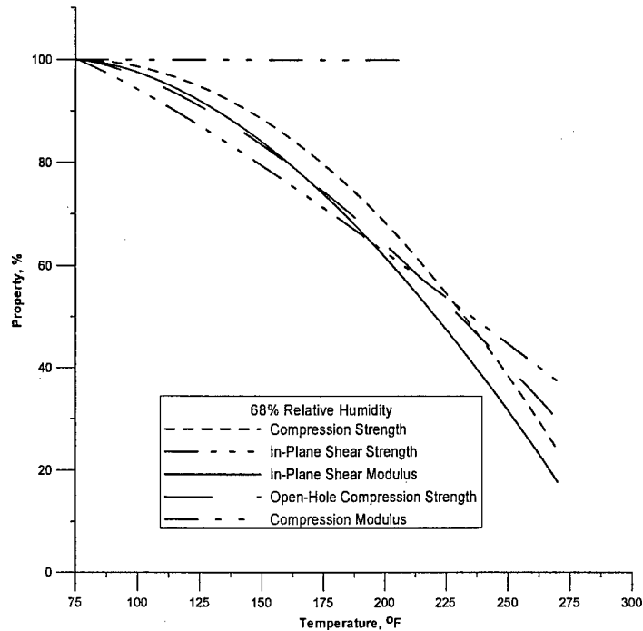
FIGURE 36. VARIATION IN THE PERCENTAGE OF MECHANICAL PROPERTIES AS A FUNCTION OF TEMPERATURE FOR FIBERCOTE E 765/T300 3KPW CARBON FABRIC SPECIMENS CONDITIONED AT 68% RH
