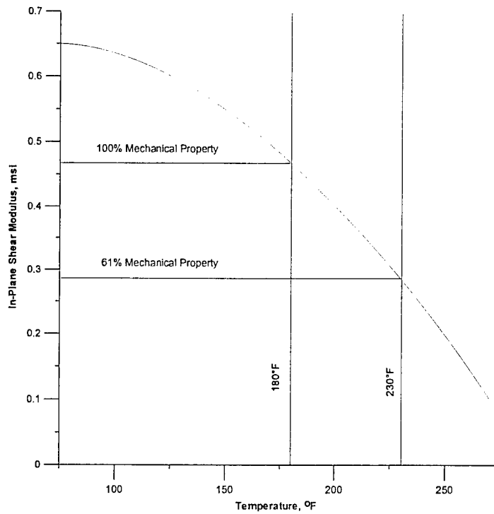
FIGURE 71. TWO-THIRD RETENTION METHOD SHOWN FOR FIBERCOTE E 765/T300 3KPW CARBON FABRIC IN-PLANE SHEAR MODULUS (68% RH)
