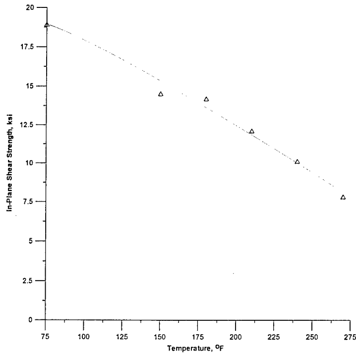
FIGURE 12. VARIATION OF IN-PLANE SHEAR STRENGTH VALUES AS A FUNCTION OF TEMPERATURE FOR NEWPORT 7781/NB321 GLASS FABRIC MATERIAL SYSTEM (68% RH)
