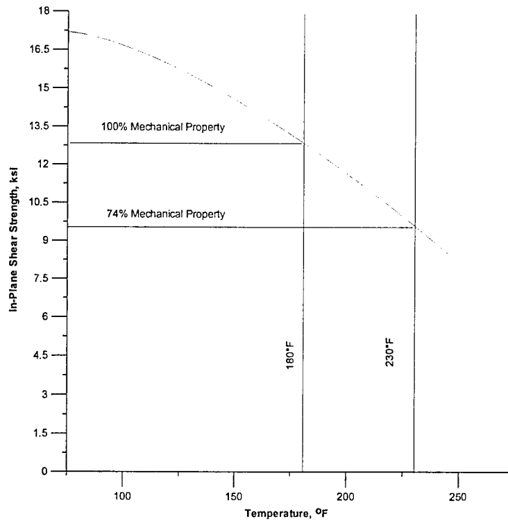
FIGURE 74. TWO-THIRD RETENTION METHOD SHOWN FOR NEWPORT 7781/NB321 GLASS FABRIC IN-PLANE SHEAR STRENGTH (85% RH)
