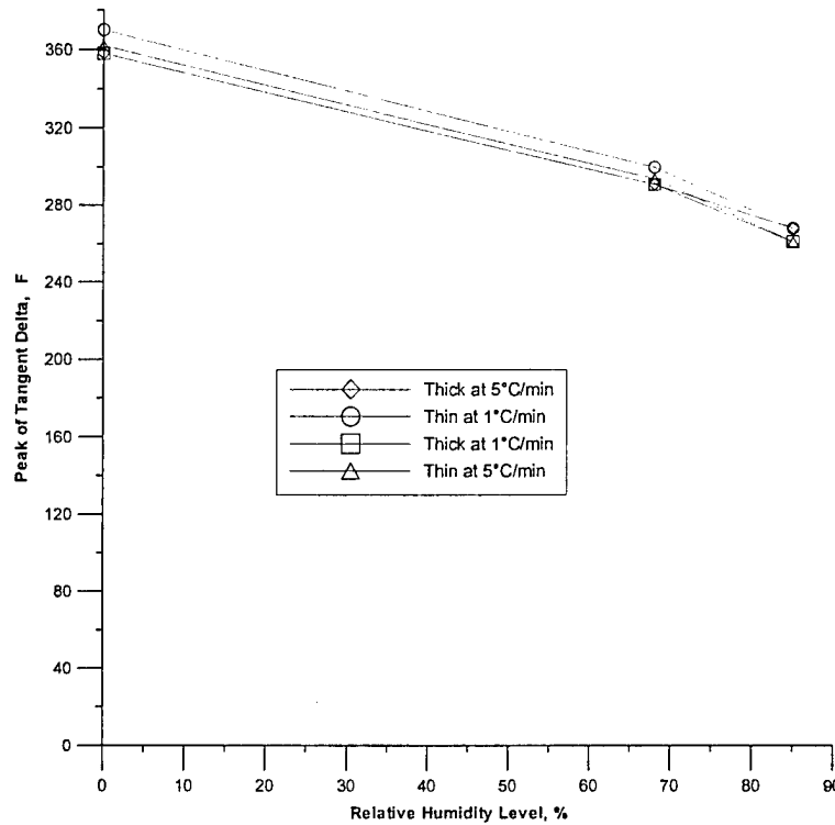
FIGURE 48. VARIATION IN THE PEAK OF TANGENT DELTA VALUES AS A FUNCTION OF RELATIVE HUMIDITY LEVEL FOR NEWPORT 7781/NB321 MATERIAL SYSTEM
