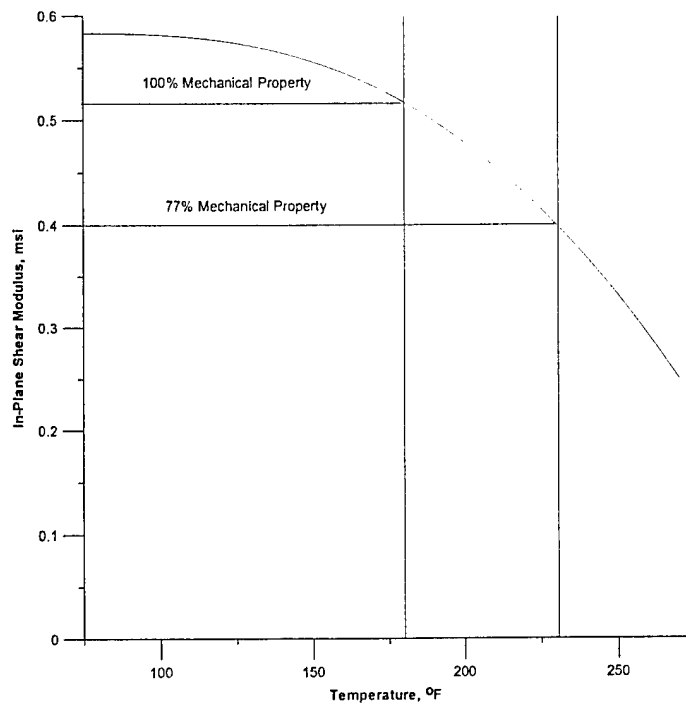
FIGURE 59. TWO-THIRD RETENTION METHOD SHOWN FOR NEWPORT 7781/NB321 GLASS FABRIC IN-PLANE SHEAR MODULUS (0% RH)
