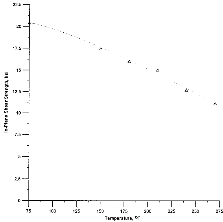
FIGURE 2. VARIATION OF IN-PLANE SHEAR STRENGTH VALUES AS A FUNCTION OF TEMPERATURE FOR NEWPORT 7781/NB321 GLASS FABRIC MATERIAL SYSTEM (0% RH)
