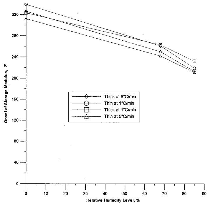
FIGURE 49. VARIATION IN THE ONSET OF STORAGE MODULUS VALUES AS A FUNCTION OF RELATIVE HUMIDITY LEVEL FOR NEWPORT 7781/NB321 MATERIAL SYSTEM
