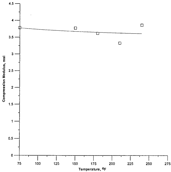
FIGURE 26. VARIATION OF COMPRESSION MODULUS VALUES AS A FUNCTION OF TEMPERATURE FOR NEWPORT 7781/NB321 GLASS FABRIC MATERIAL SYSTEM (85% RH)
