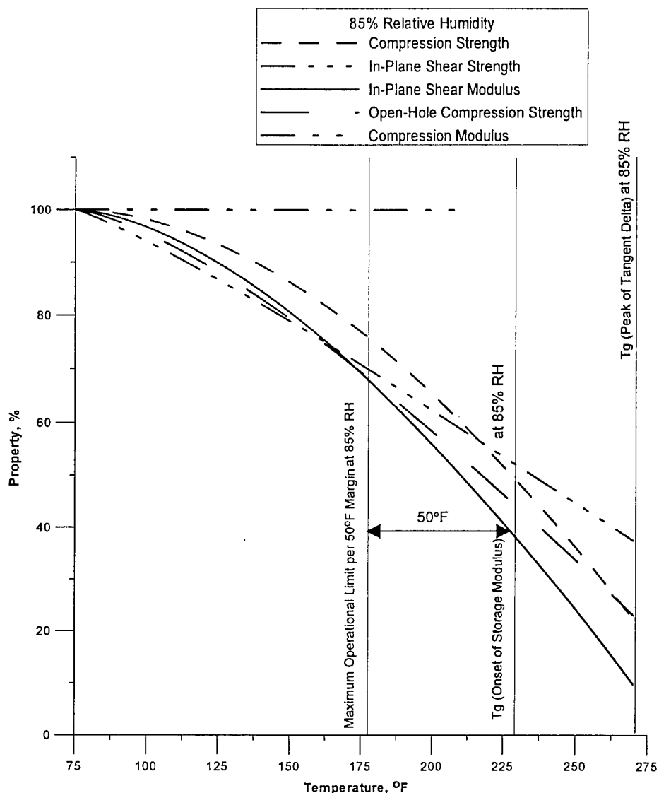
FIGURE 57. MATERIAL OPERATIONAL LIMIT AS PREDICTED BY THE 50°F MARGIN BASED ON THE RESULTS FOR FIBERCOTE E 765/T300 3KPW CARBON FABRIC SPECIMENS CONDITIONED AT 85% RH
