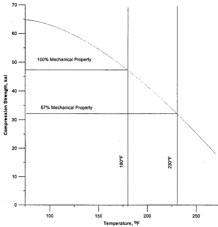
FIGURE 76. TWO-THIRD RETENTION METHOD SHOWN FOR NEWPORT 7781/NB321 GLASS FABRIC COMPRESSION STRENGTH (85% RH)
