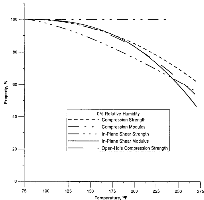
FIGURE 35. VARIATION IN THE PERCENTAGE OF MECHANICAL PROPERTIES AS A FUNCTION OF TEMPERATURE FOR FIBERCOTE E 765/T300 3KPW CARBON FABRIC SPECIMENS CONDITIONED AT 0% RH
