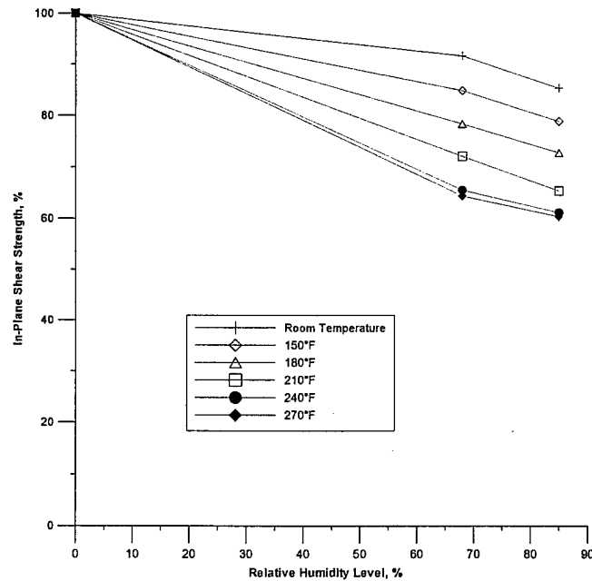
FIGURE 43. VARIATION IN THE PERCENTAGE OF IN-PLANE SHEAR STRENGTH VALUES AS A FUNCTION OF RELATIVE HUMIDITY LEVEL FOR THE SIX TEMPERATURES CONSIDERED FOR FIBERCOTE E 765/T300 3KPW MATERIAL SYSTEM
