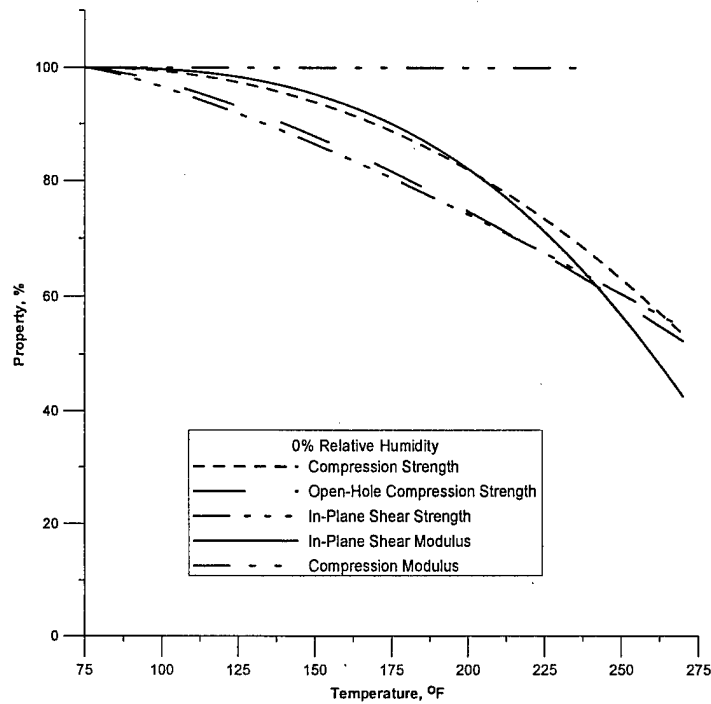
FIGURE 32. VARIATION IN THE PERCENTAGE OF MECHANICAL PROPERTIES AS A FUNCTION OF TEMPERATURE FOR NEWPORT 7781/NB321 GLASS FABRIC DRY SPECIMENS
