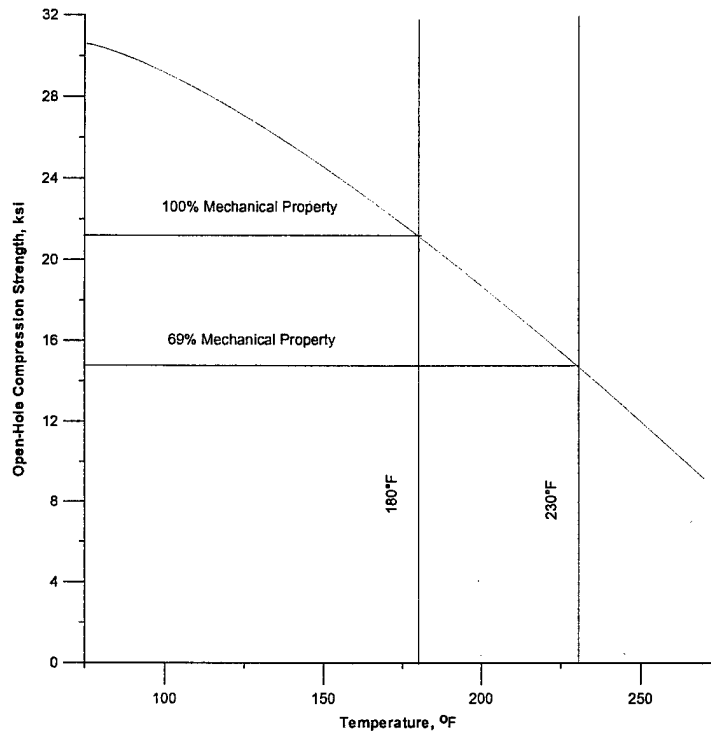
FIGURE 69. TWO-THIRD RETENTION METHOD SHOWN FOR NEWPORT 7781/NB321 GLASS FABRIC OPEN-HOLE COMPRESSION STRENGTH (68% RH)
