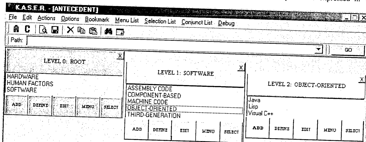
Fig. 1 A Hierarchical Sequence of Object Menus for Software Retrieval
