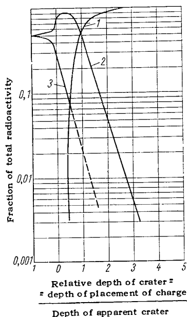
Figure 43. Distribution of radioactivity in a nuclear shot, as a function of the relative depth of the crater:
