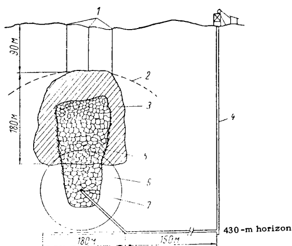
Figure 50. Fragmentation of ore by a nuclear explosion for subsequent underground leaching:
