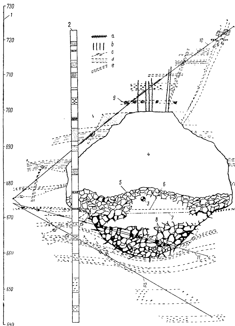
Figure 77. Vertical section of the Gnome explosion cavity: 1 -- elevation above sea level, m; 2 -- position of stratum before explosion; 3 -- center of explosion; 4 -- free space of the cavity; 5 -- pile of fragmented rock; 6 -- level of the water fed into the cavity through wells drilled from the surface; 7 -- approximate upper boundary of hardened fused salt; 8 -- distribution of hardened fused salt in well B; 9 -- strata exposed at the roof of the cavity (see Figure 78); 10 -- well A; 11 -- well B; 12 -- well C; a -- salt changed under the effect of the radiation and observed in the wells; b -- slightly radioactive hardened fused salt, forced into fractures; c -- displacement of strata; d -- contact of bedding planes; e -- zones of fractures.
