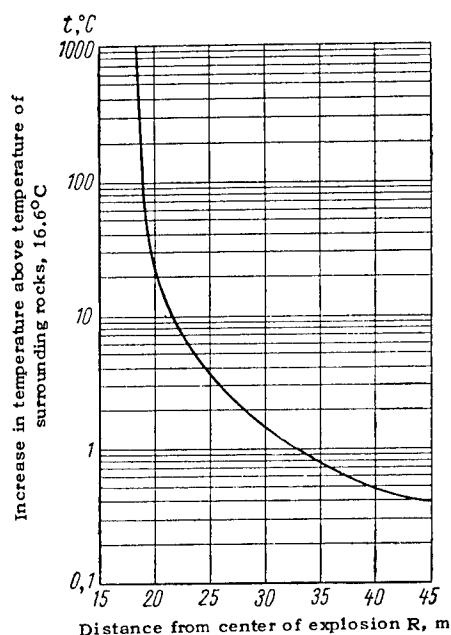
Figure 22. Initial temperature distribution in the Rainier shot.
