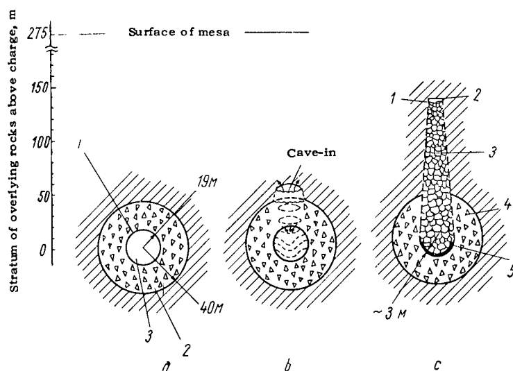
Figure 23. Development of the cave-in of the cavity in the Rainier shot:
