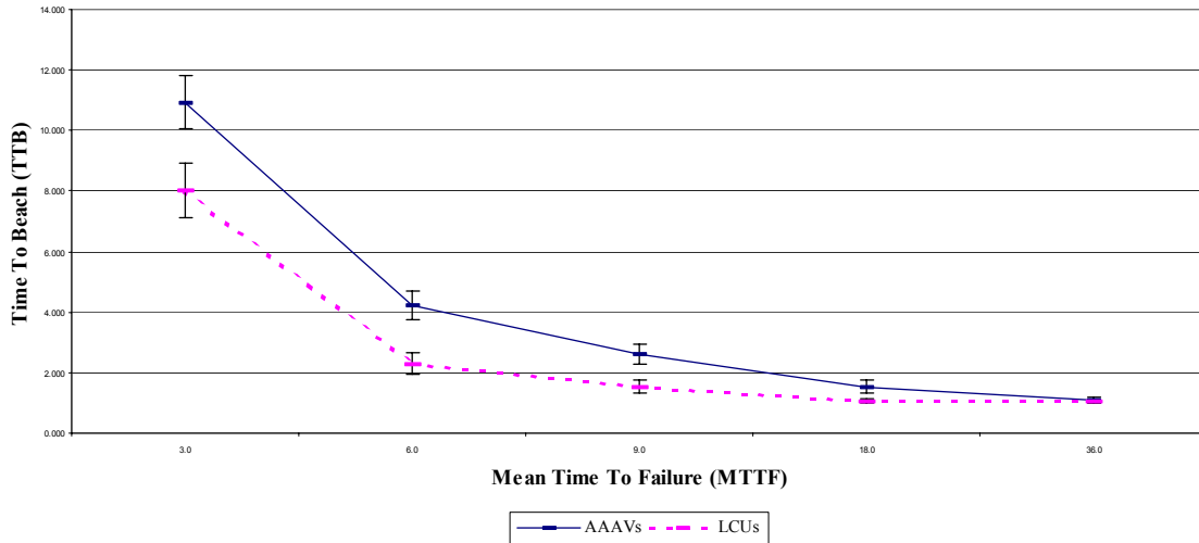
Figure 5. Comparison of Times for At Least 10 of 12 AAVs to Reach the Beach At Various MTF When Different Tow Methods are Used (Failure Times are from the Exponential Distribution).
