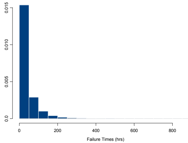
Figure 16. Distribution of Failure Times Generated from a Weibull Distribution with MTTF = 36 and Parameter Settings \kappa = 0.74 and \lambda = 30.0 .
