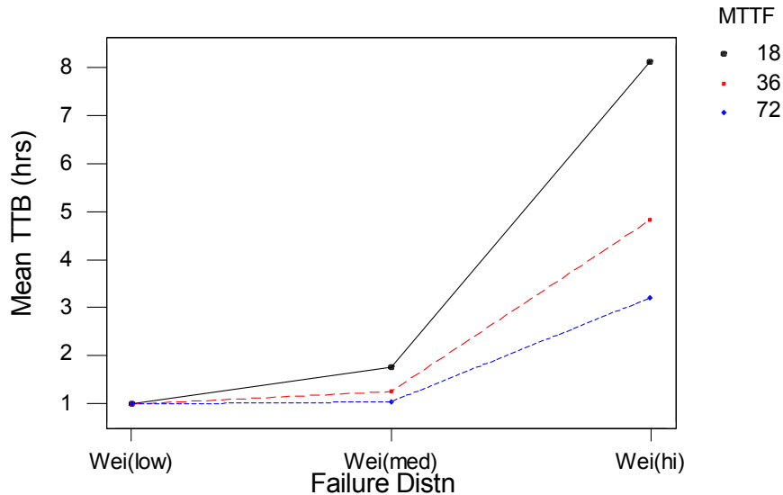
Figure 22. Plot of the Interaction Between the Factors MTTF and Failure Distribution Where the Response Variable is the Times for 12 AAVs to Reach the Beach (TTB).
