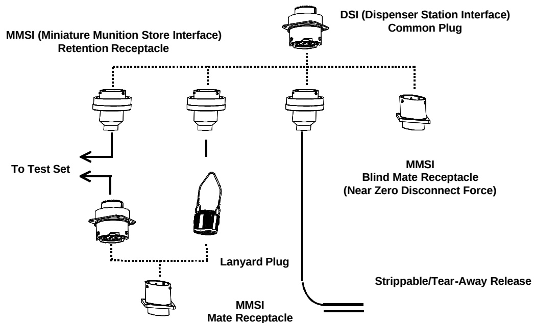
Figure 7. Notional Miniature Store Interface Connector Family
