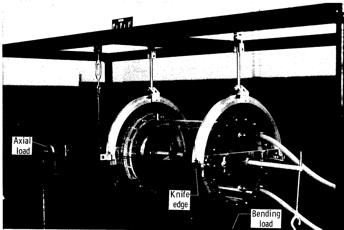
Figure 3. - Details of test setup.
