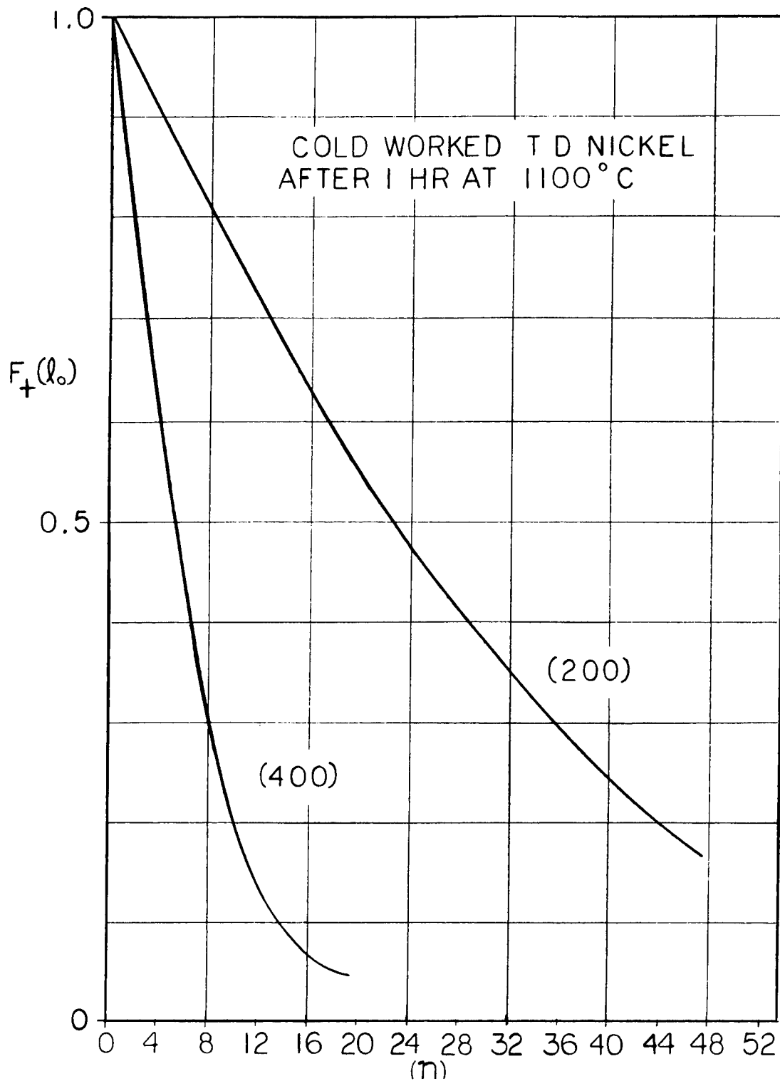
Figure 20. The Fourier coefficients for the 200 and 400 x-ray diffraction lines for TD nickel which has been cold worked and then annealed at 1100°C for 1 hour
