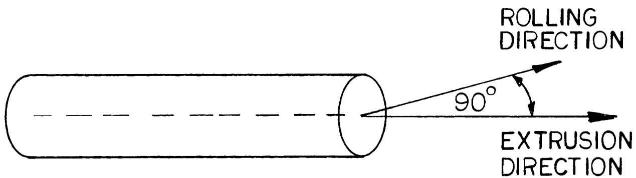
Figure 2. The rolling direction used in the preparation of electron microscopical and x-ray specimens
