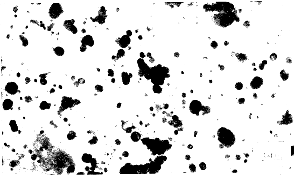
Figure 11. TD nickel. Cold worked and then annealed for 1 hour at 1100°C
