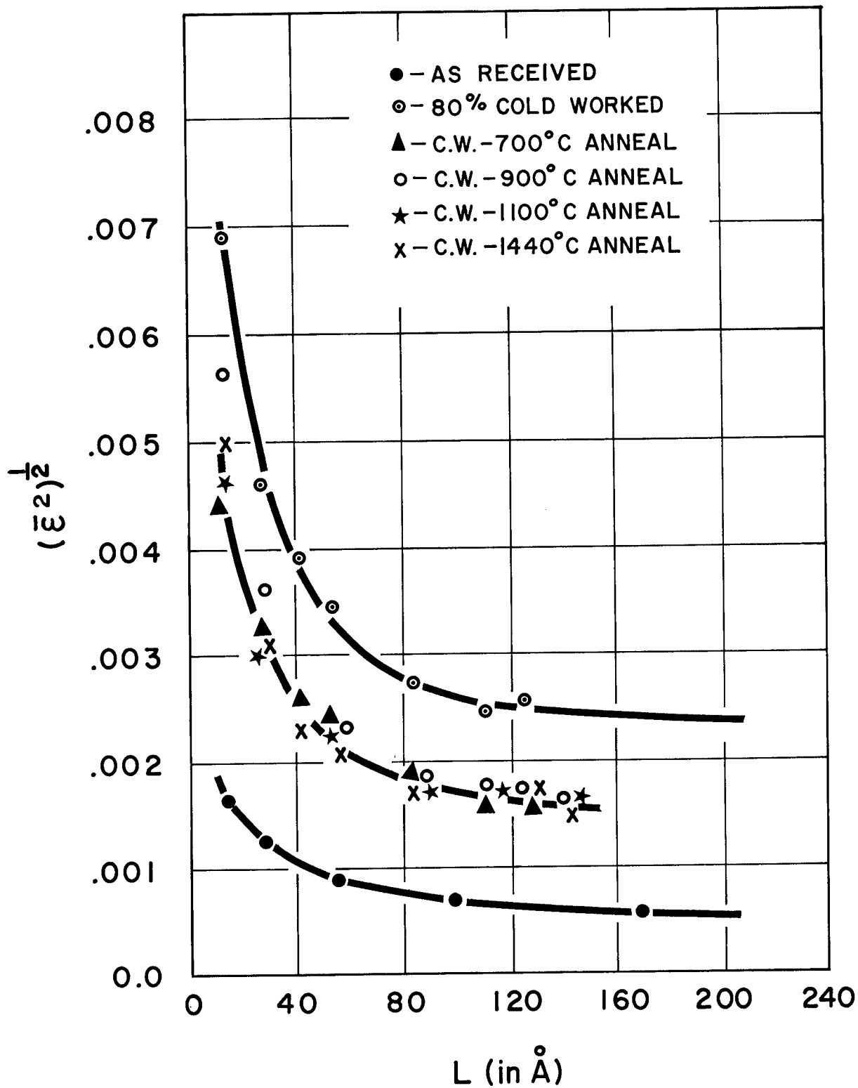
Figure 27. The effect of various heat treatments on the NiB elastic strains in TD nickel
