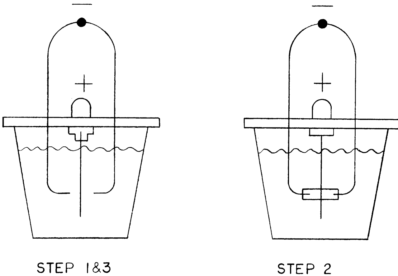
Figure 1. The electrode positions used in the preparation of thin foils
