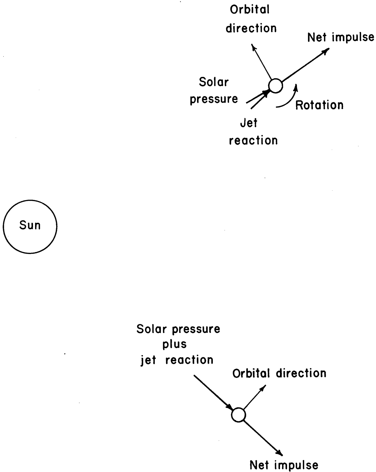
Figure 2.- The jet effect on cometary particle scattering.
