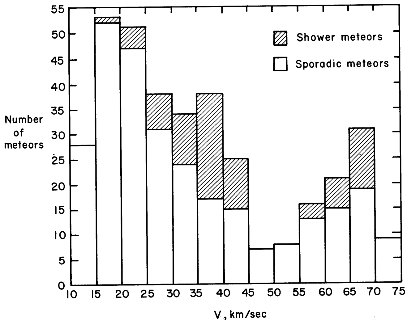
Figure 6.- Distribution of corrected velocities for 285 sporadic and 74 shower meteors. From reference 21.
