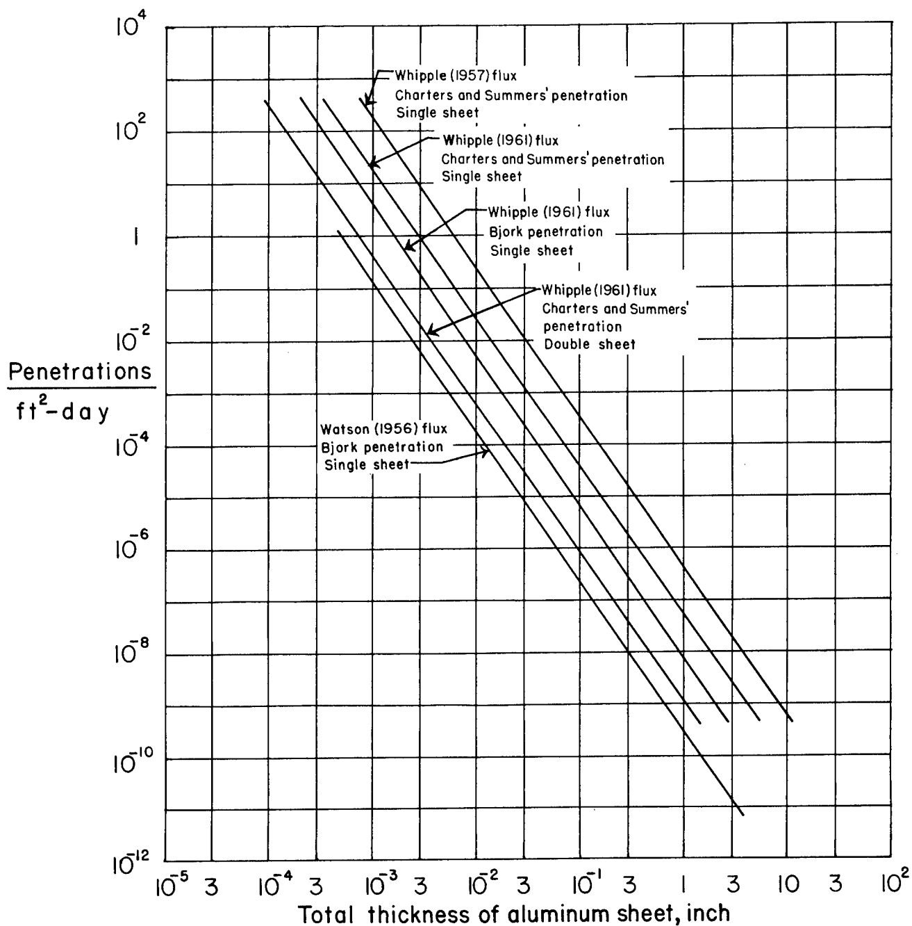
Figure 10.- Most probable rate of puncture as a function of total aluminum skin thickness as determined by various methods. For the purpose of comparison a meteoroid density of 2.7 \text{ g/cm}^3 was assumed in all cases.
