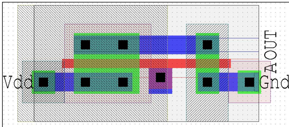
Figure 69. Inverter for ALU GP.
