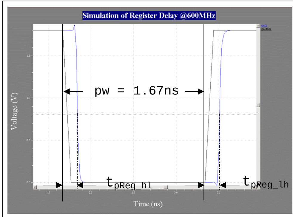
Figure 1. Simulation of Register Propagation Delay.
