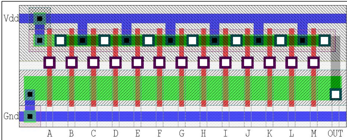
Figure 83. 13-Input NAND.
