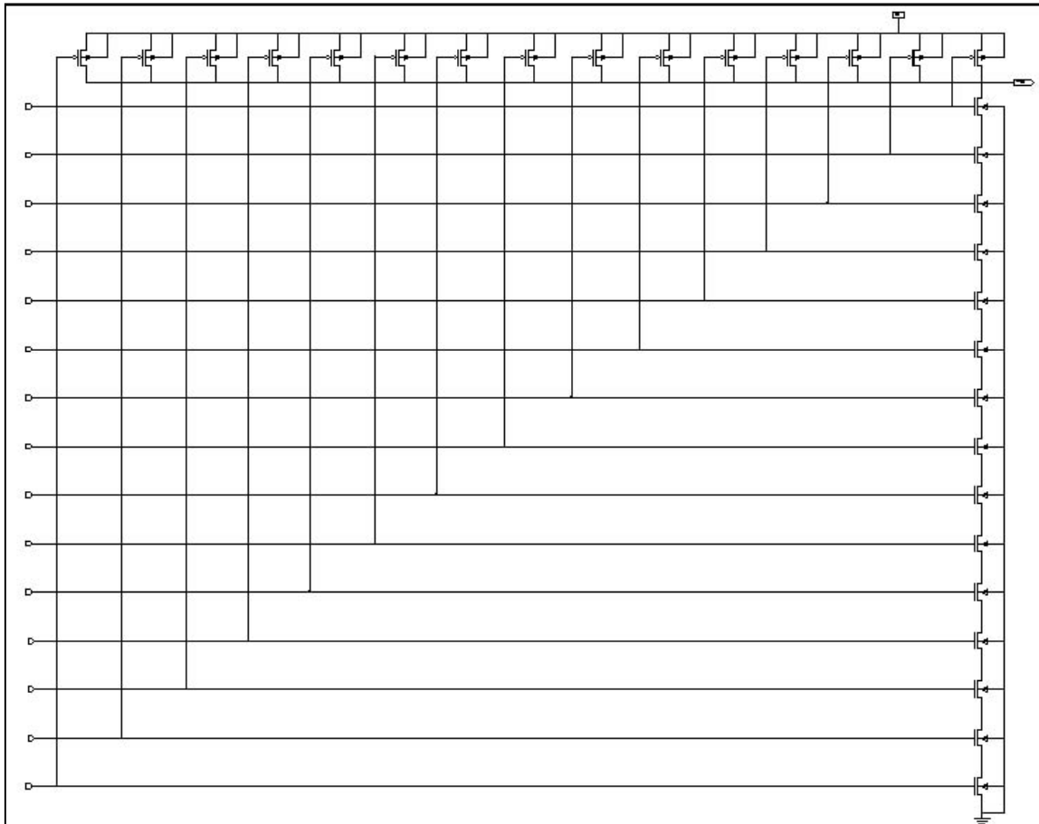
Figure 55. 15-Input NAND.
