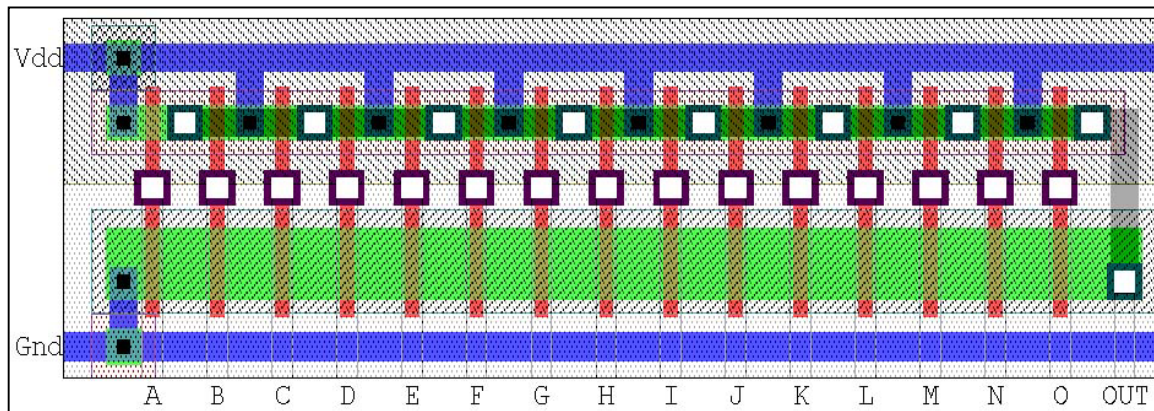
Figure 84. 15-Input NAND.
