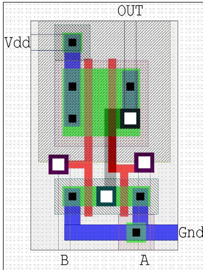
Figure 85. 2-Input NOR.
