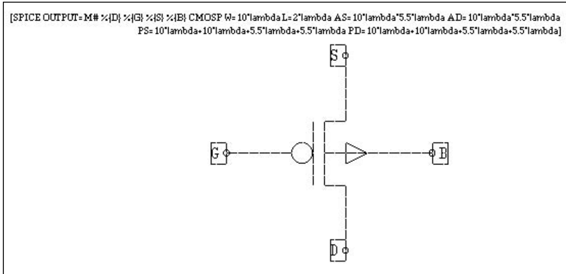
Figure 43. PFET L = 2 lambda, W = 10 lambda.
