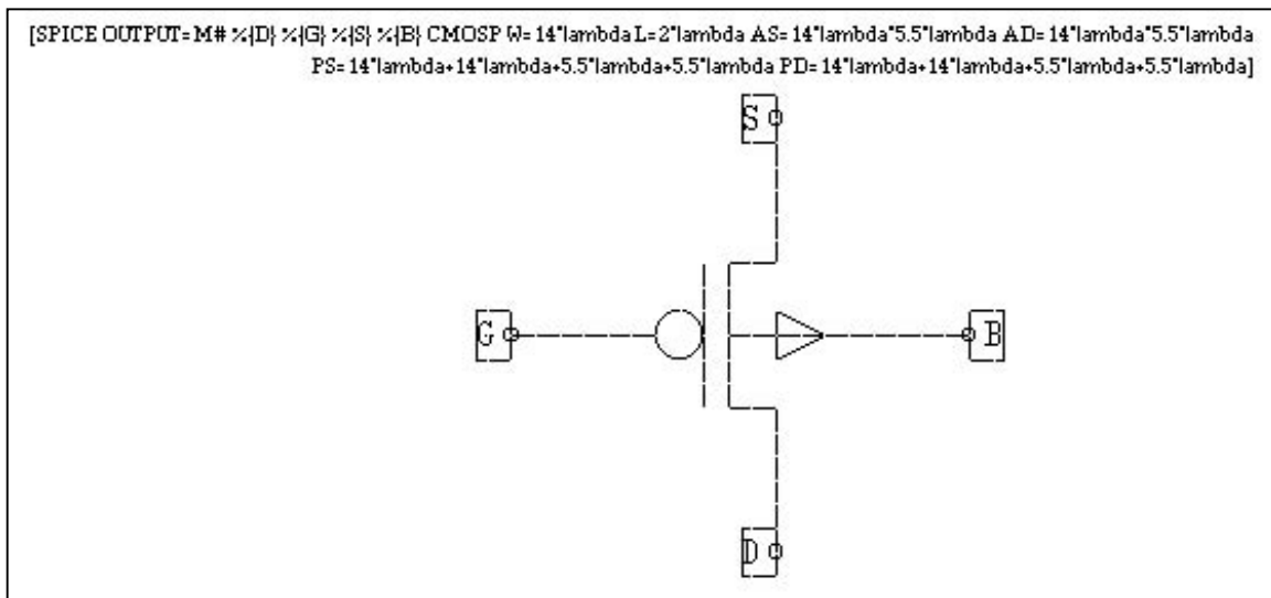
Figure 44. PFET L = 2 lambda, W = 14 lambda.
