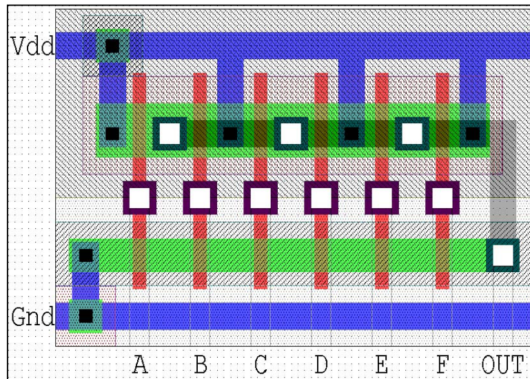
Figure 79. 6-Input NAND.
