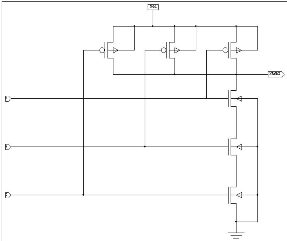
Figure 48. 3-Input NAND.
