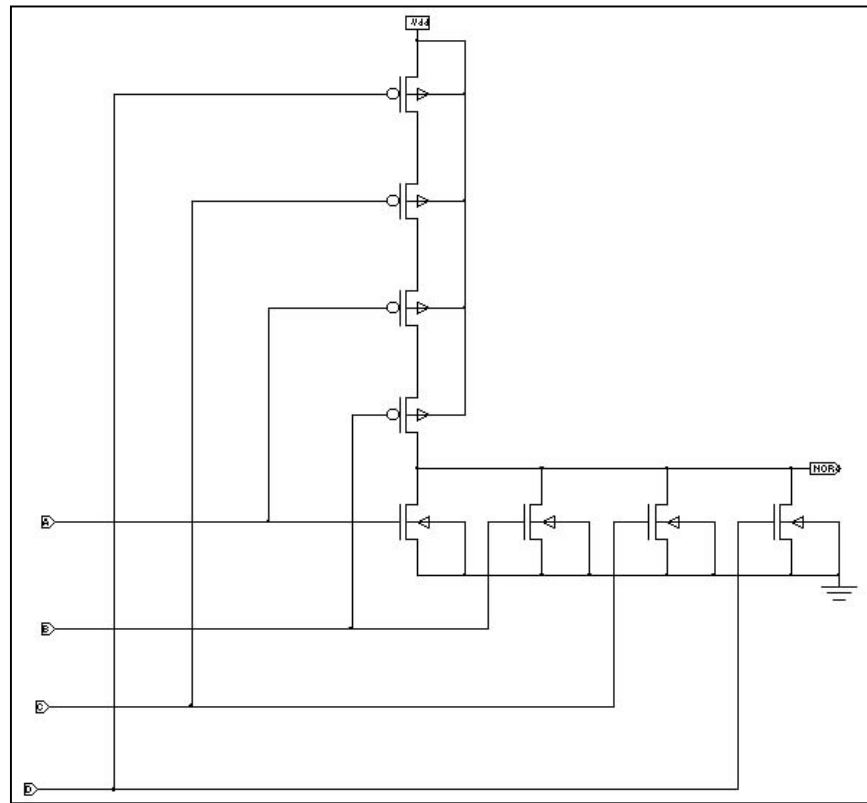
Figure 57. 4-Input NOR.
