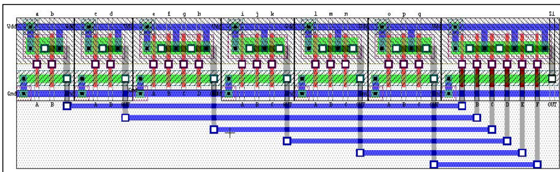
Figure 89. S1 Circuit.
