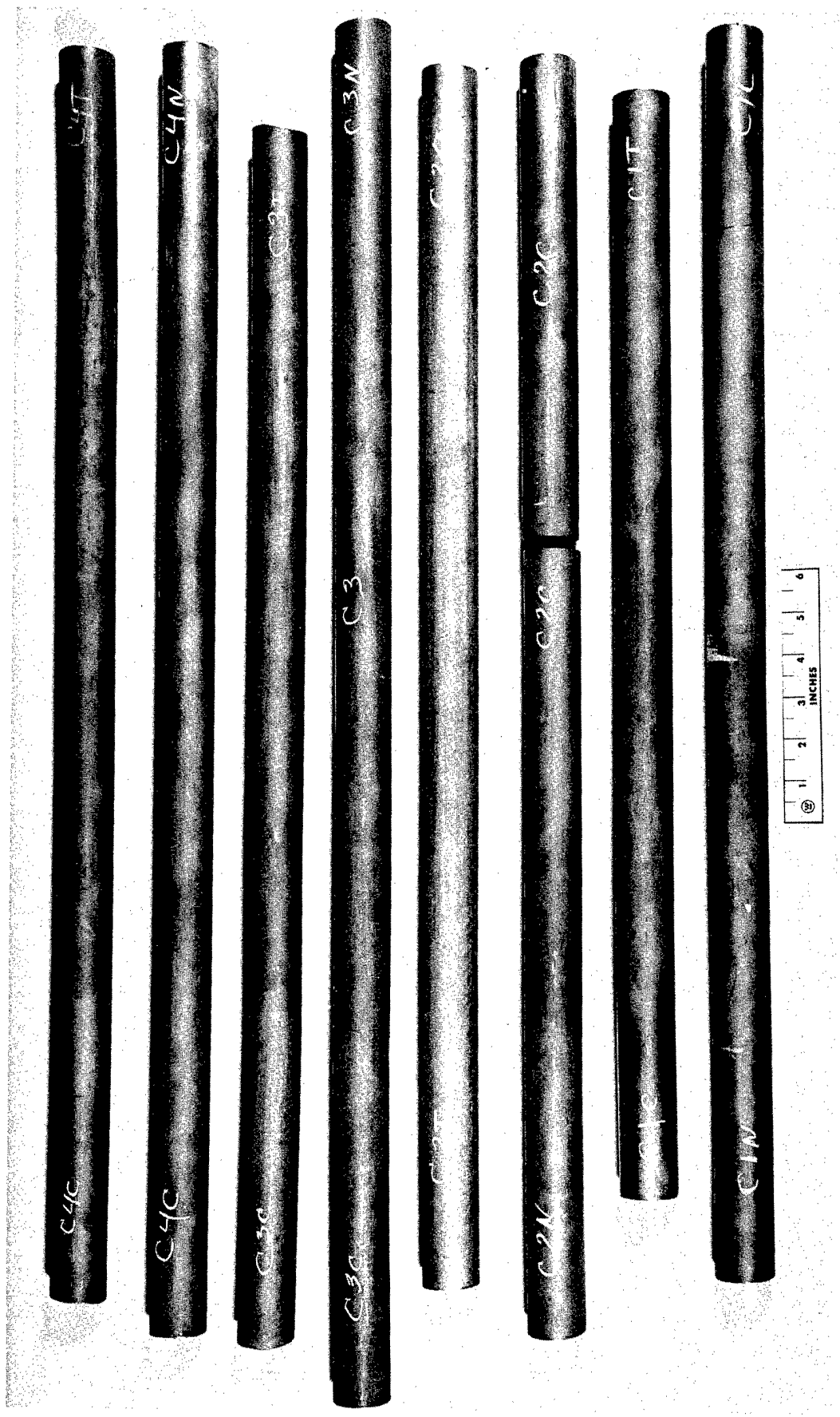
Figure 16 - B-66 Tube Blanks After First Tube Reducing Pass
