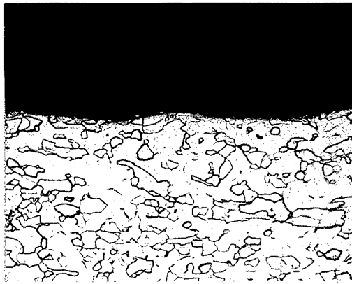
a. I.D. of B-66-II-1, 200X
