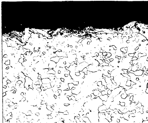
c. B-66-2 Nose, 150X
