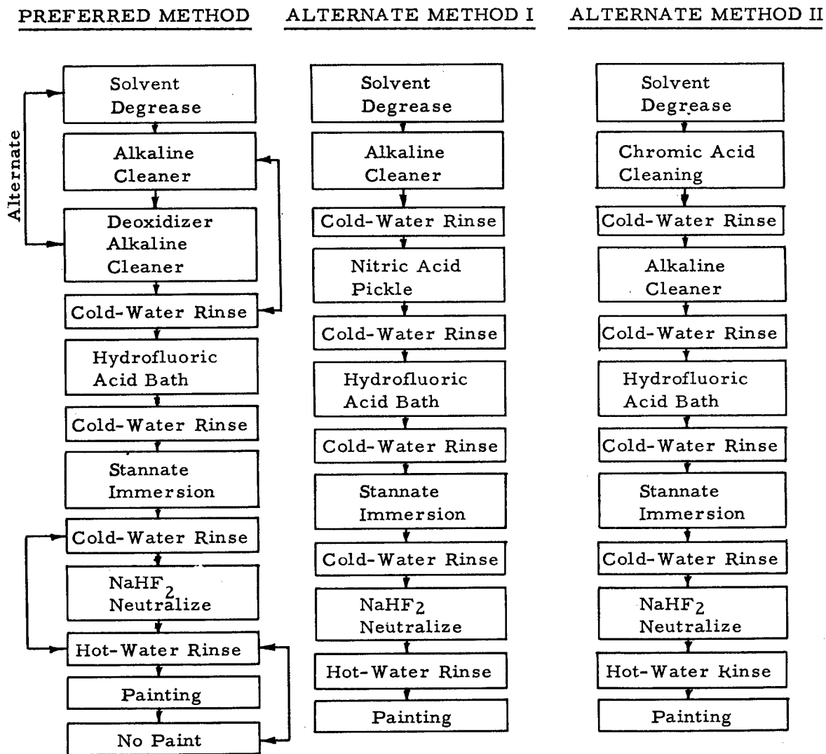
FIGURE A-9. PROCEDURES FOR APPLYING STANNATE COATING(13)
