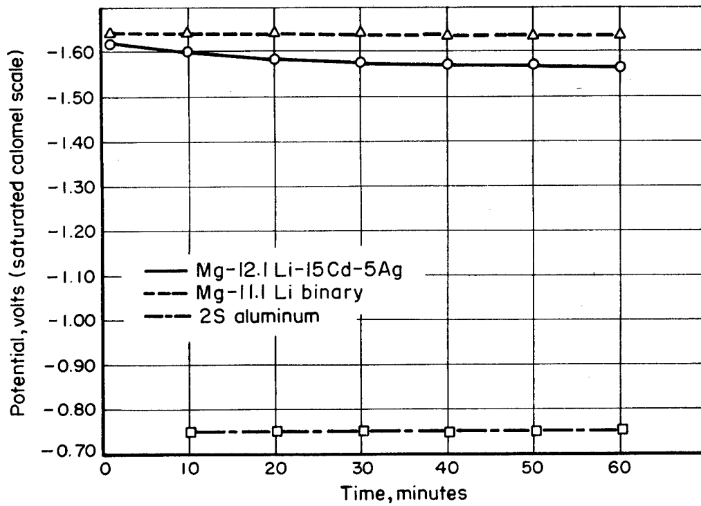
FIGURE A-4. TIME-POTENTIAL VALUES FOR MAGNESIUM-LITHIUM ALLOYS COMPARED WITH ALUMINUM
