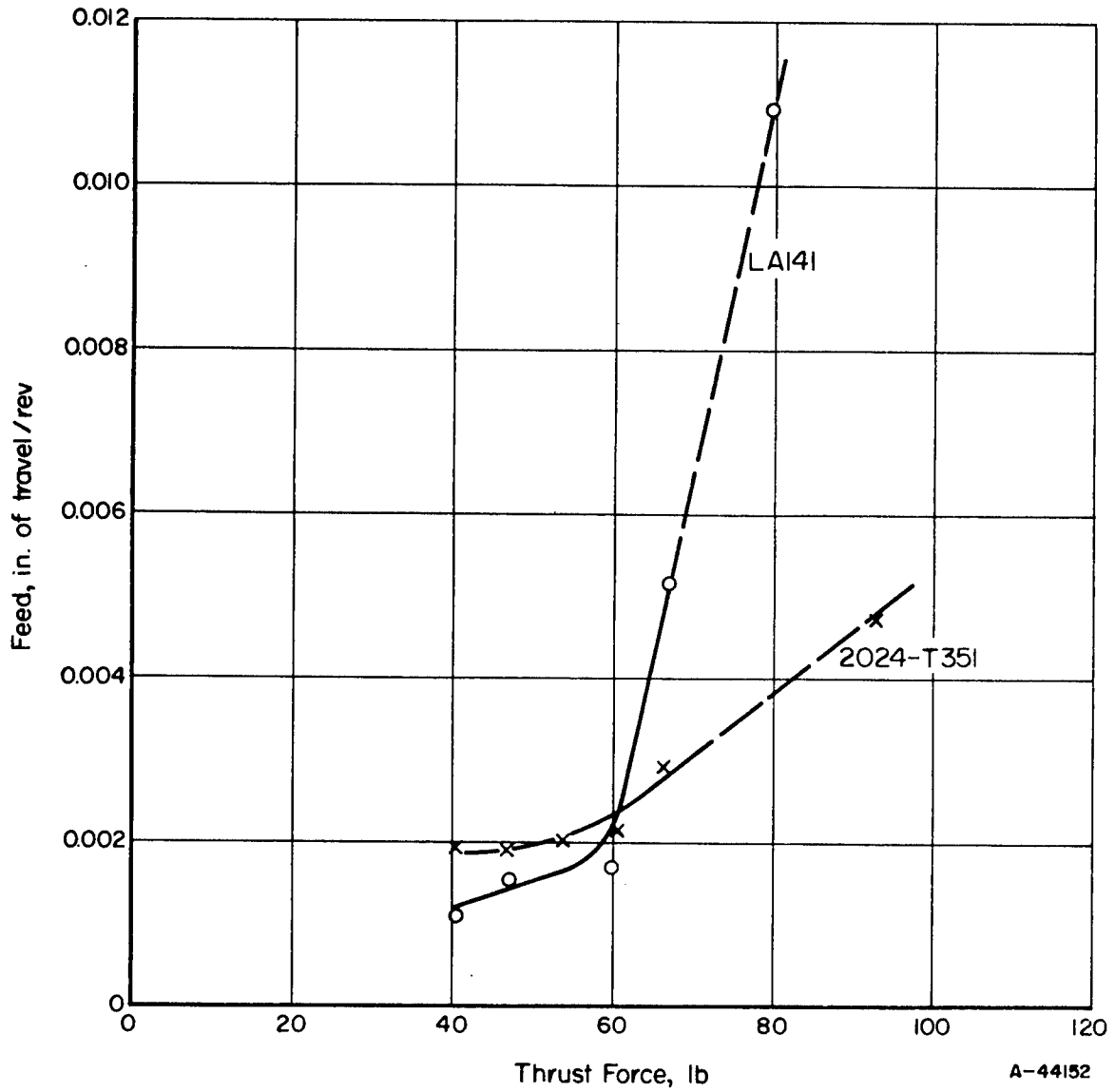
FIGURE 11. EFFECT OF THRUST FORCE ON THE RATE OF FEED FOR LA141 AND 2024 ALUMINUM ALLOY IN CONSTANT-PRESSURE LATHE TEST
