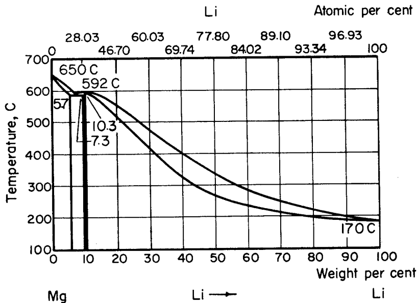
FIGURE A-1. MAGNESIUM-LITHIUM EQUILIBRIUM DIAGRAM (1)
