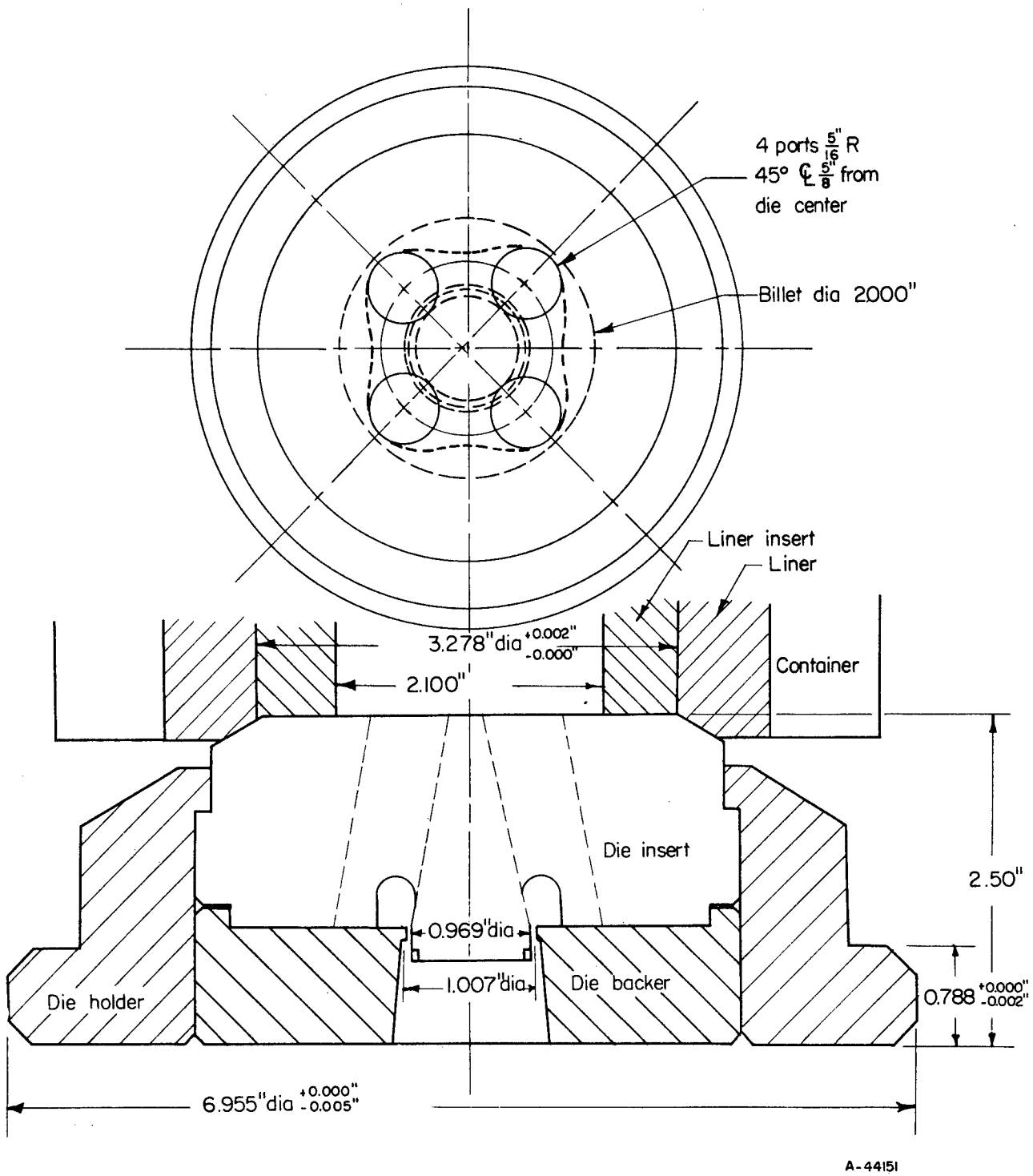
FIGURE 8. DESIGN OF PORTHOLE DIE FOR EXTRUSION OF LA141 TUBING
