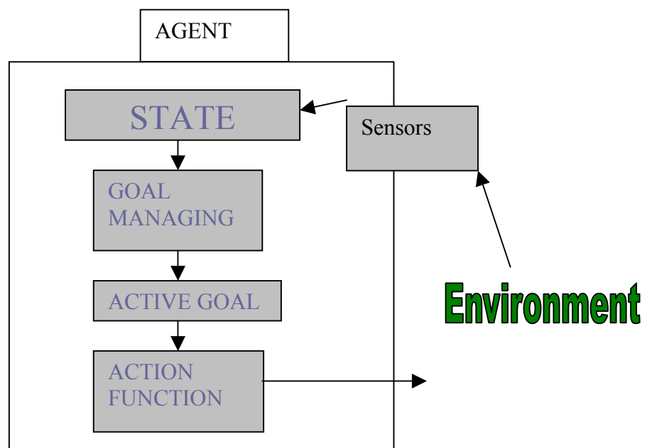
Figure 5. Agent Framework.
