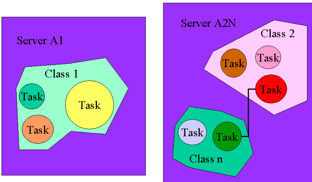
Figure 4: Decomposed Object Servers.
