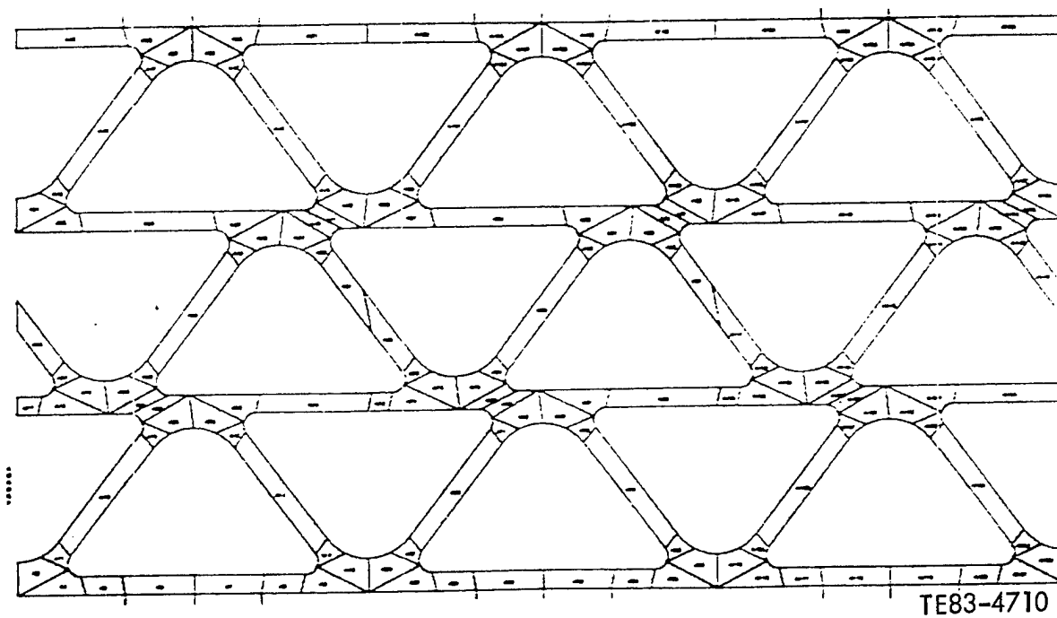
Figure 2-4. Micro Model for Wrapped AS Matrix.
