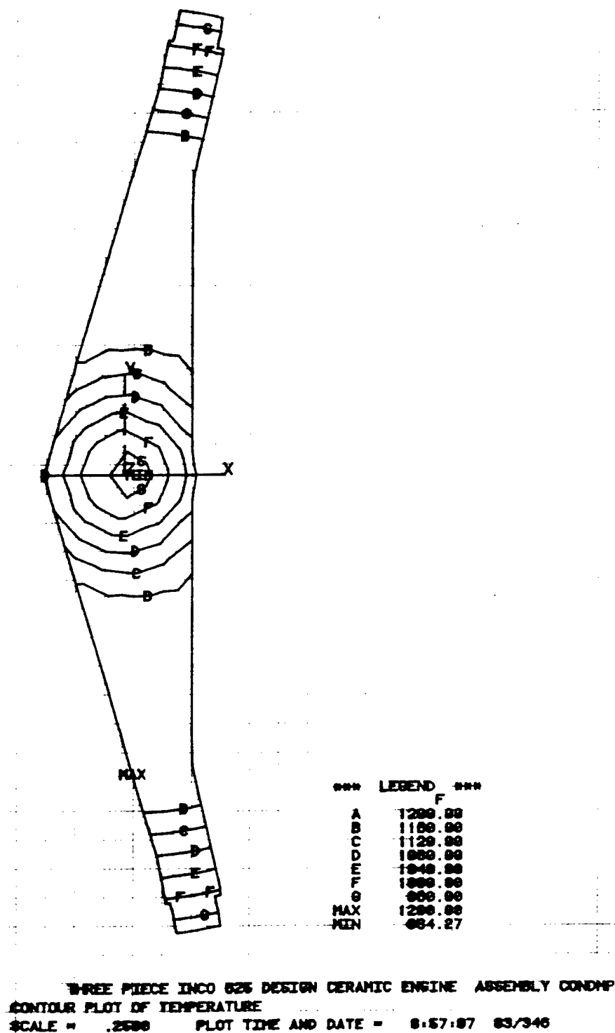
Figure 3-3. Crossarm Temperature--1500 HP Condition
