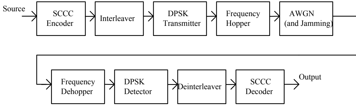
Figure 6.3. SCCC/DPSK simulation model with frequency-hopped spread spectrum.
