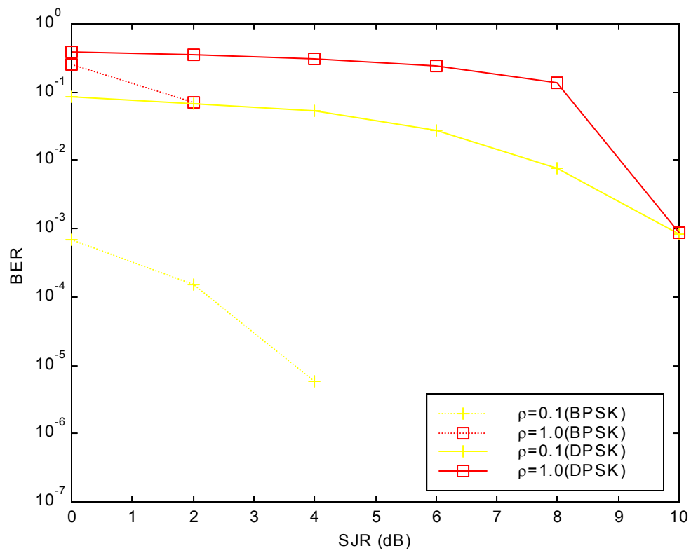
Figure 8.9. Simulated SCCC with AWGN and pulsed noise jamming and side information: effect of BPSK and DPSK modulation on BER for \rho = 0.1 and 1.0 , \text{SNR} = 8 dB and \text{SJR} = 0 to 10 dB.
