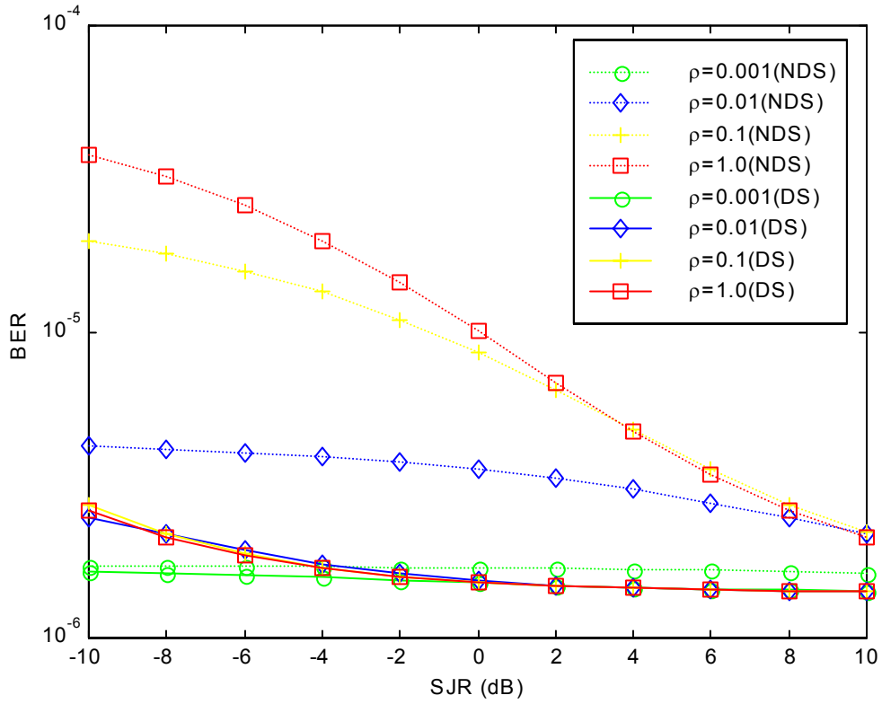
Figure 4.13. Theoretical SCCC/BPSK with AWGN and pulsed noise jamming with no side information: effect of direct sequence spread spectrum on BER for \rho = 0.001, 0.01, 0.1 and 1.0 , SNR = 2 dB and SJR = -10 to 10 dB.
