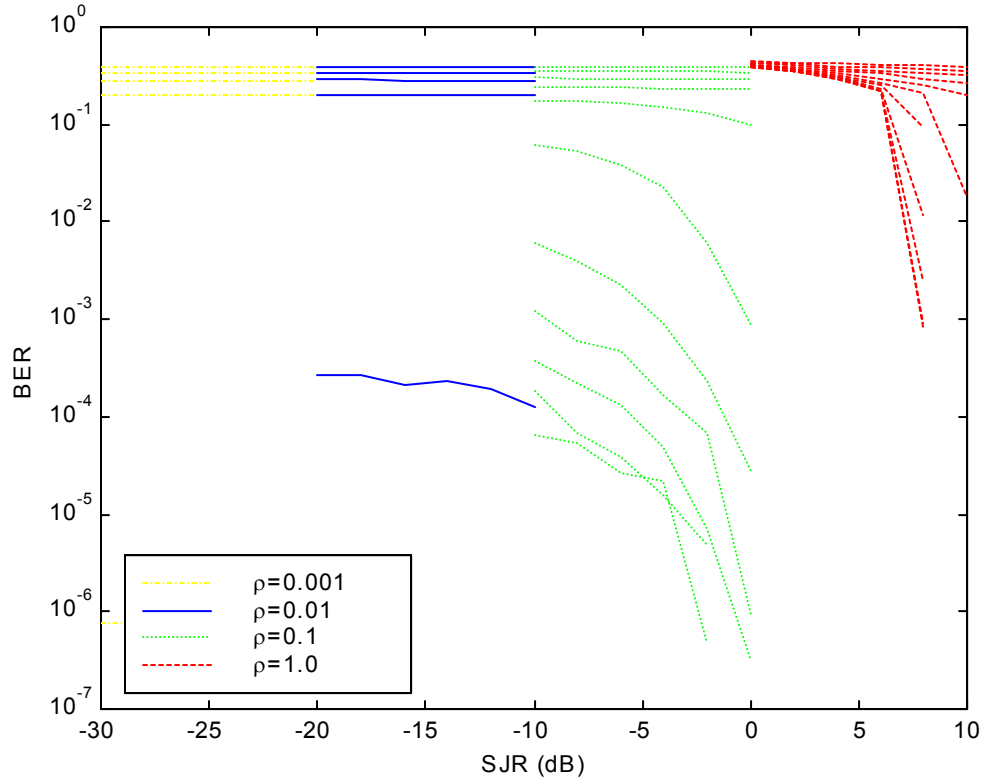
Figure 7.13. Simulated SCCC/DPSK with AWGN, pulsed noise jamming with no side information and Rayleigh fading with no channel information: effect of \rho on BER for \rho = 0.001, 0.01, 0.1 and 1.0 , \text{SNR} = 0 to 20 dB and \text{SJR} = 0 to 10 dB. Note that in order to show the graphs for the different values of \rho , the SJR is offset by \rho in dB. Thus, for \rho = 0.001, 0.01, 0.1 and 1.0 , there are offsets of -30, -20, -10, 0 dB, respectively. The graphs start at 0 dB at the top with increments of 2 dB for each subsequent graph downwards. Note that when there is no graph for a particular SNR, it means that all errors were corrected for that SNR for the range of SJR considered.
