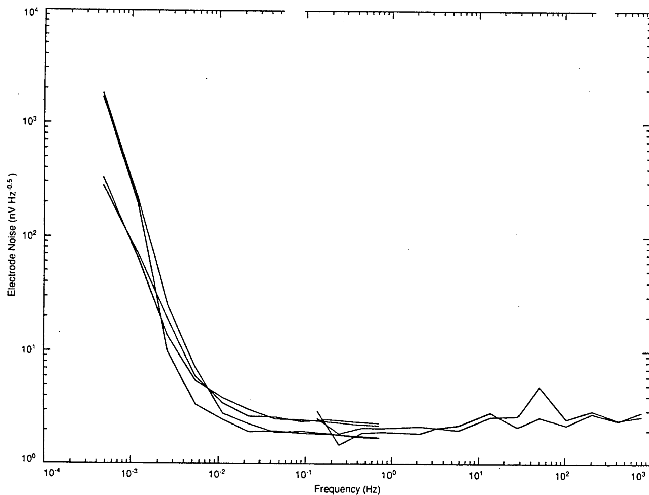
Figure B.1 APL electrode spectra at 4°C. Four electrode pairs were sampled for the spectra below 1 Hz while two were sampled above 1 Hz. The better pairs have about 100 nV/√Hz noise at 1 mHz and reach the instrumentation noise floor of 2 to 3 nV/√Hz at about 30 mHz.
