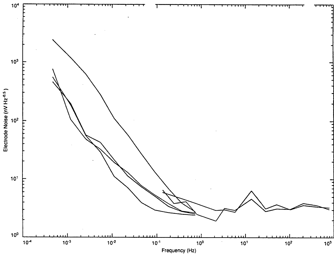
Figure B.8 NSWC electrode spectra at 17–19°C while the bath controller is turned off. The spectral levels are nearly the same as Figure B.6.
