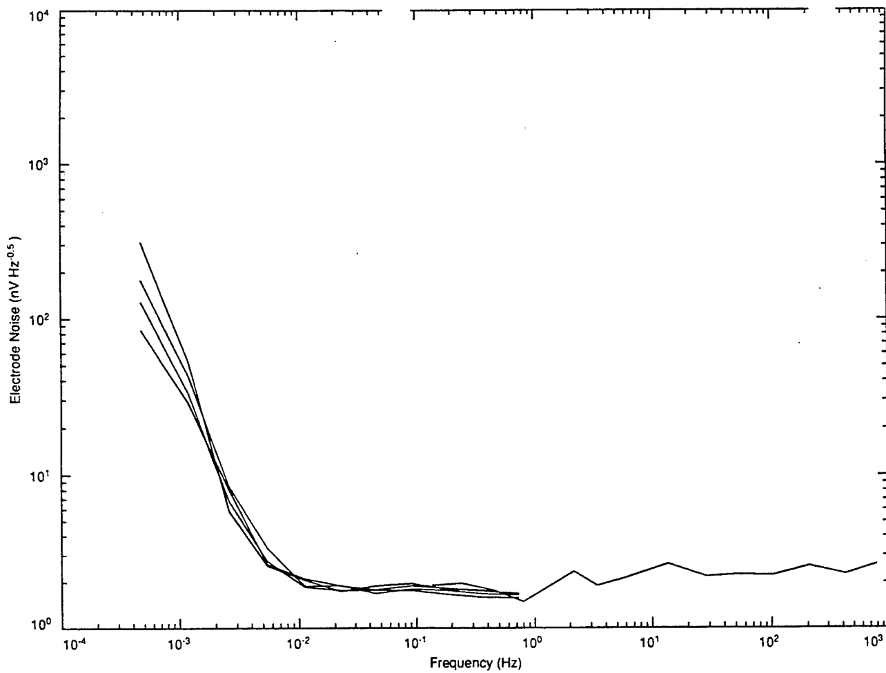
Figure B.11 SAIC electrode spectra at 15°C. The best have 30 \text{ nV}/\sqrt{\text{Hz}} noise at 1 mHz. The noise floor is reached at a slightly lower frequency than Figures B.9 and B.10.
