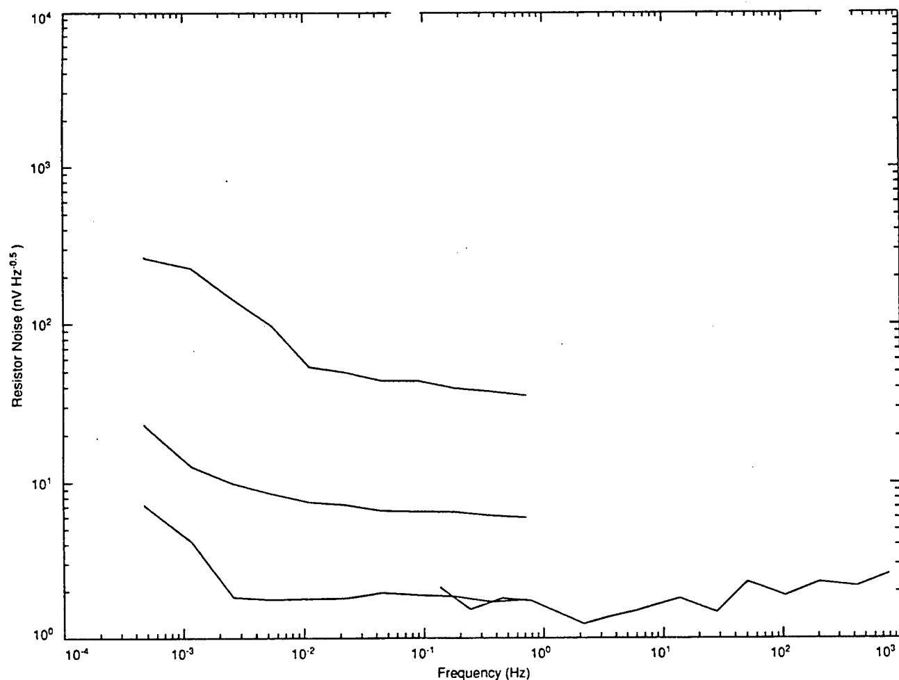
Figure B.13 Resistor spectra at 4°C. The three groups of measured spectra less than 1 Hz correspond to three values of resistance, 10 kΩ, 950 kΩ, and 20 Ω. The single high frequency spectrum is measured with a 20 Ω resistor. These measured spectra have the same noise at all frequencies above 10 mHz and the noise decreases as resistance decreases. We feel that the rise in noise below 10 mHz is due to the thermal noise of the scanner.
