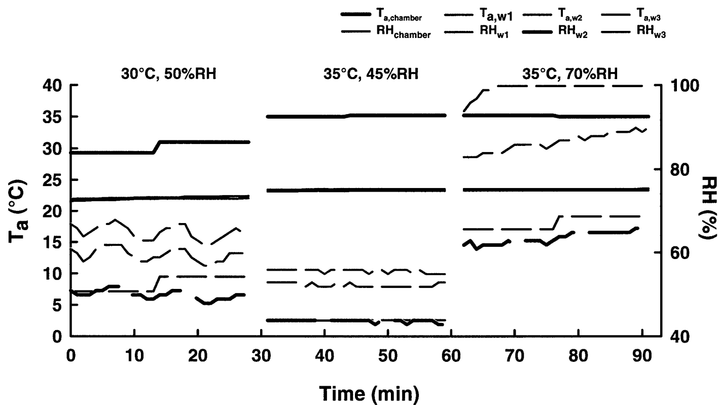
Figure 8. The WAPEM's ambient temperature ( T_a ) and relative humidity (RH) measurements in a climatic chamber (Heller Institute) at T_a of 30°C and 35°C and RH of 50%, 45% and 70%.
