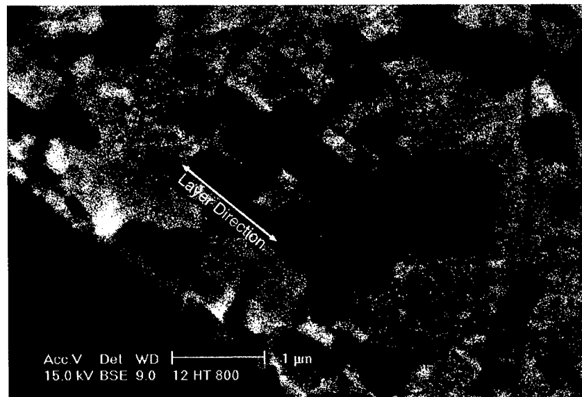
Fig. 6: Morphology of \langle 111 \rangle 20nm/20nm \gamma -Ni(Al)/ \gamma' -Ni 3 Al multilayer after heating to 800C for 101 hours in an Argon atmosphere (#12-7). Note that significant coarsening has occurred, since the particles are several time the initial layer thickness.
