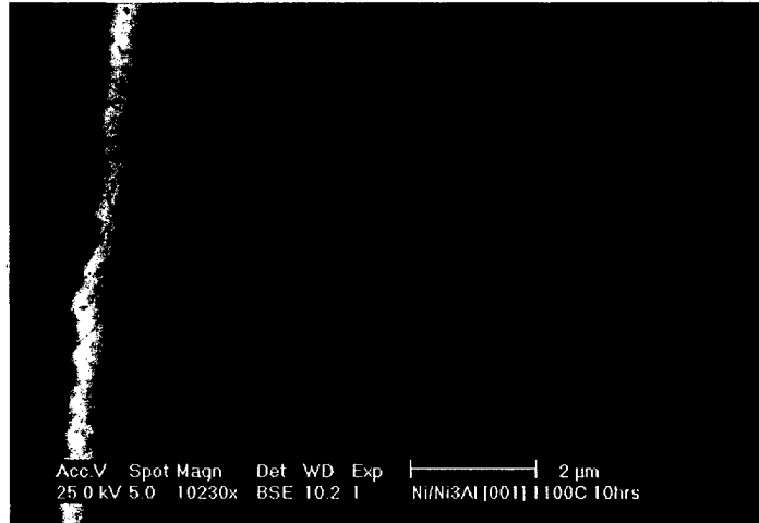
Fig. 12: Observed morphology of a \langle 001 \rangle 120nm/120nm \gamma -Ni(Al)/ \gamma' -Ni 3 Al multilayer after heating to 1100C for 10 hours in an Argon atmosphere, then furnace cooling (from Denman presentation).
