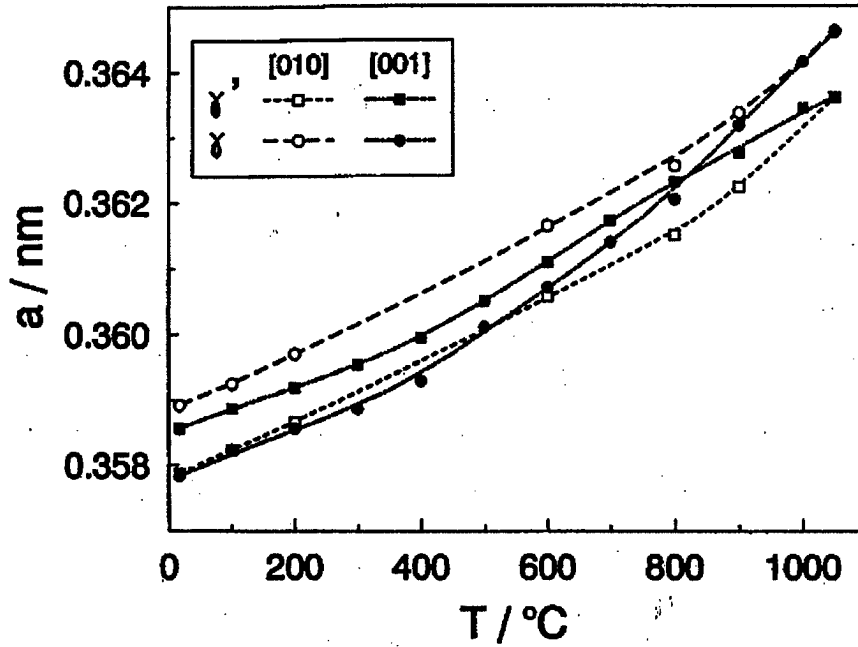
Fig. 17: Stress-free lattice parameters of \gamma \gamma -Ni(Al) and \gamma' -Ni 3 Al phases as a function of temperature [11].
