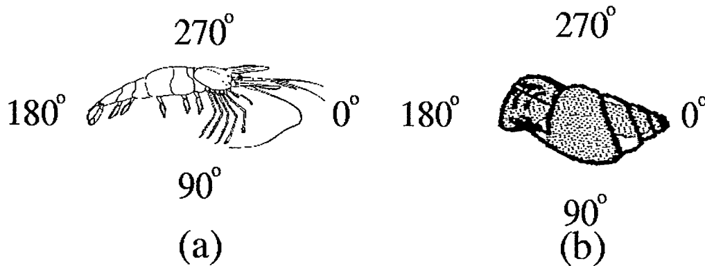
Figure 2-2: Orientation of incident acoustic wave relative to the (a) shrimp and (b) snail. 0° incidence is approximately “head-on” and “apex-on” incidence for the two animals respectively.
