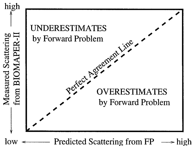
Figure 4-19: Schematic explaining the cause of errors in the plots showing the results of the Forward Problem calculations. If our model and data were perfect, all FP outputs would lie along the diagonal line. If points appear above the diagonal line, then these are “underestimates” of the scattering by the FP calculations. If points lie below the diagonal line, then they are “overestimates”.
