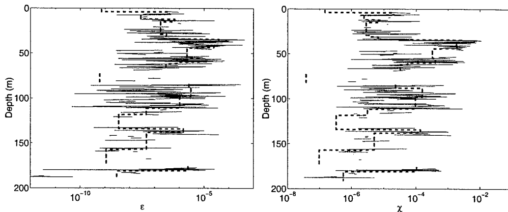
Figure A-16: Calculated values of \epsilon (left) and \chi (right) from hydrographic information from MOCNESS #7 using equations 4.8, 4.9, 4.10, and 4.11. Dashed lines are the mean value for the depth bins selected for the Thorpe length analysis.
