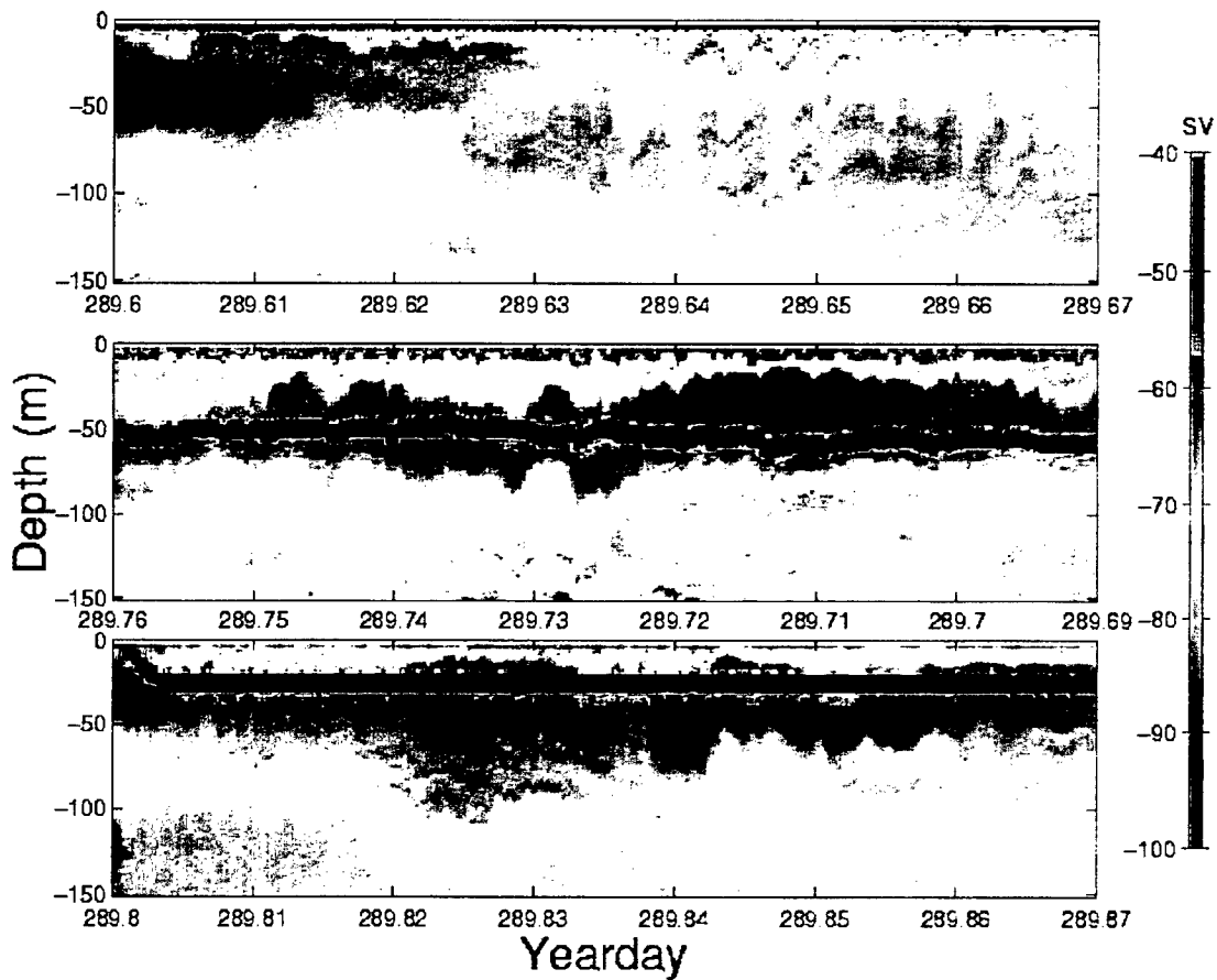
Figure 4-6: The three acoustic transects (120 kHz data shown) through the internal wave field. The first (top), second (middle) and third (bottom) surveys were made consecutively with a 180° turn in the ship between each transect. While a strong internal wave was seen in the first transect, the second and third passes do not show the wave nearly as well. BIOMAPER-II was towed at varying depths (5, 50, and 25 meters respectively) through the internal wave in order to use the VPR data to characterize the different layers, unfortunately the distinct layers were not present during the second and third passes.
