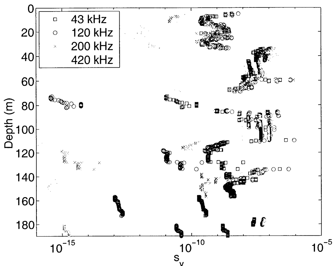
Figure A-17: Predicted levels of volume scattering from Seim's model and the hydrographic information from MOCNESS #7. There is increased scattering from microstructure at the surface and in the regions that appear to be well mixed in the density profile. It should be noted that the largest amount of scattering is not always at the same frequency which suggests that the length scale of the microstructure or turbulence is varying throughout the water column as well. These values of volume scattering are likely to be too large since they would account for all of the scattering that was measured in the water column, this is attributable to our method of estimating \epsilon which is an imperfect assumption.
