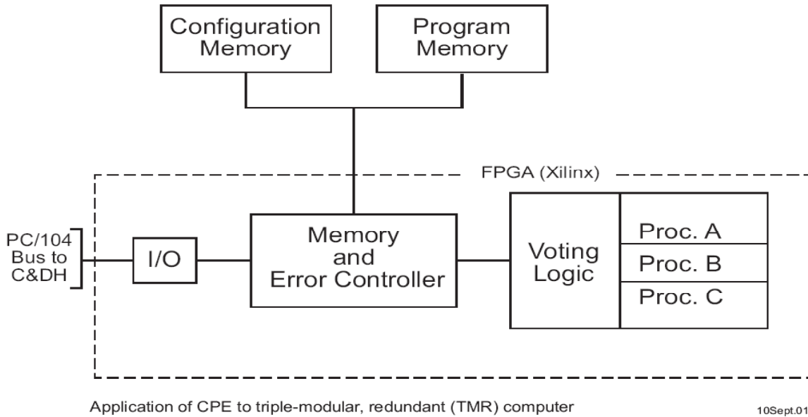
Figure 16. CPE Block Diagram
