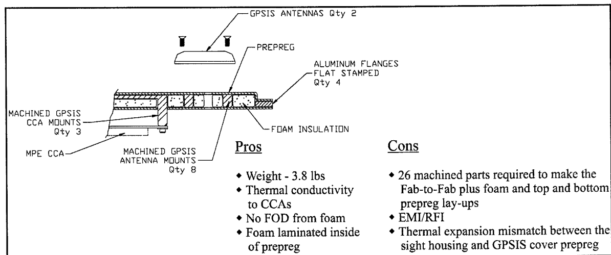
Figure E.7 - Design Option 4
