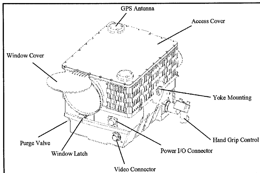
Figure E.1 - Long Range Advanced Scout Surveillance System
