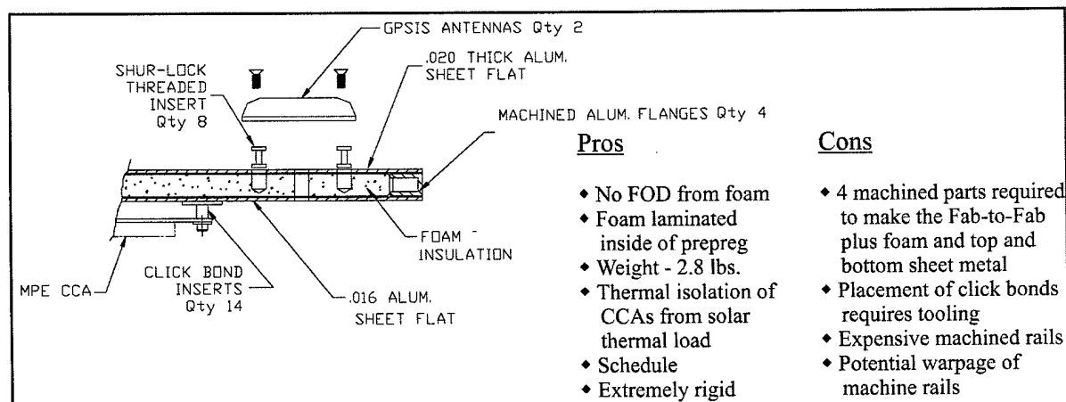
Figure E.9 - Design Option 6
