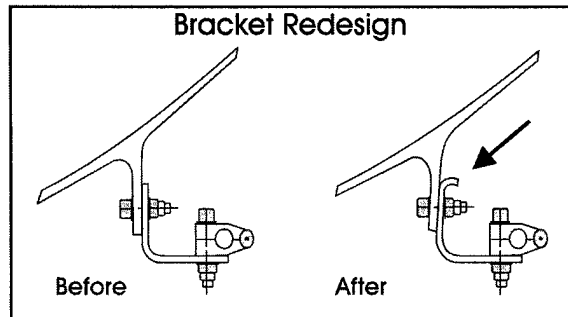
Figure 4.3 - Error-Proofed Bracket Design
