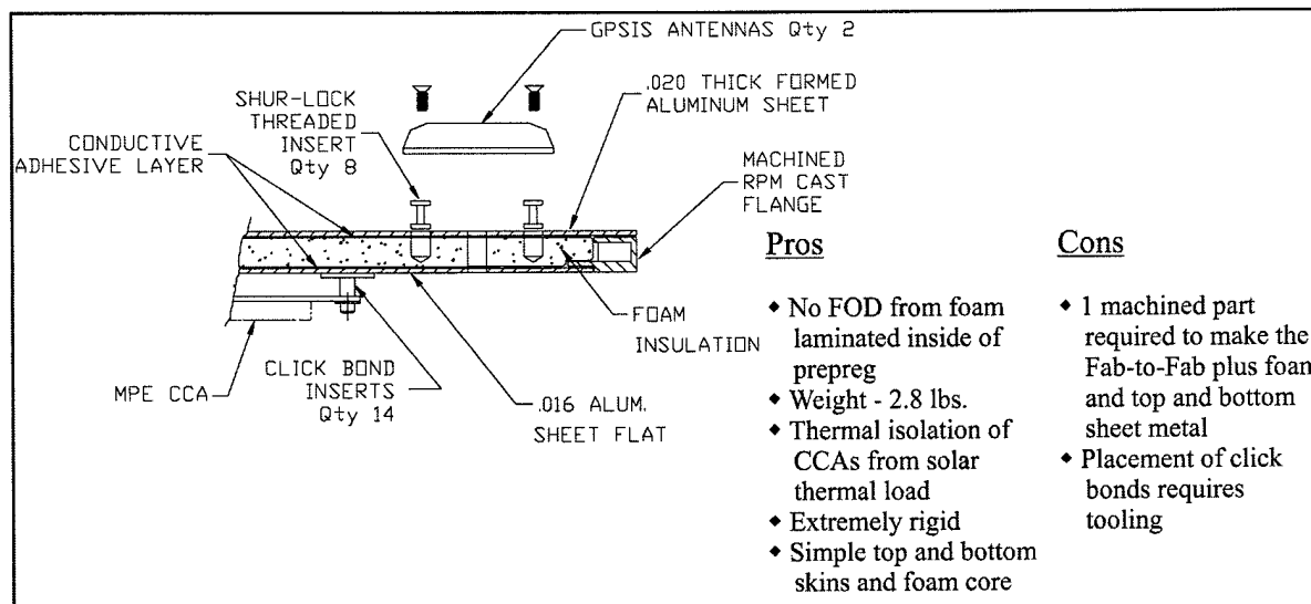
Figure E.10 - Design Option 7
