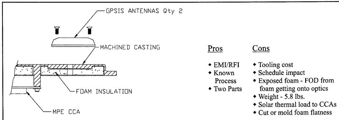
Figure E.4 - Design Option 1
