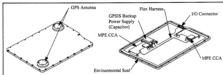
Figure E.2 - GPSIS Cover Assembly
