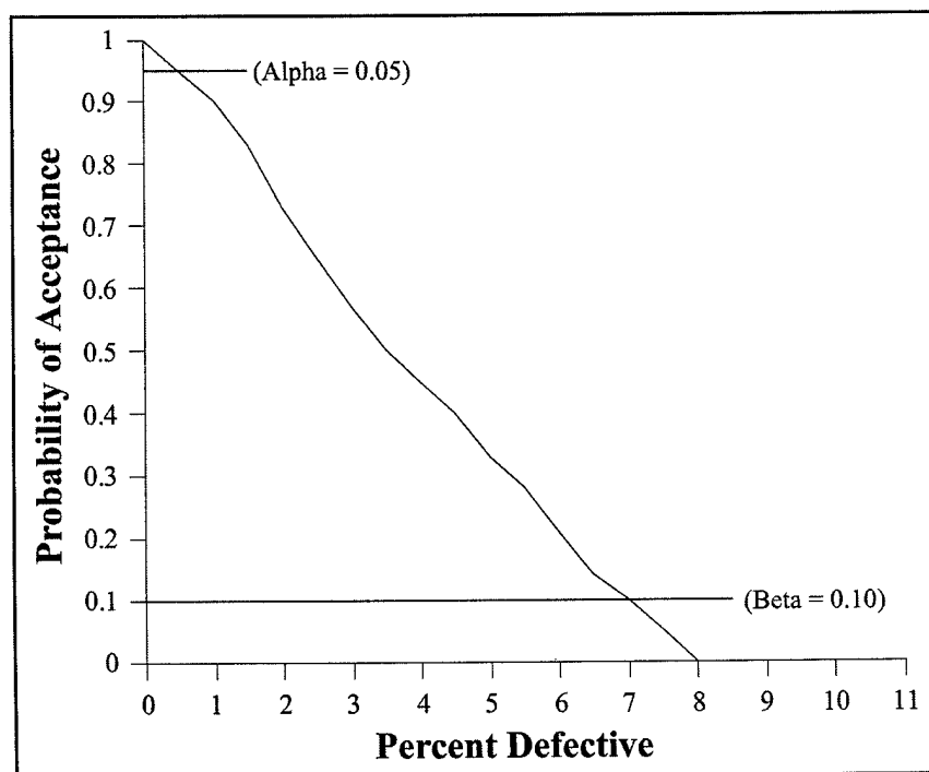
Figure F.10 - Sample OC Curve
