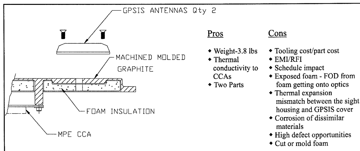
Figure E.6 - Design Option 3
