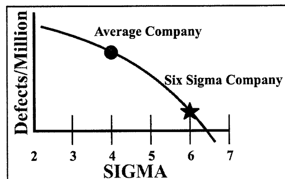
Figure F.7 - Sigma
