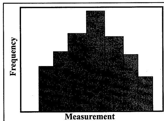
Figure F.8 - Histogram Example
