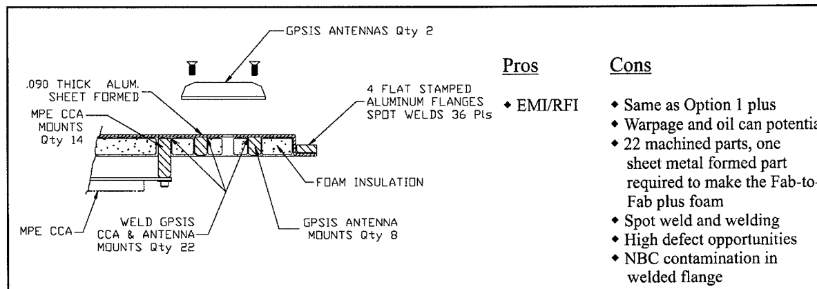
Figure E.5 - Design Option 2
