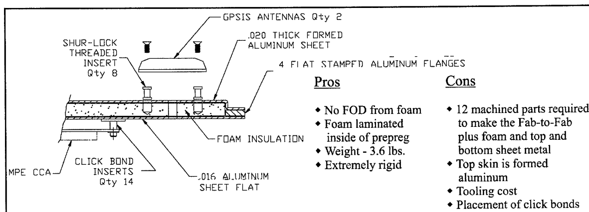
Figure E.8 - Design Option 5
