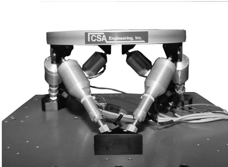
Figure 2.2. Ultra-Quiet Platform.
