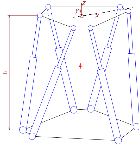
Figure 3.1. Hexapod—3D.
