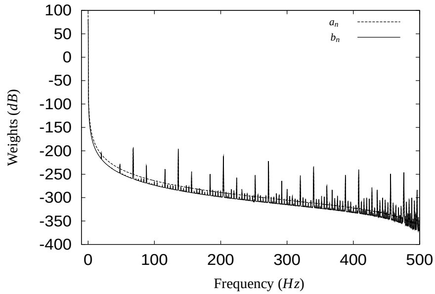
(b) Weights
