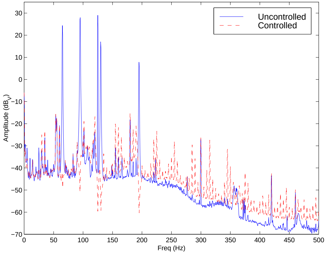
Figure 6.11. Adaptive Disturbance Cancellor on UQP with Five Tones.
