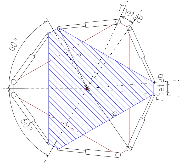
Figure 3.2. Hexapod—Top View.
