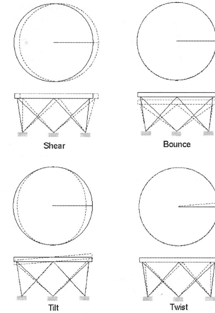
Figure 4.12. Hexapod modes [5].
