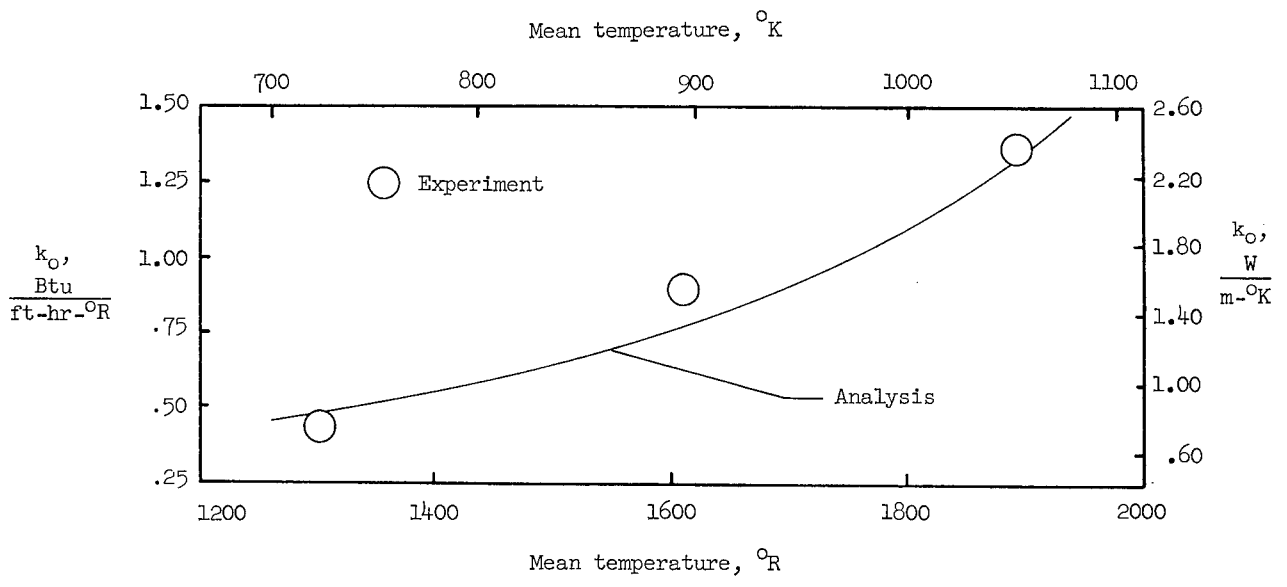
(c) \lambda = 3 .
