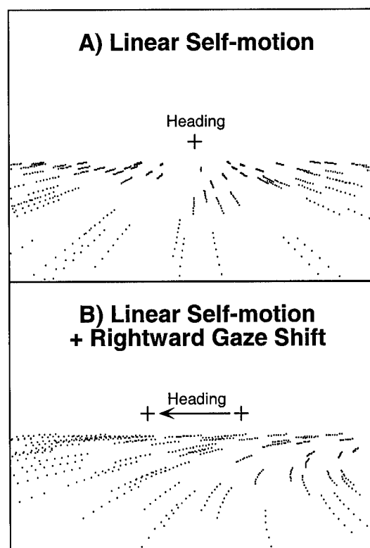
Figure 2.1. Retinal flow fields for two viewing situations. A) Forward translation without a gaze rotation. Observer is fixating in constant direction and heading toward the cross. B) Forward translation while making a gaze rotation. Observer is making a rightward eye movement.
