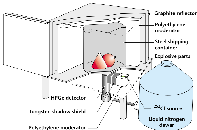
The Portable Isotopic Neutron Spectroscopy (PINS) setup in TA-18 at Los Alamos National Laboratory. The shapes simulate high explosives.
