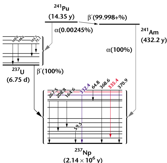
The branching decay of ^{241}\text{Pu} shows the gamma-ray transitions measured by the Pu300 method.
