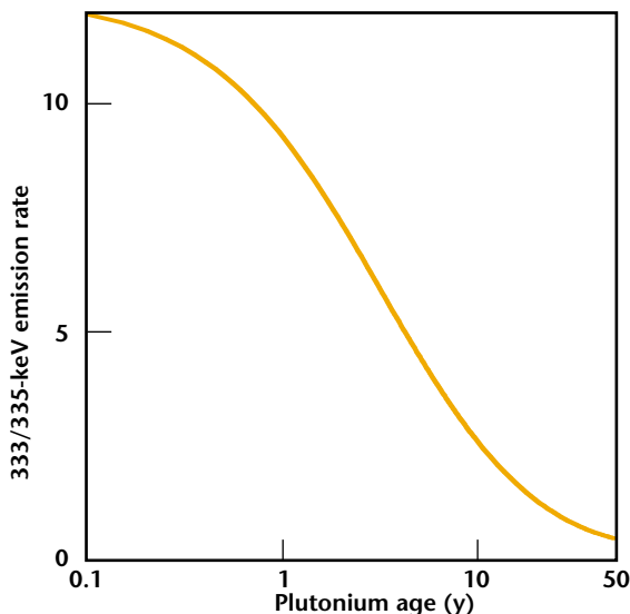
The age of plutonium can be determined by the relative emission rates of the 332.4- and 335.4-keV gamma rays.
