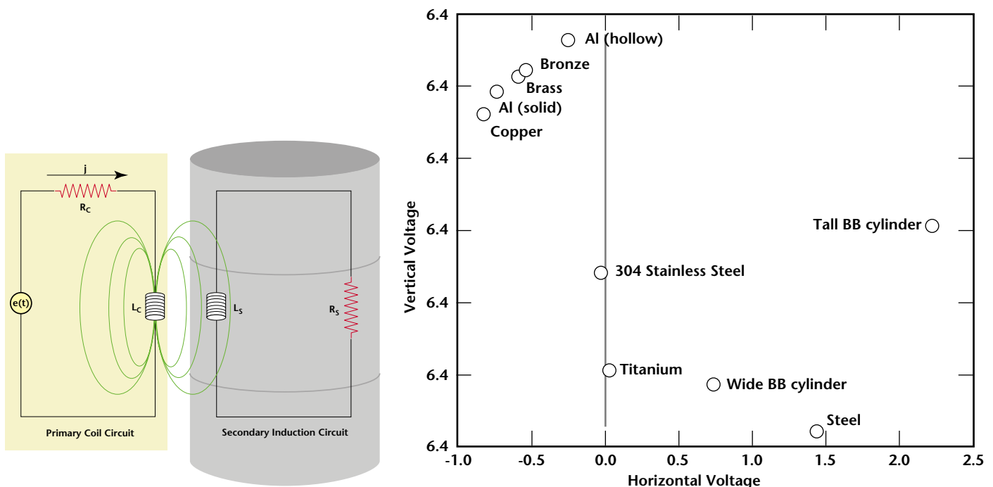
Eddyscope output for different metal objects placed in a steel drum surrounded by a coil.
