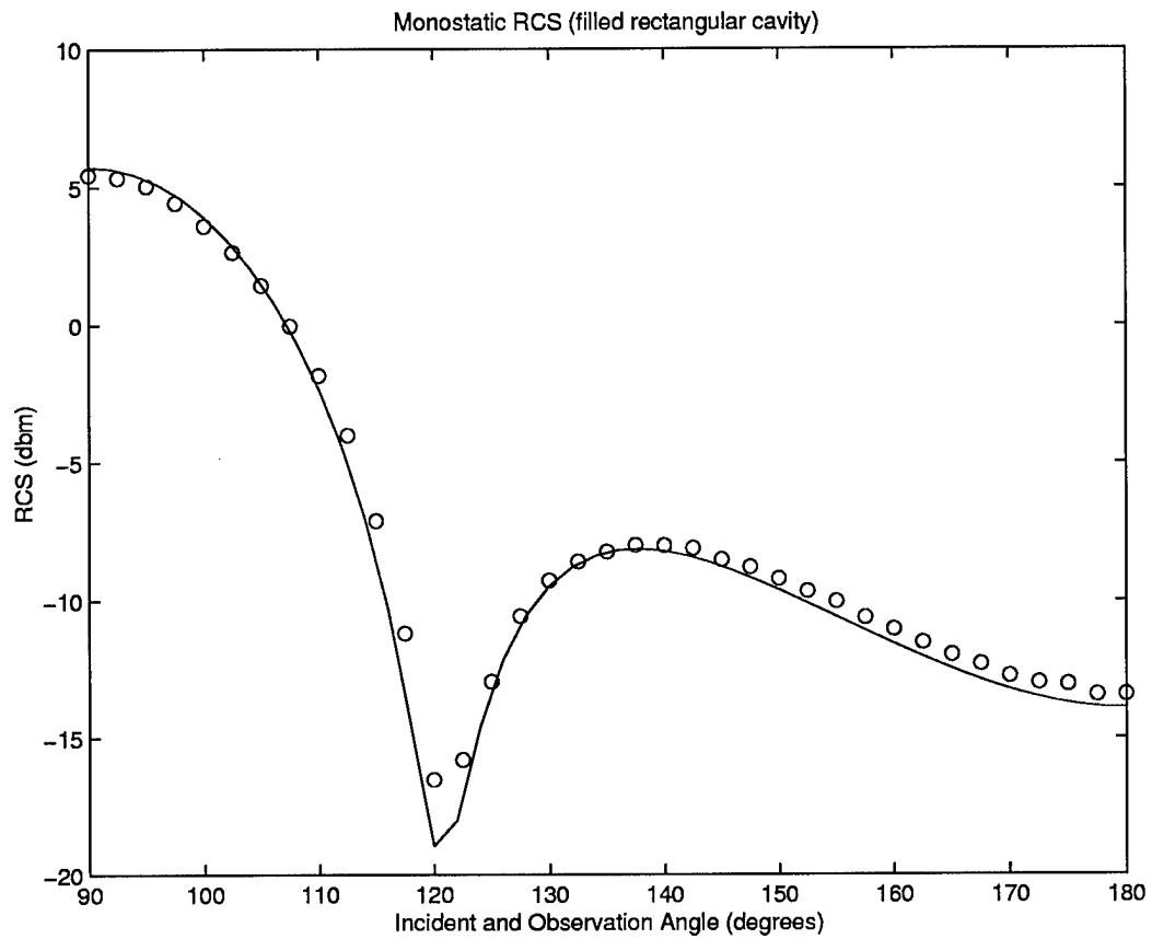
Figure 13 Monostatic RCS signature of a rectangular cavity filled with a lossy dielectric material. Integral equation method ( \circ ) and finite element method ( - )
