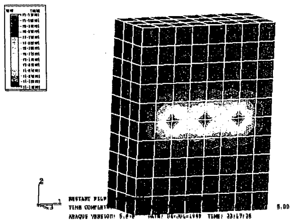
Figure 5-19: Three Dimensional Analysis After Five Days (for comparison) (Scale: maximum 114°F, minimum 55.3°F, interval 4.5°F)
