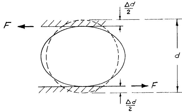
Figure 14. Lateral Compression of Cylinder
