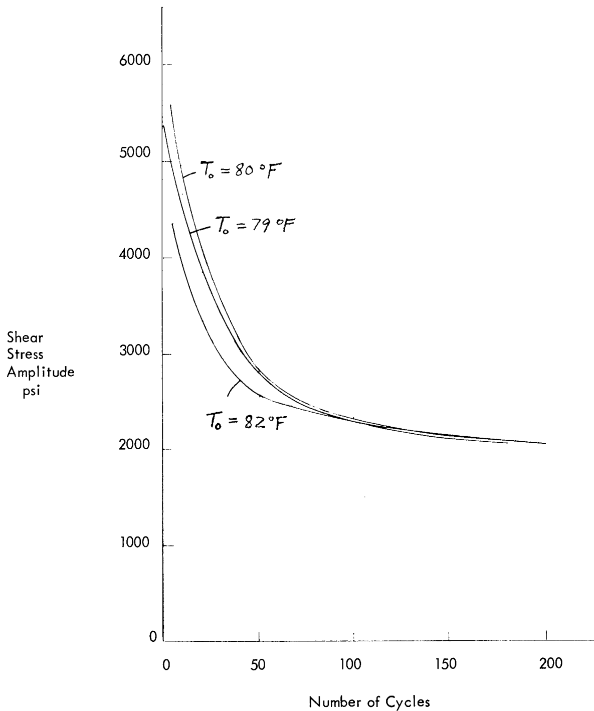
Figure 51. Stress Amplitude vs Number of Cycles for Nylon 66 at 15% Strain Range and 100 cps
