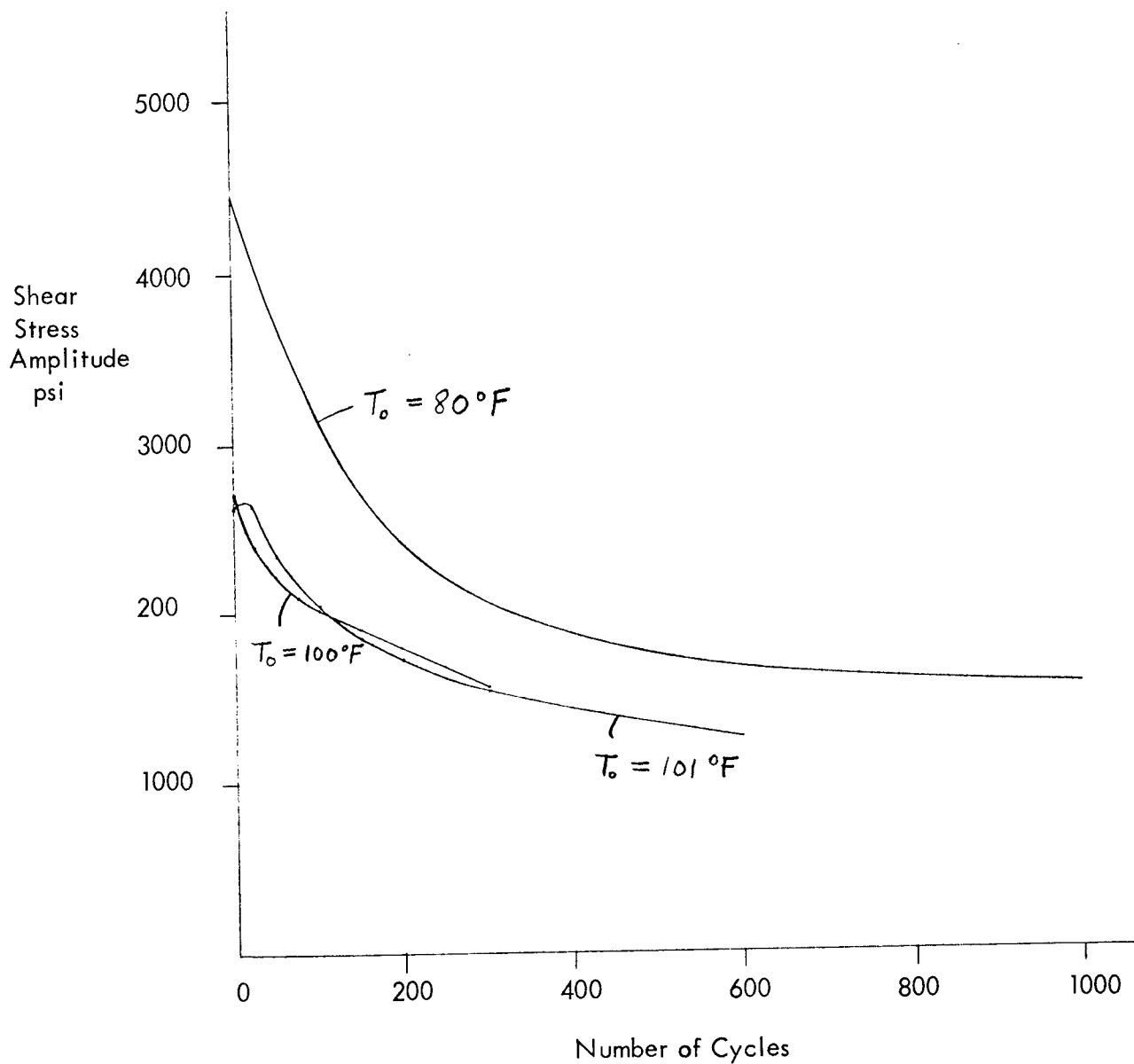
Figure 49. Stress Amplitude vs Number of Cycles for Nylon 66 at 8% Strain Range and 100 cps
