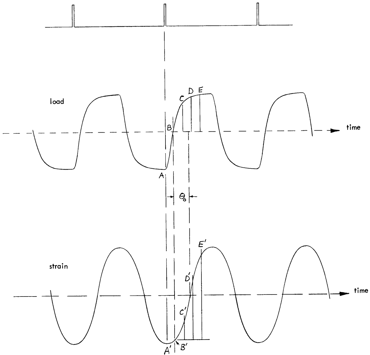
Figure 31. Load-Time and Strain-Time Curves
