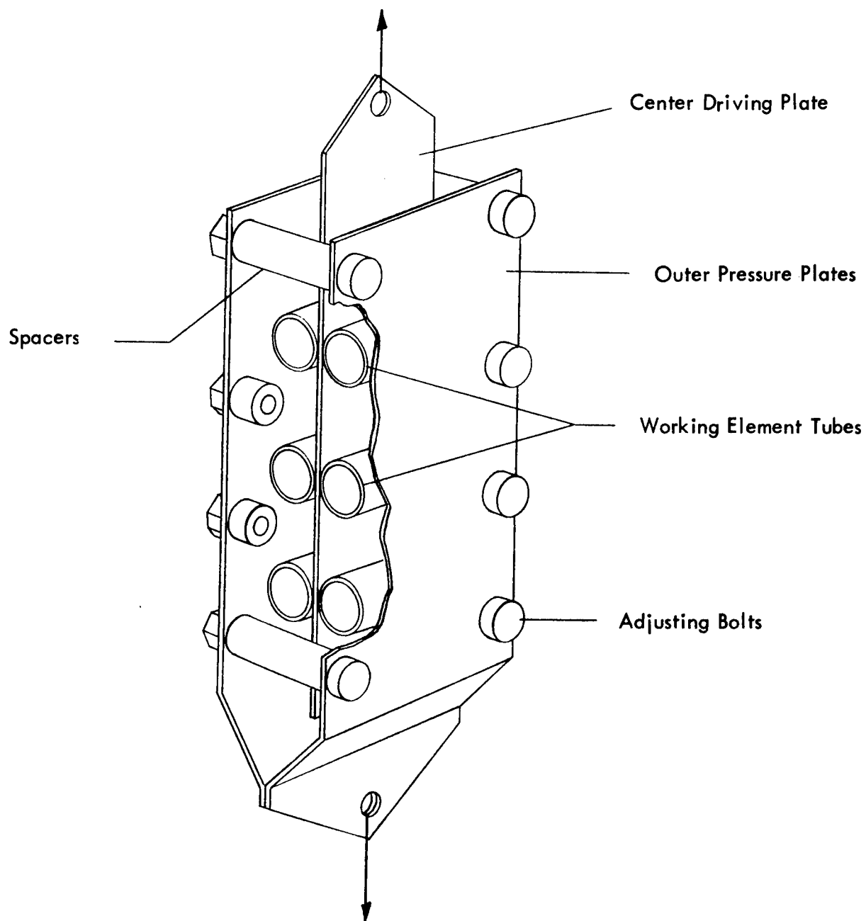
Figure 67. Laboratory Rolling Tube Device
