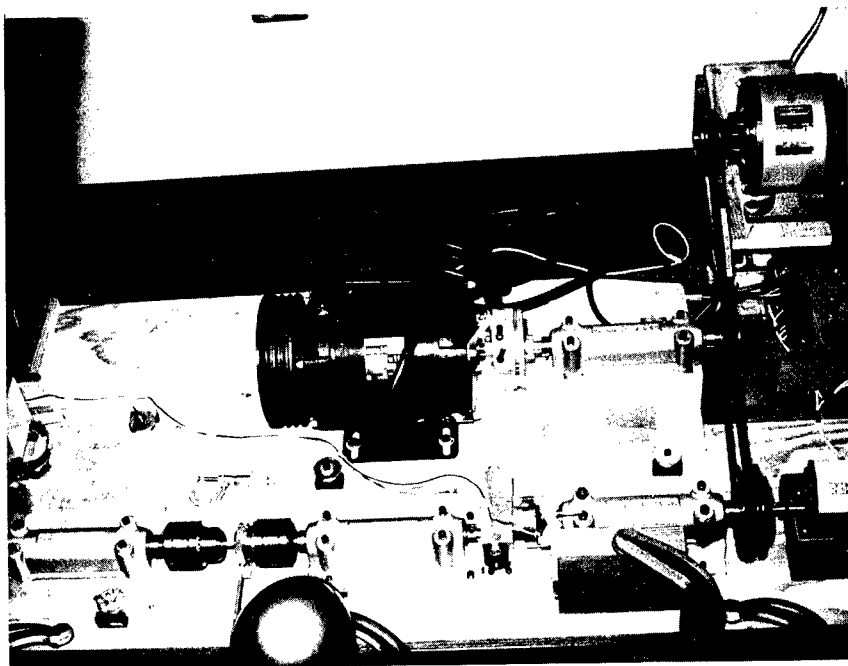
Figure 24 Cyclic Torsion Apparatus I - General Assembly
