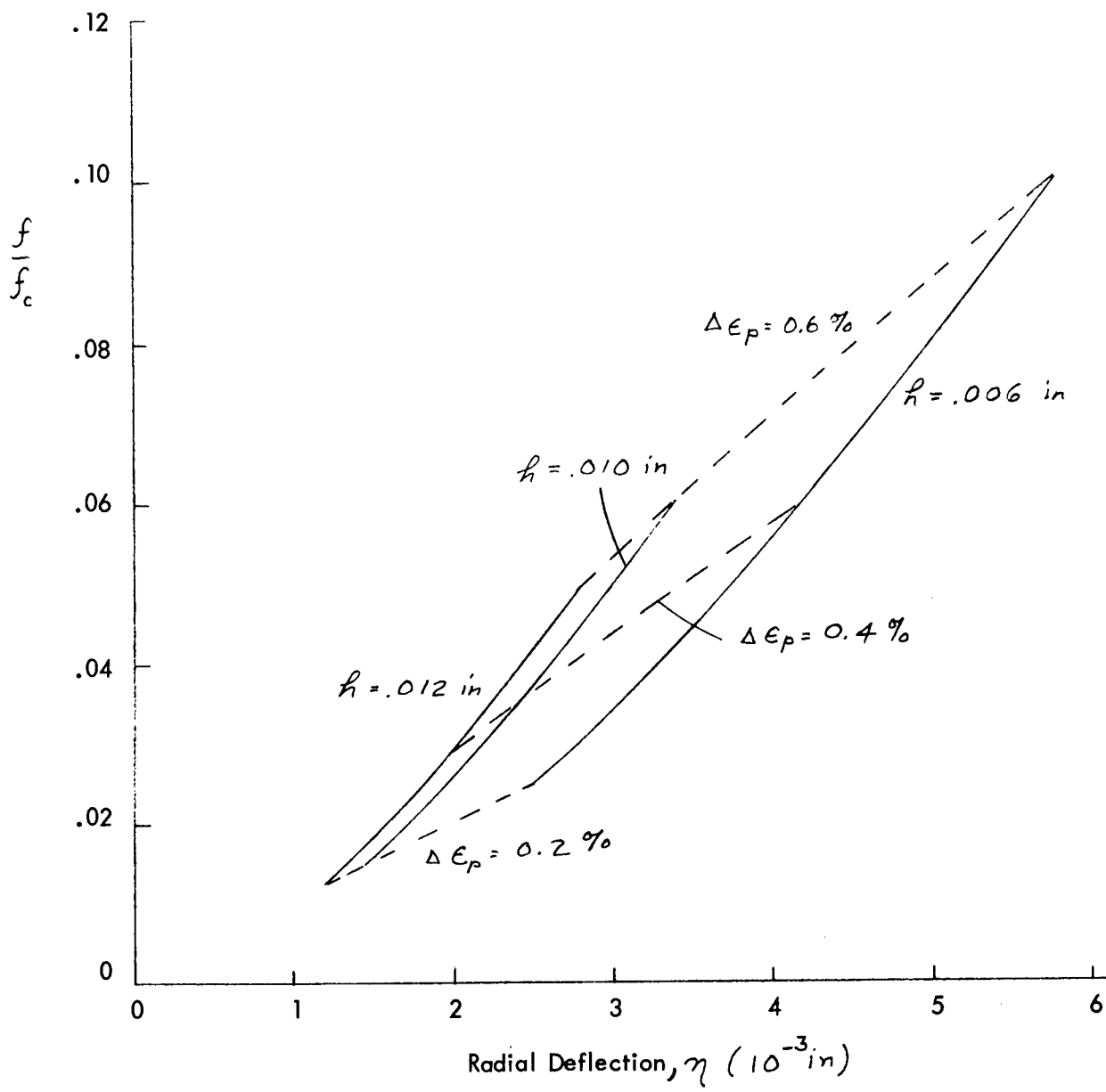
Figure 70. Driving Force - Compressive Force Ratio vs Lateral Deflection for 0.25 inch OD 302 stainless Steel Tube
