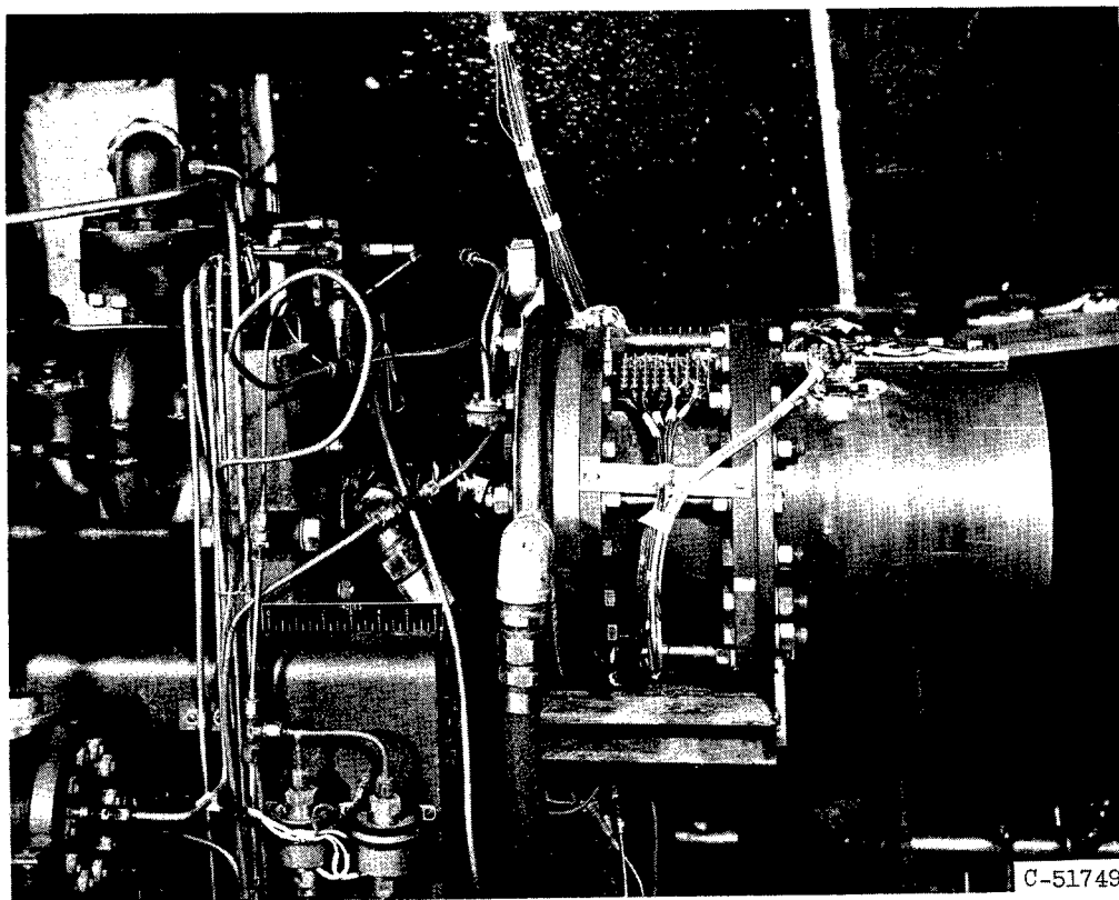
Figure 5. - Engine configuration for chamber heat-transfer tests.
