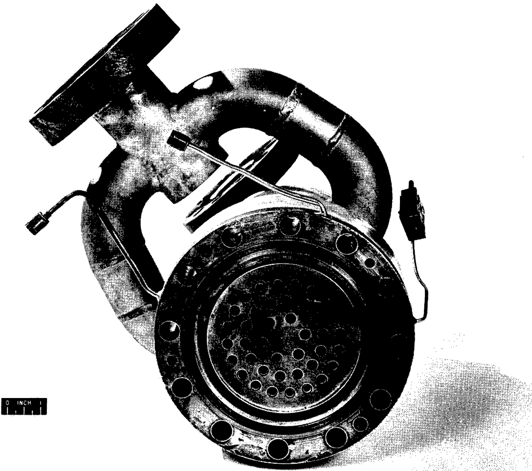
Figure 1. - Propellant injector.
