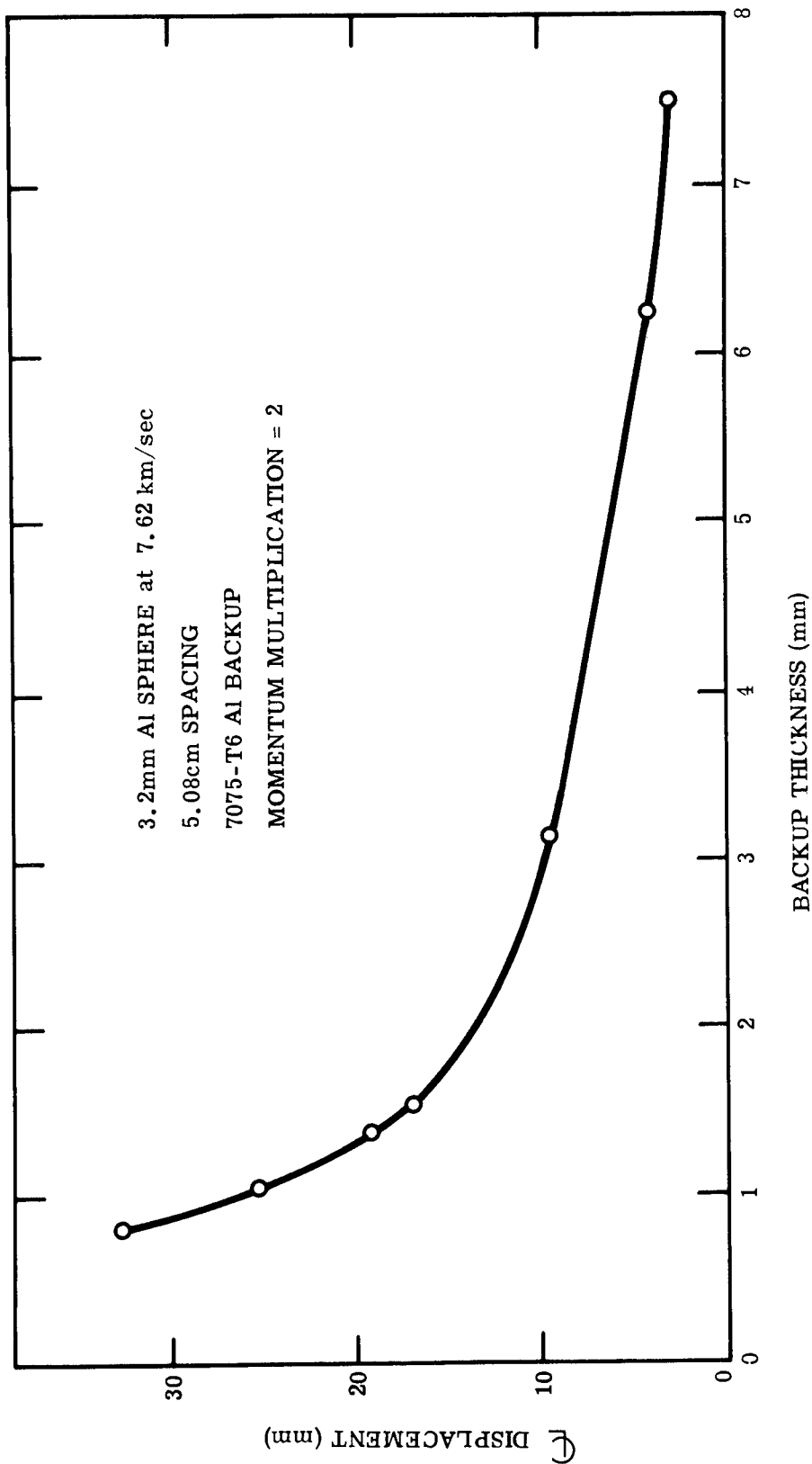
Fig. 16a Centerline Displacement vs Backup Thickness at 200 Microseconds for 3.2-mm Aluminum Sphere
