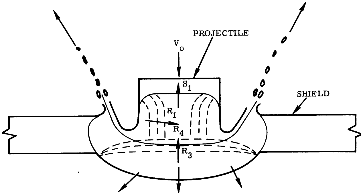
Fig. 1a Wave Pattern in Projectile and Shield Soon After Impact
