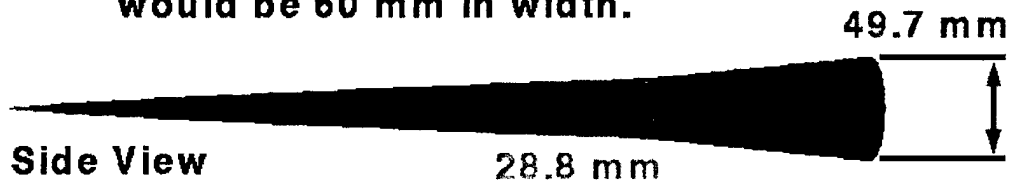
Figure 2. H3P78 Projectile.
