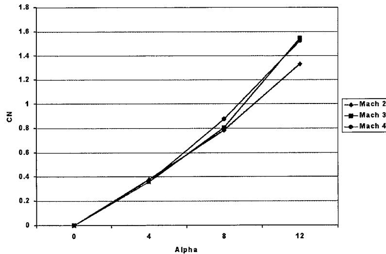
Figure 13. Normal Force Versus Angle of Attack.
