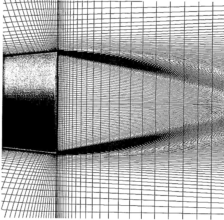
Figure 4. Expanded View of the Grid in the Base Region, Jet Off.
