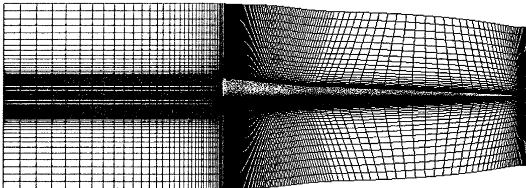
Figure 6. Full Grid for Viscous Computations, Jet On.
