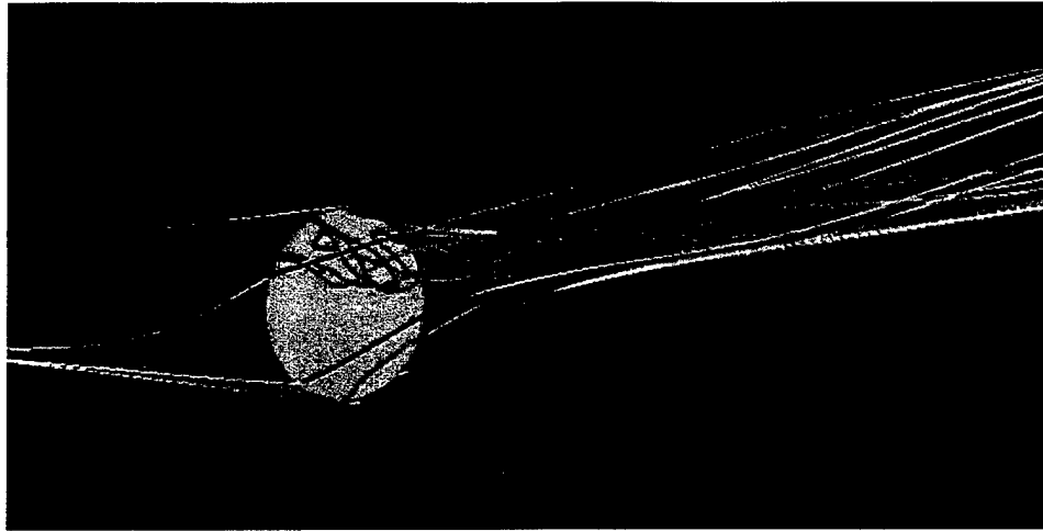
Figure 18. Computed Particle Traces, M = 4.0 , \alpha = 12 .
