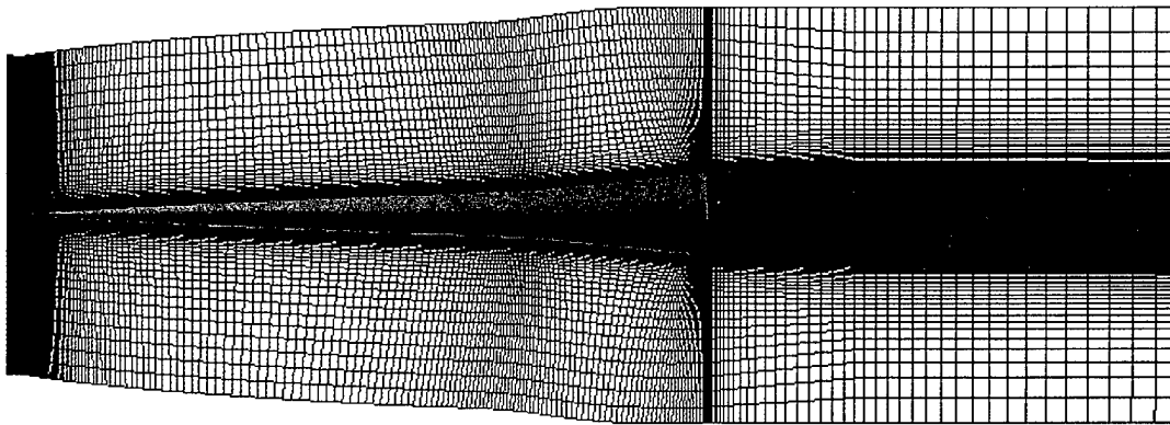
Figure 3. Full Grid for Viscous Computations, Jet Off.
