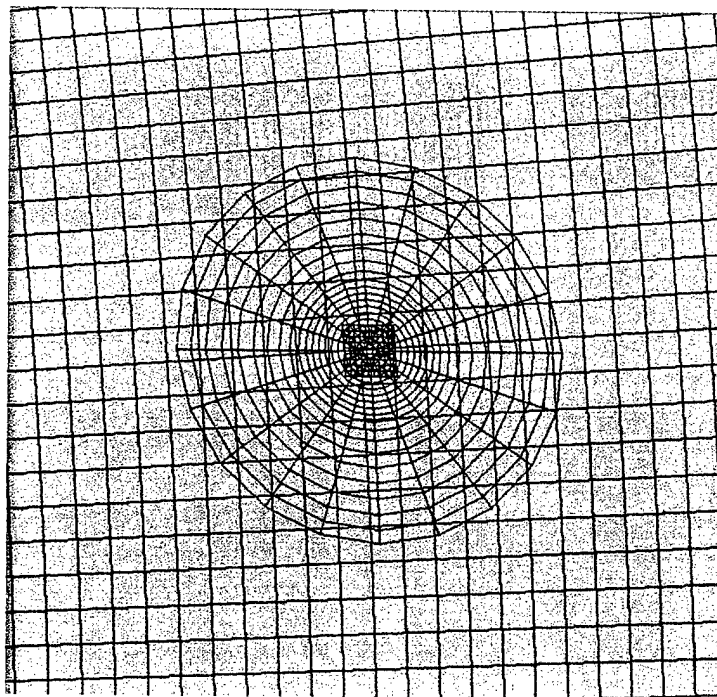
Figure 8. Expanded View of the Jet Grids Projected Onto the Projectile Surface.
