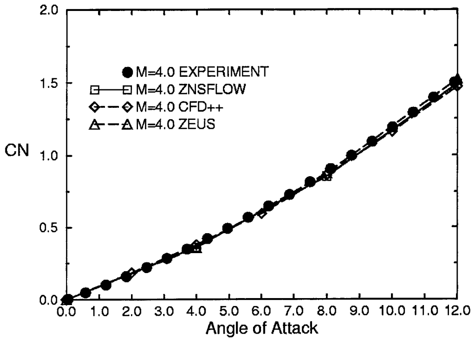
Figure 22. Normal Force Coefficient, M = 4.0.
