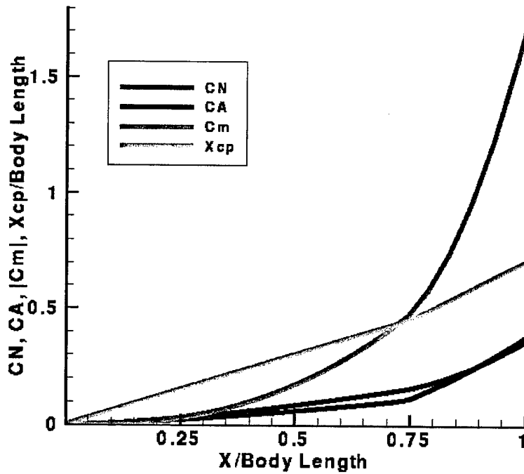
Figure 15. Force/Moment Versus Body Length.
