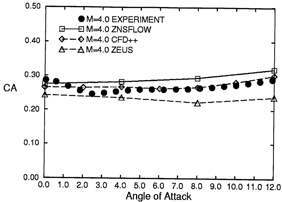
Figure 24. Axial Force Coefficient, M = 4.0 .
