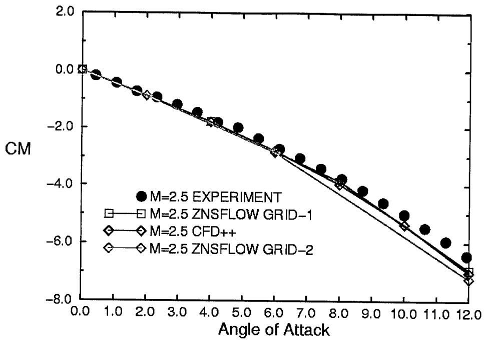
Figure 20. Pitching Moment Coefficient, M= 2.5.
