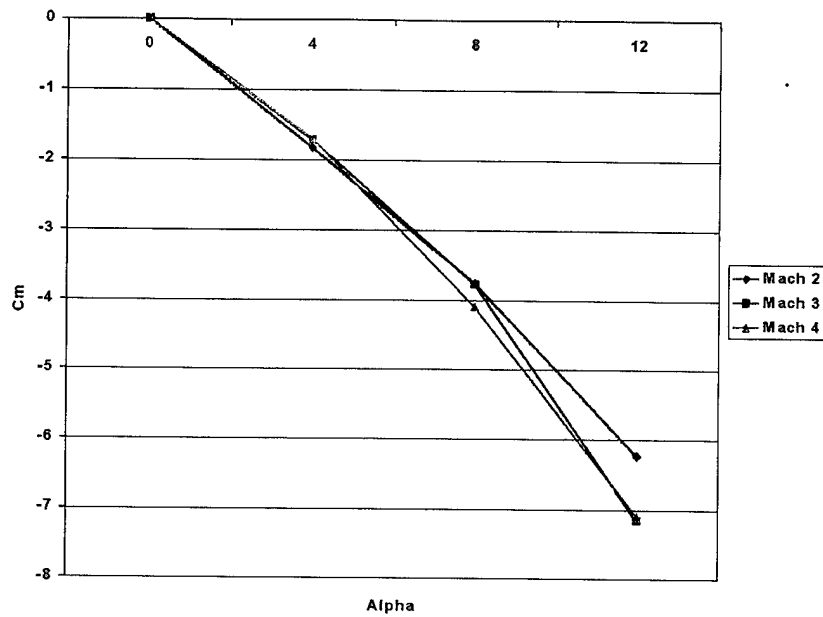
Figure 14. Pitching Moment Versus Angle of Attack.
