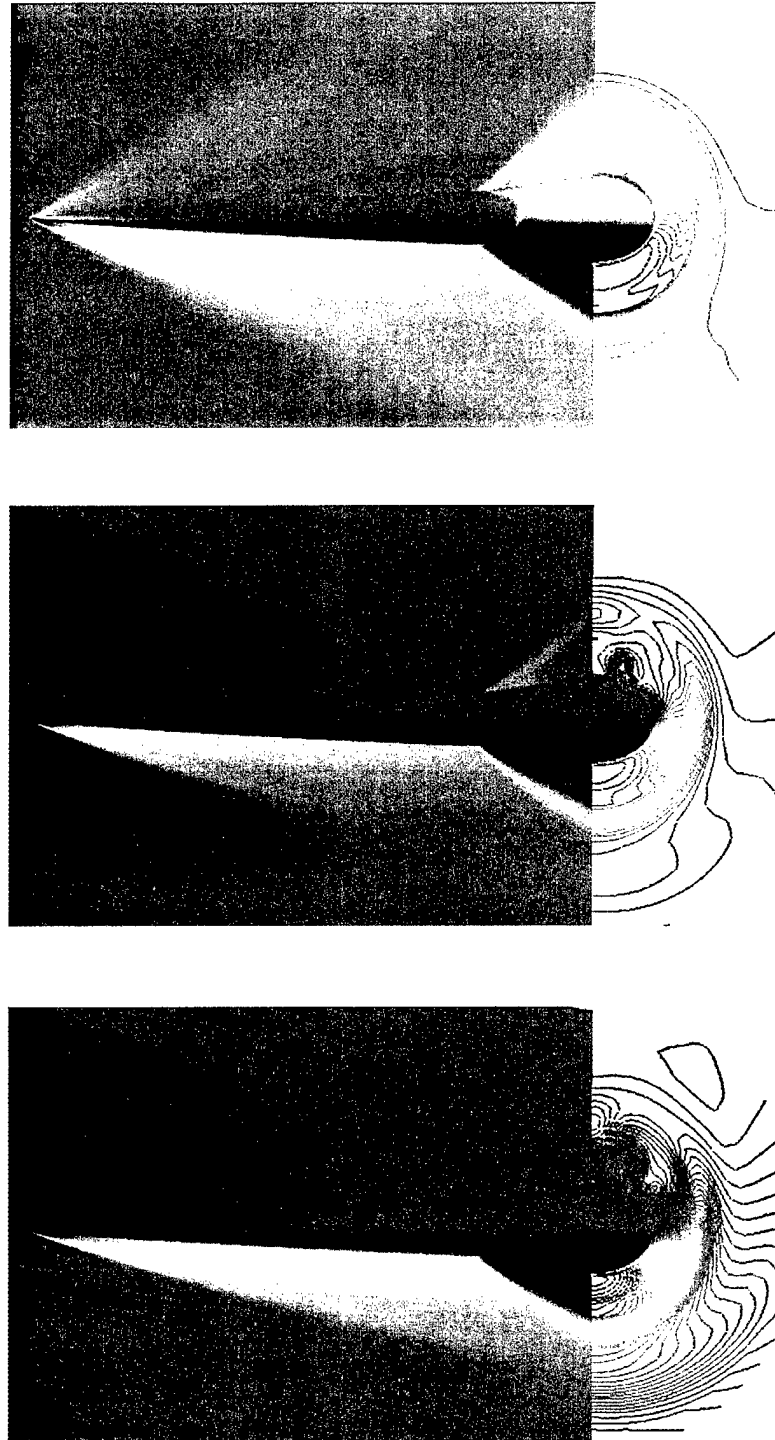
Figure 16. Computed Pressure Contours, M = 2.5 , \alpha = 4^\circ, 8^\circ, 12^\circ (top to bottom).
