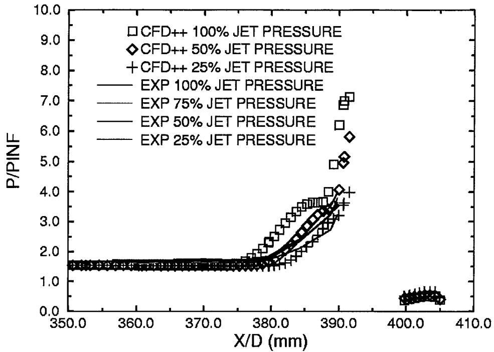
Figure 31. Surface Pressure Contours Comparison Along the Centerline of Symmetry, M = 4.0 , \alpha = 0^\circ .
