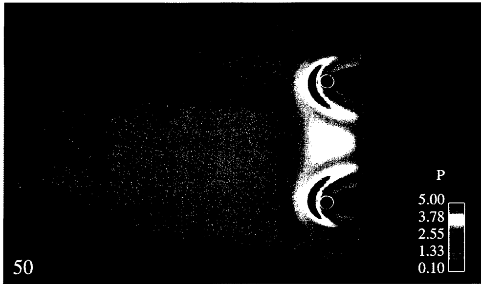
Figure 29. Computed Surface Pressure Contours Near the Jet, 50% Jet Pressure, M = 4.0 , \alpha = 0^\circ .
