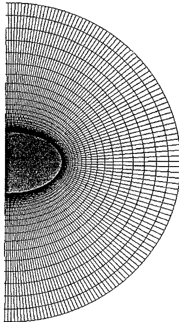
Figure 5. Circumferential Cross Section of the Grid at the Base.
