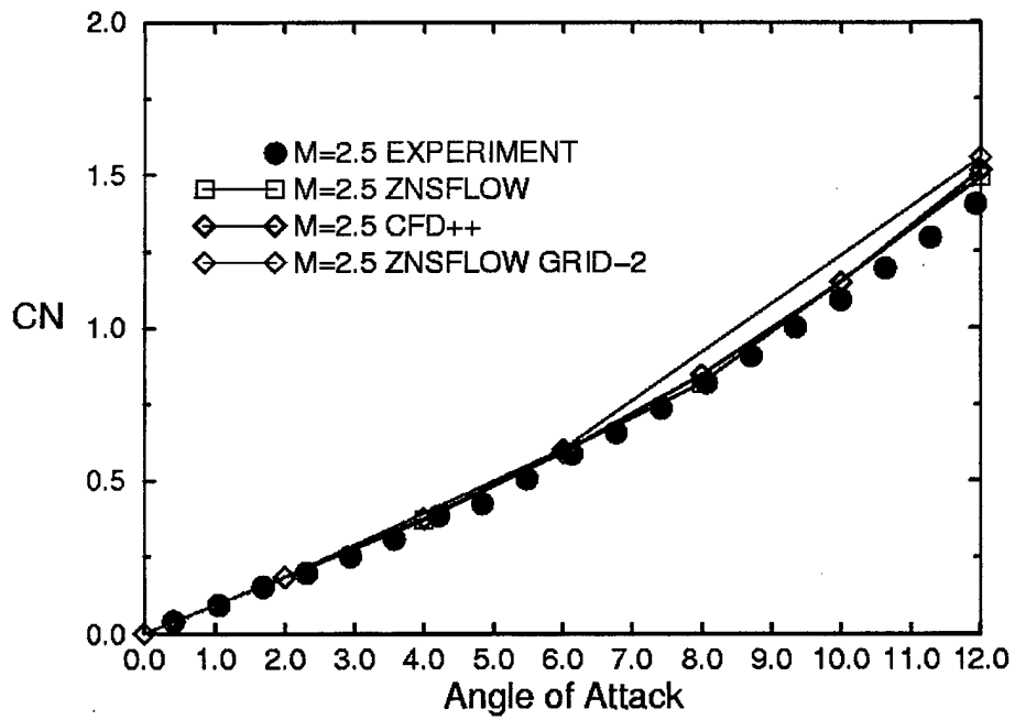
Figure 19. Normal Force Coefficient, M = 2.5 .
