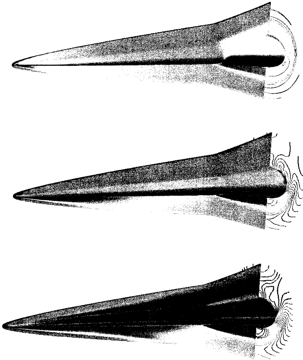
Figure 17. Computed Pressure Contours, M=4.0 , \alpha = 4^\circ, 8^\circ, 12^\circ (top to bottom).
