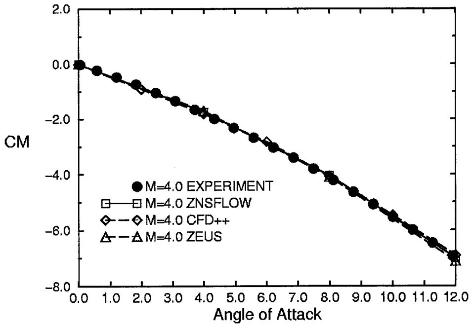
Figure 23. Pitching Moment Coefficient, M = 4.0.
