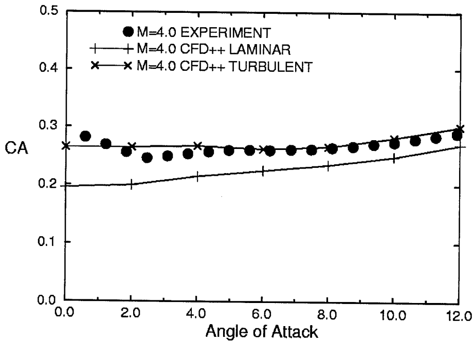
Figure 25. Effects of Turbulence on Axial Force Coefficient, M = 4.0 .
