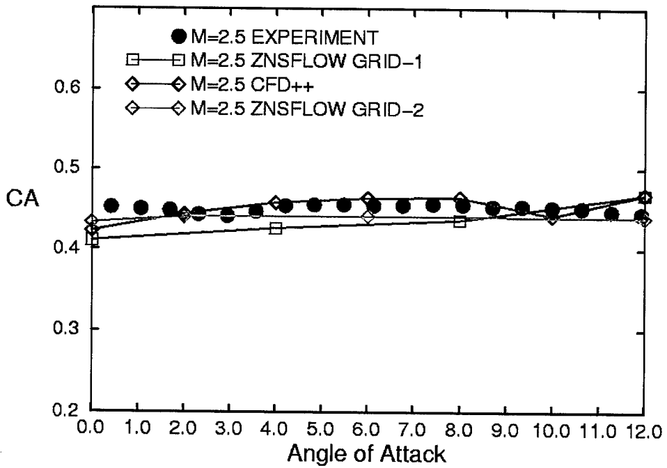
Figure 21. Axial Force Coefficient, M = 2.5.
