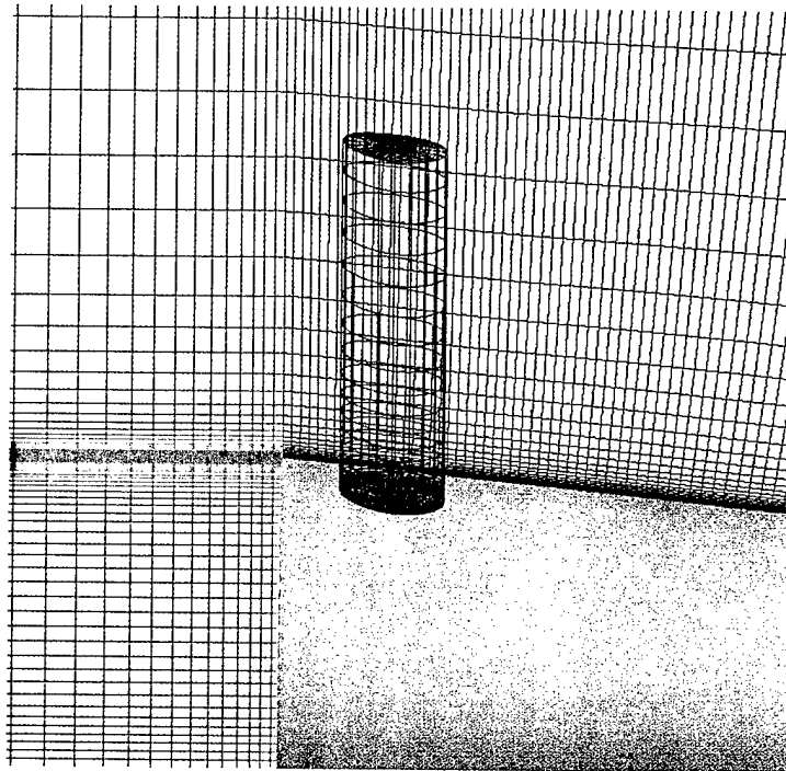
Figure 7. Expanded View of the Grid in the Base Region, Jet On.
