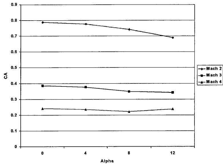
Figure 12. Axial Force Versus Angle of Attack.
