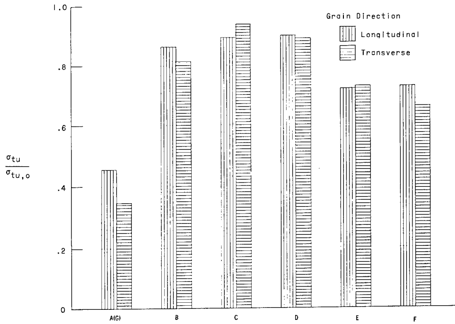
(a) Ultimate strength.
