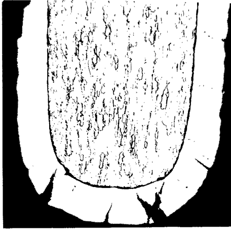
(c) Tumbled edge. L-63-4796
