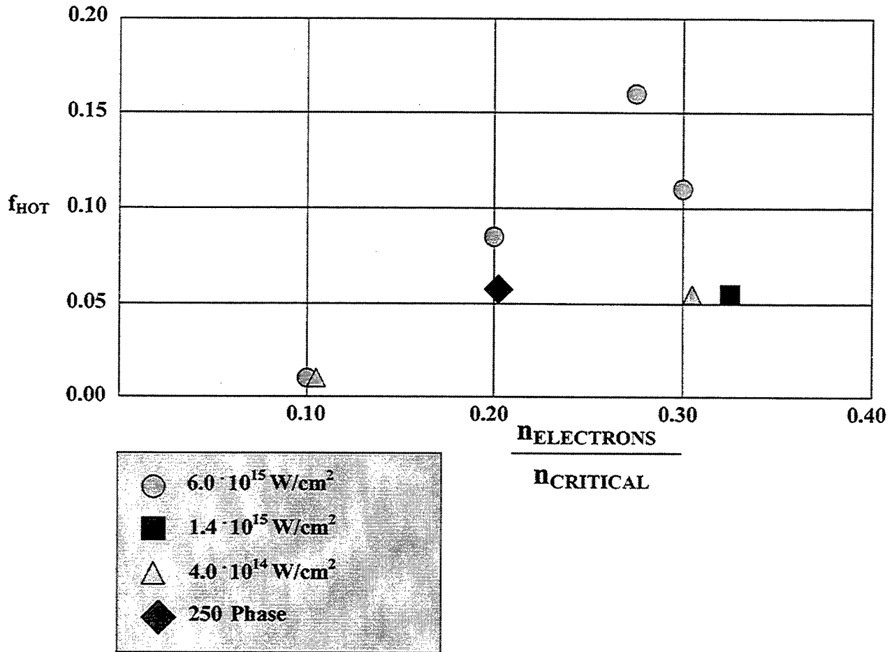
Figure 17. Hot Electron Fraction, f_{HOT} , versus Density. Helen Laser Experiment, Atomic Weapons Establishment, England [Reference 5].
