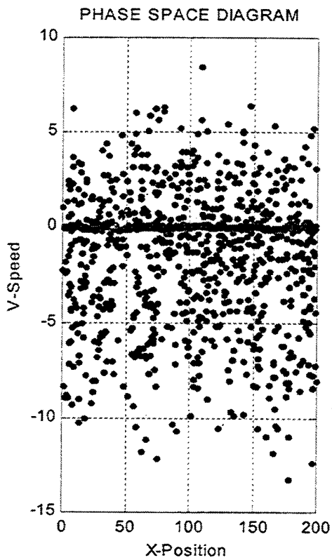
Figures 6a and 6b. Phase Space and Velocity Distributions at times 50 and 100
