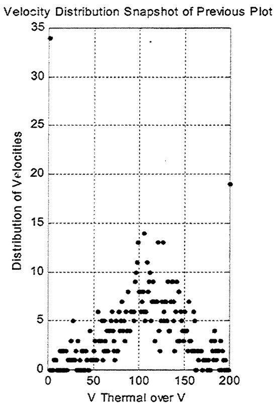
Figures 6g and 6h. Phase Space and Velocity Distributions at times 350 and 400
