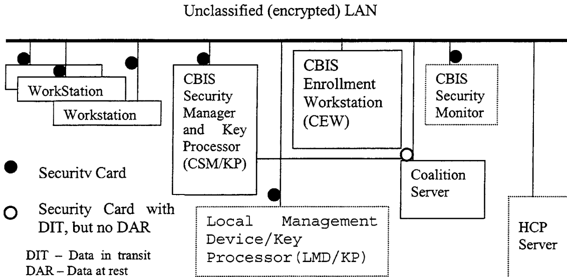
Figure 5.1. CBIS LAN Segment from Ref. [15]
