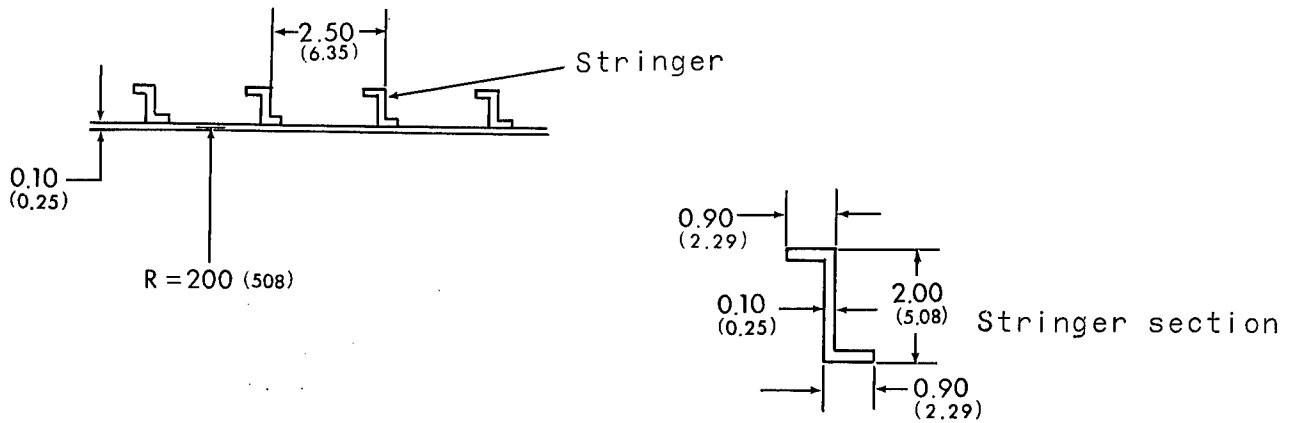
(b) Ring-and-stringer-stiffened cylinders; a = 200 in. (508 cm). (See fig. 2(a) for ring section.)
