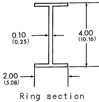
(a) Ring-stiffened corrugated cylinders; a = 200 in. (508 cm).
