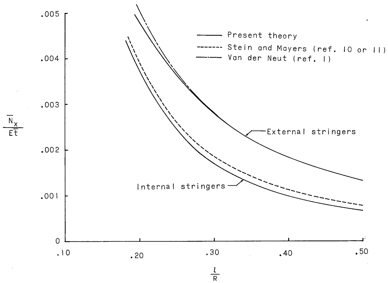
Figure 5.- Panel instability predictions for compressed longitudinally stiffened cylinders.
