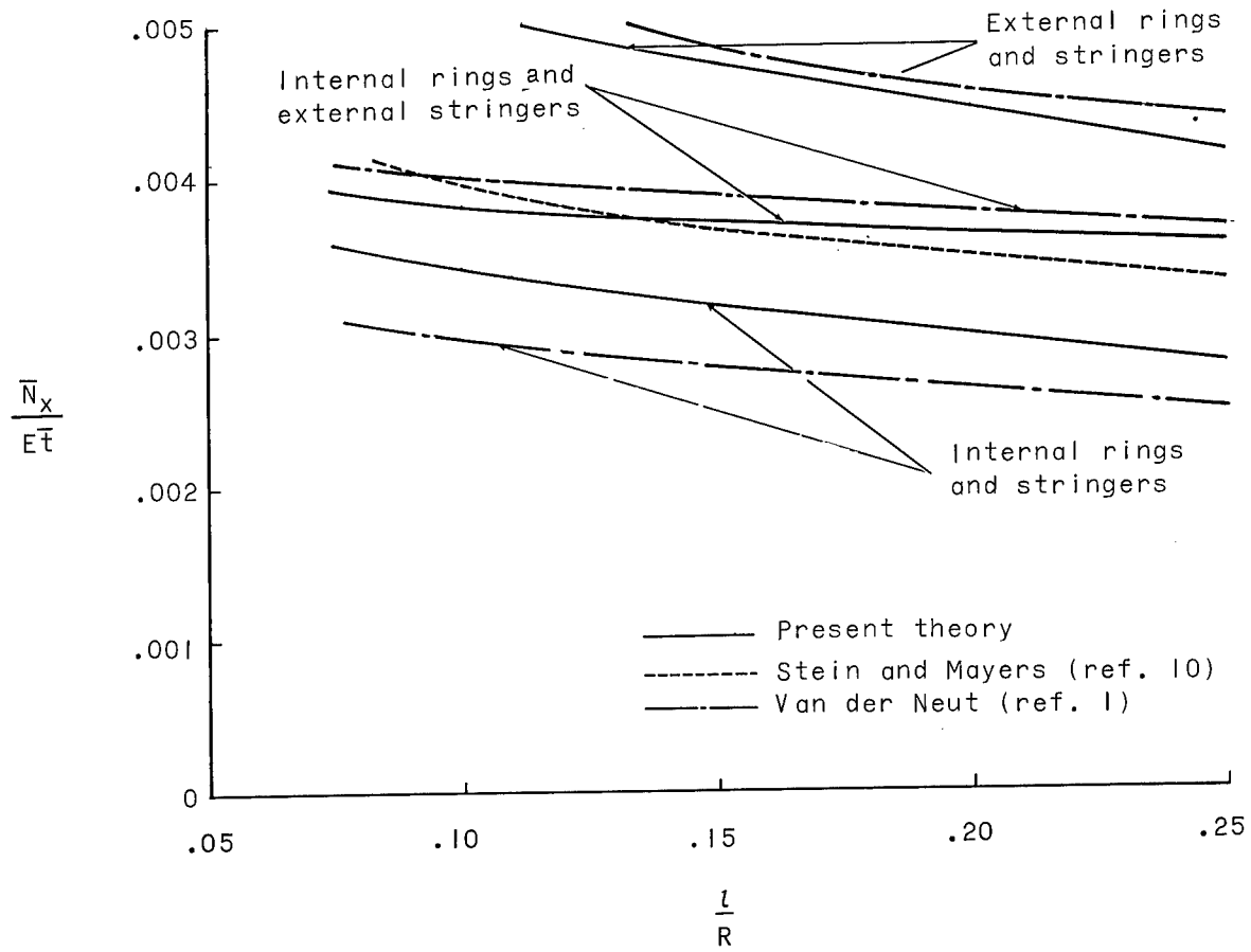
Figure 4.- General instability predictions for compressed ring-and-stringer-stiffened cylinders.
