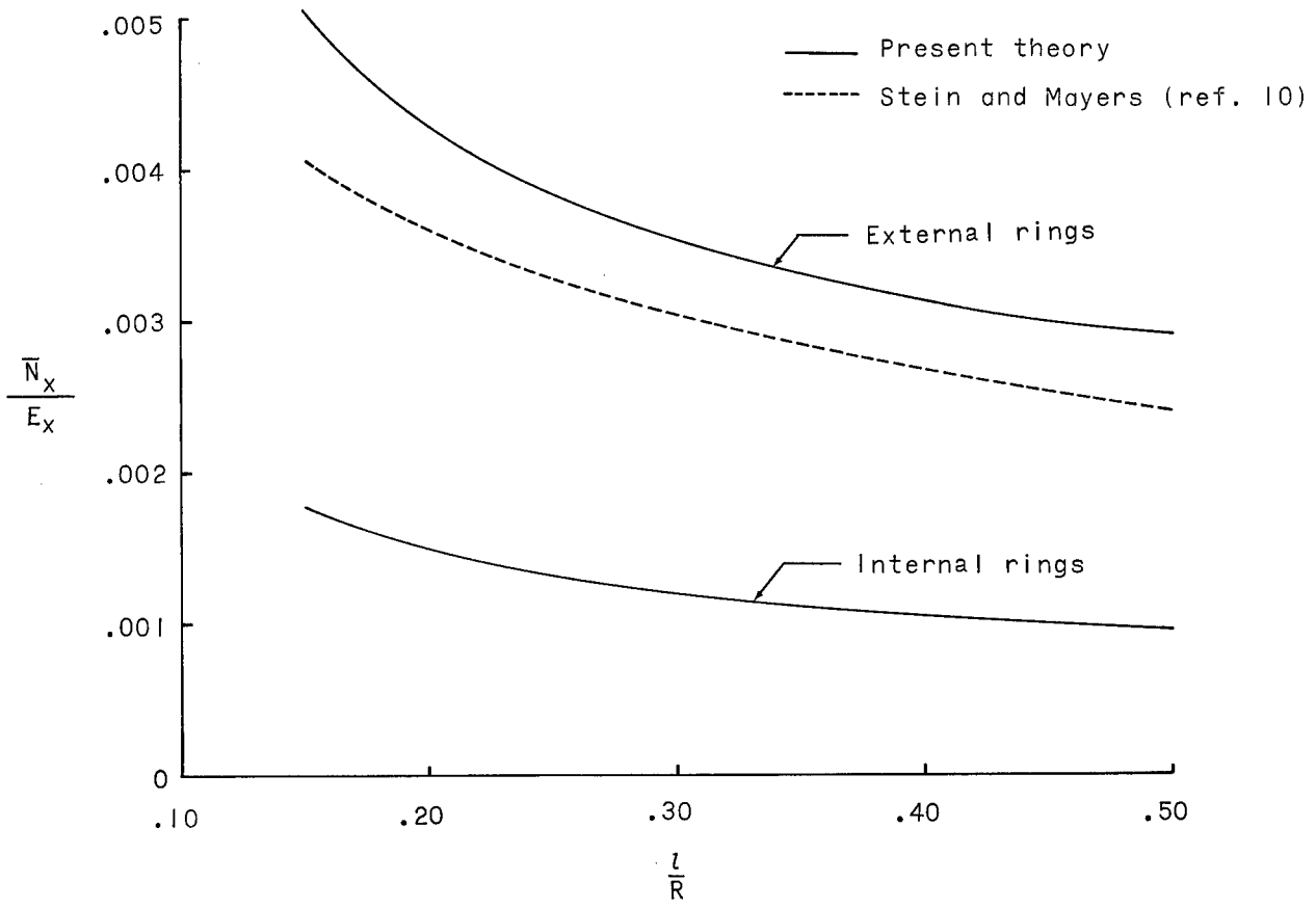
Figure 3.- General instability predictions for compressed ring-stiffened corrugated cylinders.
