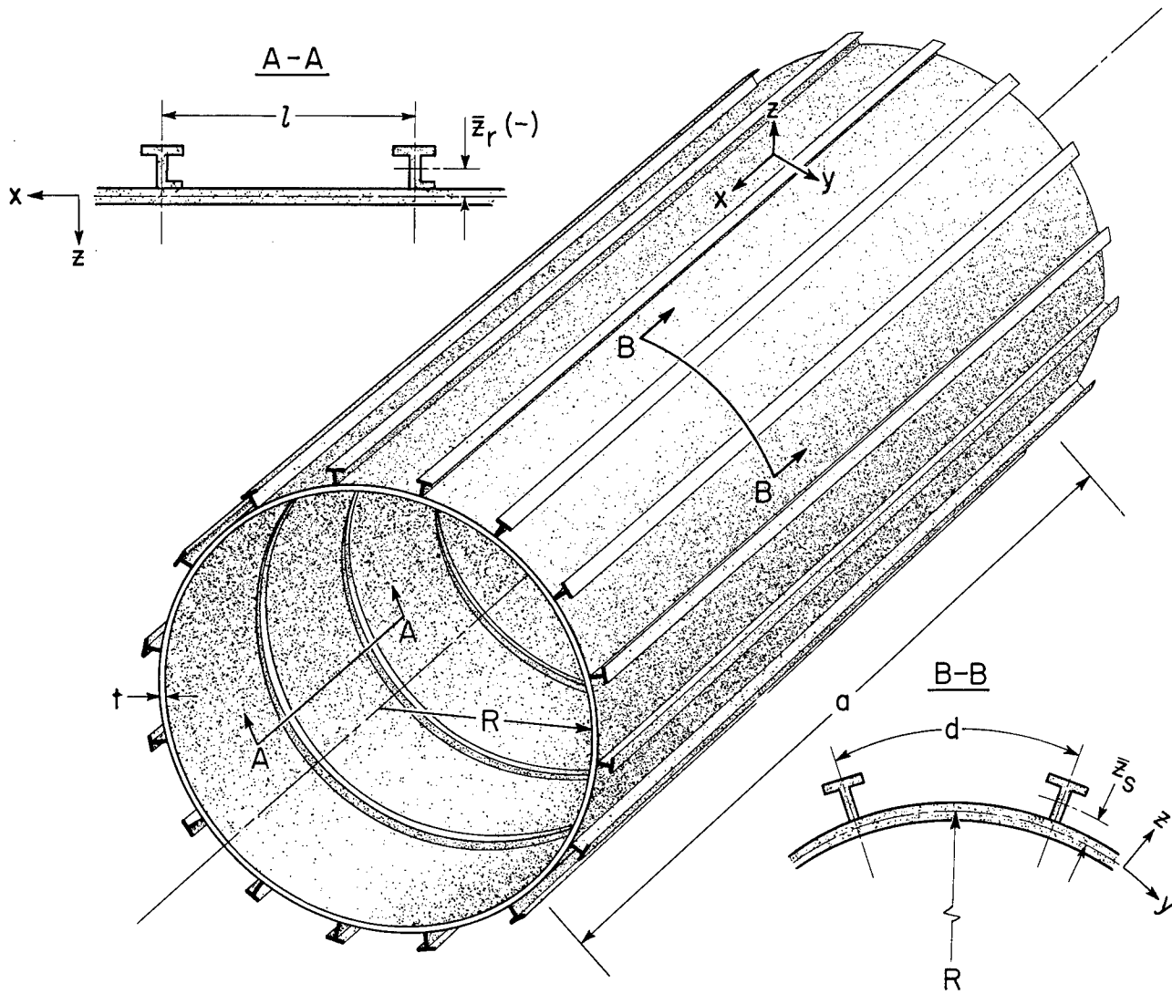
Figure 1.- Geometry of stiffened cylinder.
