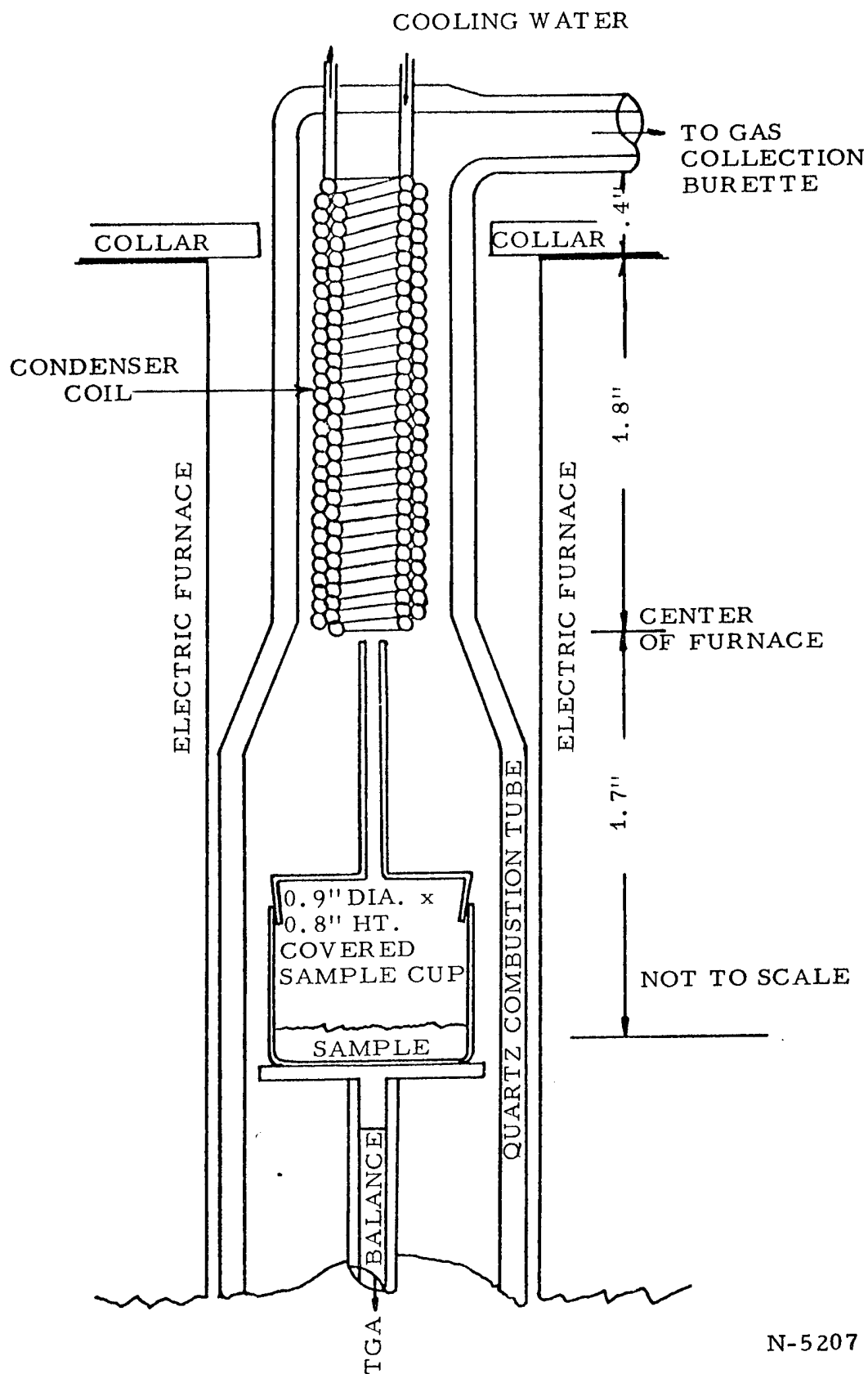
Figure 6. Gas Evolution System of TGA-GE Apparatus
