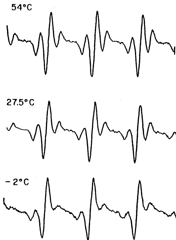
Figure 39. ESR of Hexamethylbenzene in \text{H}_2\text{SO}_4 at 3 Temperatures
