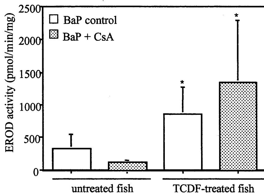
Figure 3. Ethoxyresorufin-O-deethylase activity in liver microsomes of previously untreated fish and those treated with 10 pmol TCDF/g fish weight. Untreated and TCDF-treated fish where further exposed to 28 \mu\text{g} ^3\text{H} -BaP/g fish weight \pm 10 \mu\text{g} /g cyclosporin A. Values are reported as pmol/min/mg EROD activity \pm standard deviation. * indicates significant difference from previously untreated fish exposed to BaP control ( p \leq 0.05 ).
