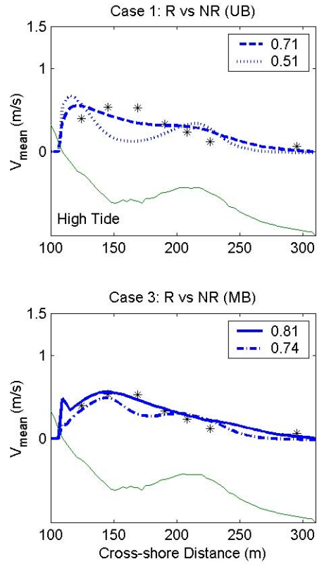
Figure 4.16. Measured and model computed cross-shore variation of the alongshore current for the high tide (0400) at Delilah on Oct.15. The solid line represents roller dissipation (R) with measured bathymetry (MB), dashed line R with uniform bathymetry (UB), dash-dot line no roller (NR) with MB and dotted line NR with UB. Numbers in right corner represent model skill values. Instrument bathymetry transect provided as a reference
