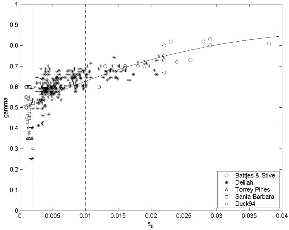
Figure 4.1. Optimized values of \gamma versus deepwater wave steepness, s_0 , for data from Battjes & Stive (1985), Delilah, Torrey Pines, Santa Barbara and Duck94. Solid curve is Equation 18. Dashed-dot line indicates extent of Battjes & Stive data sets. Dashed line indicates s_0 values equal to 0.002.
