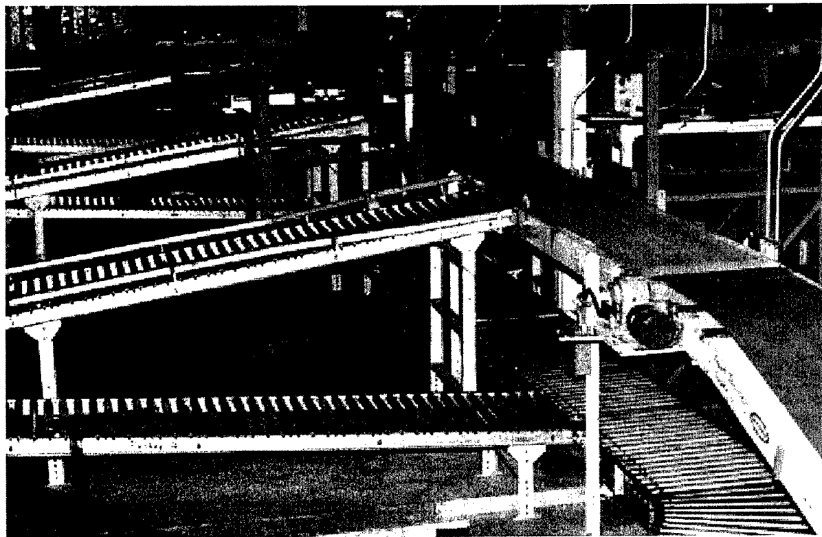
Figure 3-2. Conveyor System
